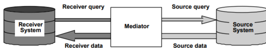
Figure 19: data mediation
