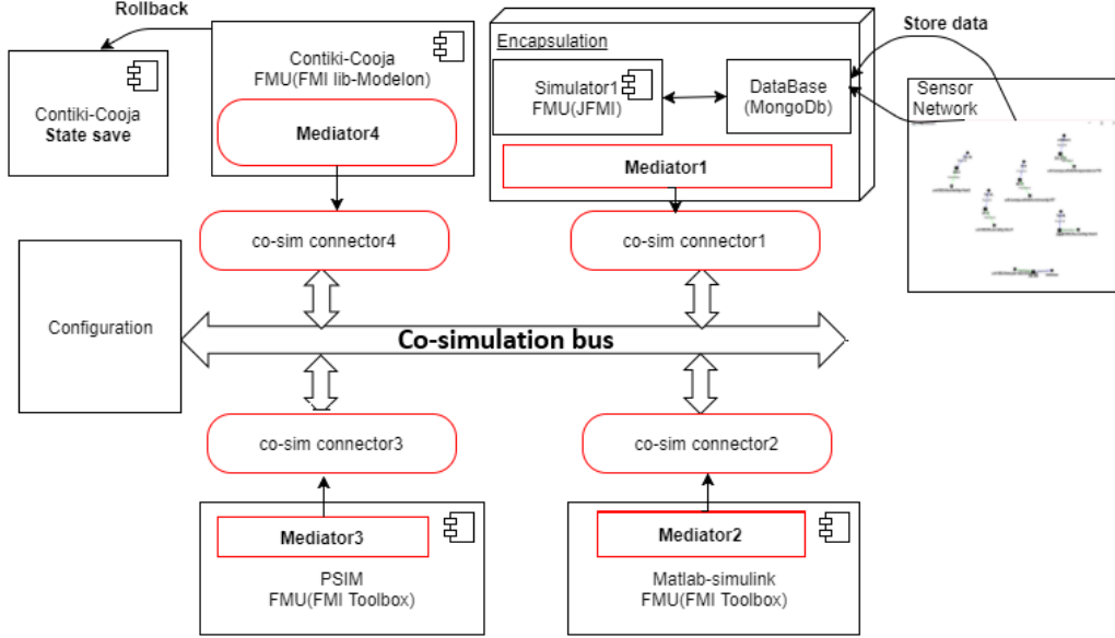
Figure 28: components mediation
