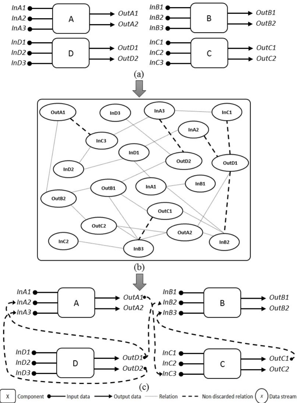
Figure 42: Example of Subsystem-to-Subsystem Graph Model building with DREAM
