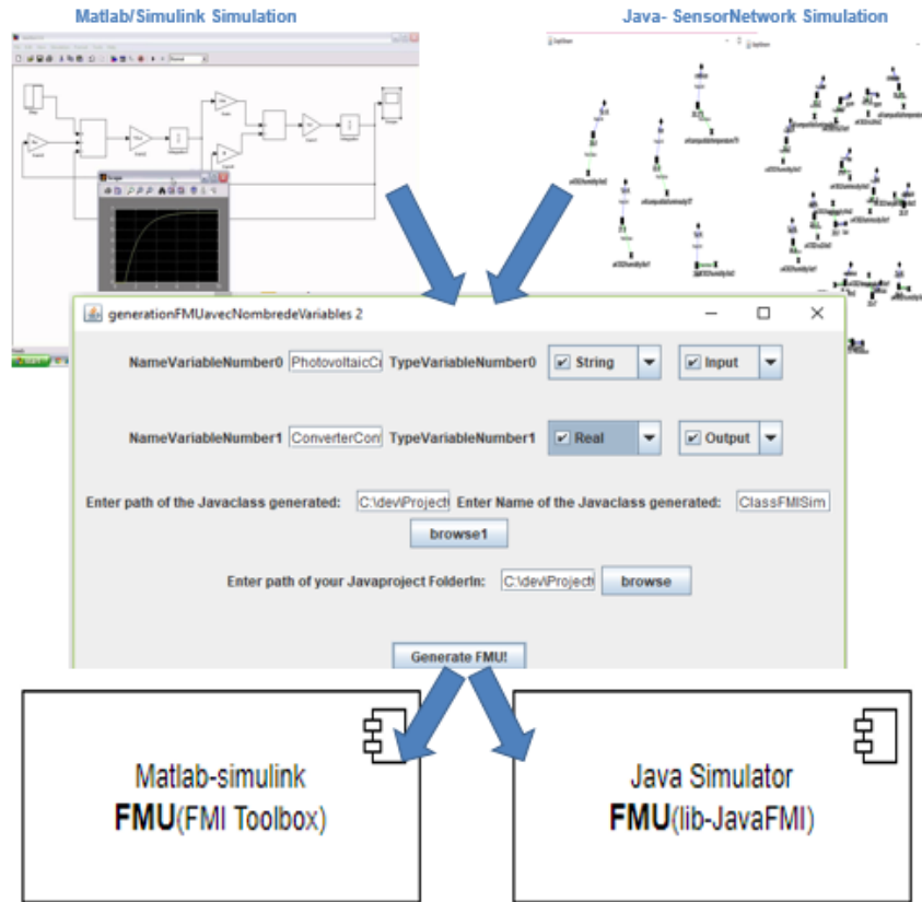
Figure 61: FMI component generation process
