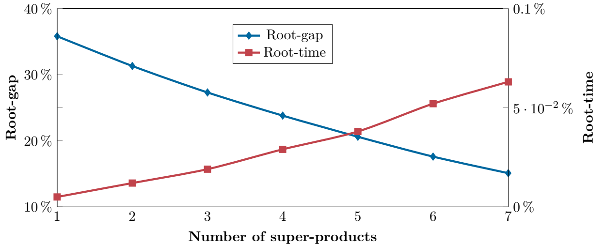
Figure 4.7: K-EMP root-gap and computation time rate
