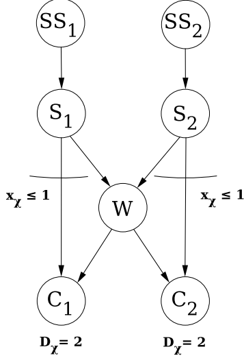
Figure 3.9: Valid inequalities
