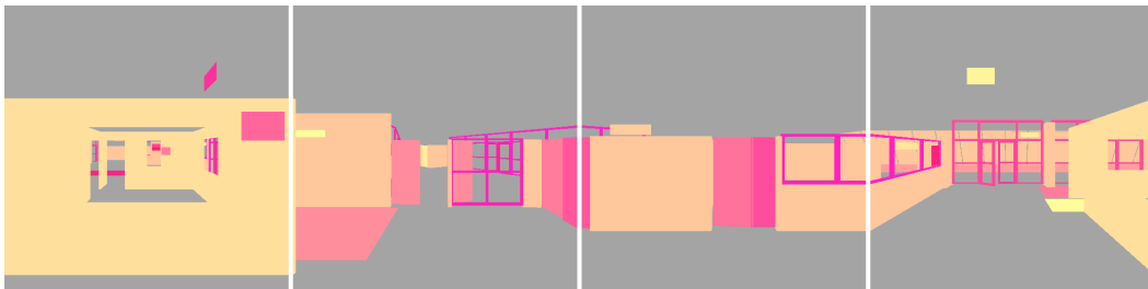
Figure 4.6: A view of how visibility of objects are computed. Each of the four images represent are renderings with a 90^\circ \times 90^\circ virtual camera, pointing in four orthogonal directions, thus creating a 360^\circ \times 90^\circ field of view. Each object of the scene are given a unique color, and pixels of each color are counted to know the size of the object in the field of view. Above a certain number of pixels, the object is considered visible from the point where the camera are placed for the rendering. The place from which these images are taken roughly correspond to the location indicated in figure 4.4, and the left-most image correspond to the perspectives shown in figure 4.5.
