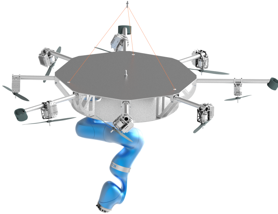
Figure 6.14 – CAD model of the SAM prototype.
