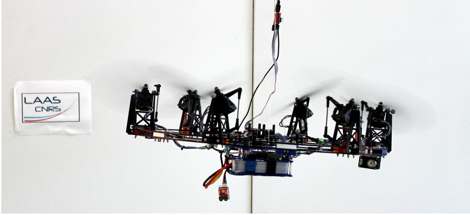
Figure 6.9 – Photo of the real FAST-Hex prototype.
