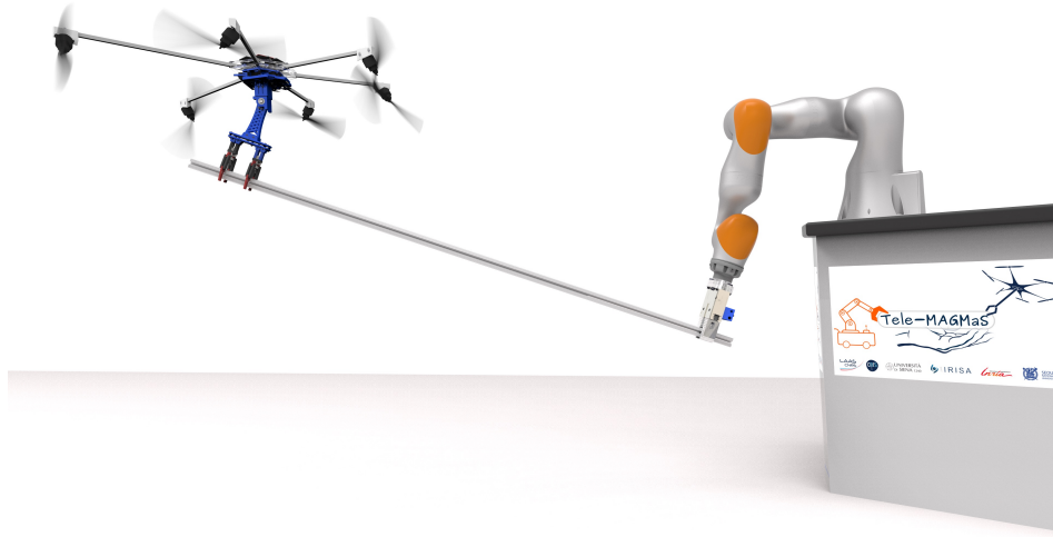
Figure 9.5 – CAD model of the MAGMaS system used for the experimental validation. The ground robot is a KUKA LBR iiwa industrial manipulator, while the aerial robot is the OT-Hex MRAV presented in Sec. 6.1.
