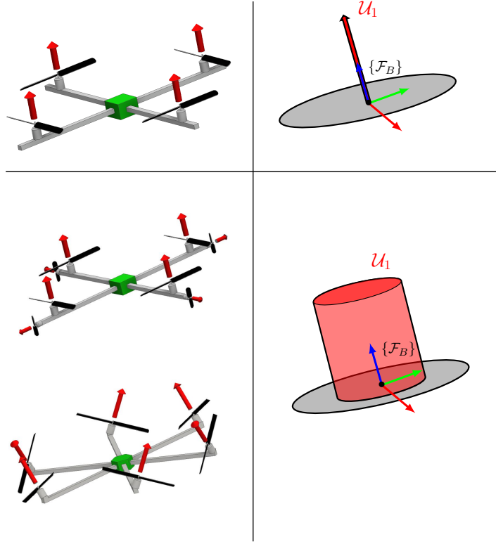
Figure 7.2 – Examples of MDT MRV designs ( left ) and possible Laterally-Bounded input Force (LBF) approximations ( right ). In particular, the set of body forces obtained with a zero net torque are represented.
