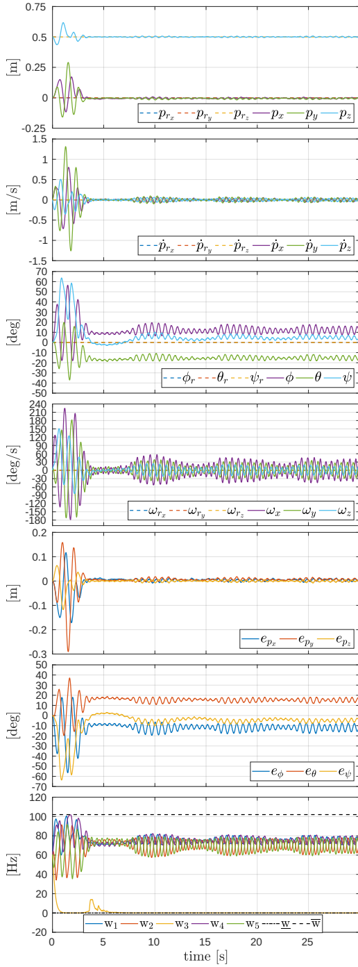
Figure 7.35 – Plots of the Tilt-Hex with rotor failure and \beta = 0 deg while hovering. The robot is disturbed with a constant external torque. From top to bottom : the position, linear velocity, orientation and angular velocity tracking, the position and orientation errors, and the actuator spinning velocities.
