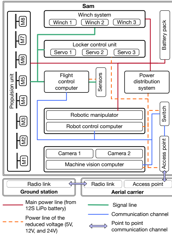
Figure 11.6 – Diagram of the architecture of the SAM ( left ) and photos of the power distribution system ( right ), composed of two power bus-bars ( top ), a power distribution unit ( middle ), and a battery pack ( bottom ).
