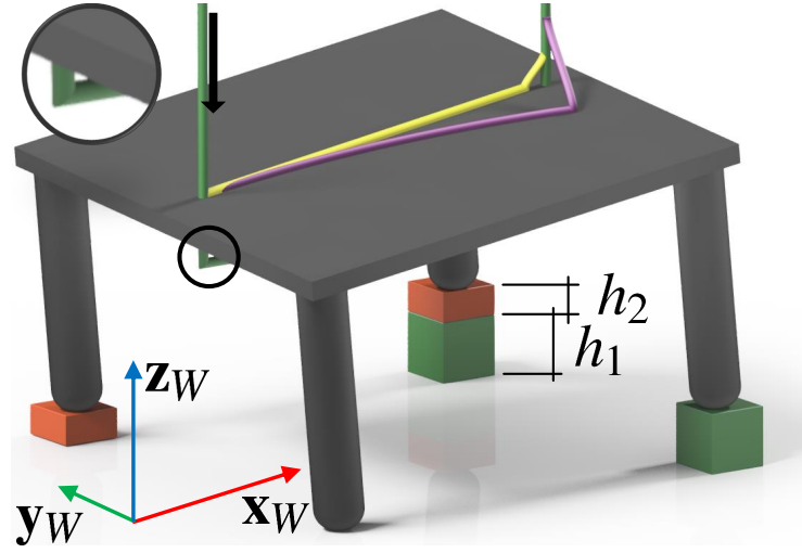
Figure 10.1 – Sliding with constant force application on a rigid, tilted surface. The black arrow indicates the direction of the trajectory. The green line represents the desired trajectory \mathbf{p}_{E,d} , which pierces the tilted surface (magnification shows the reference trajectory below the table). The yellow and violet lines represent the two reference trajectories, due to the contact forces, generated by two different values of the admittance parameter \mathbf{K}_E , which is related to the virtual spring stiffness.
