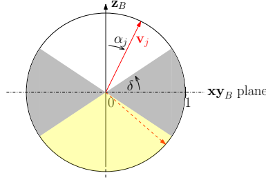
Figure 6.16 – Illustration of constraint iii ) in the design optimization.
