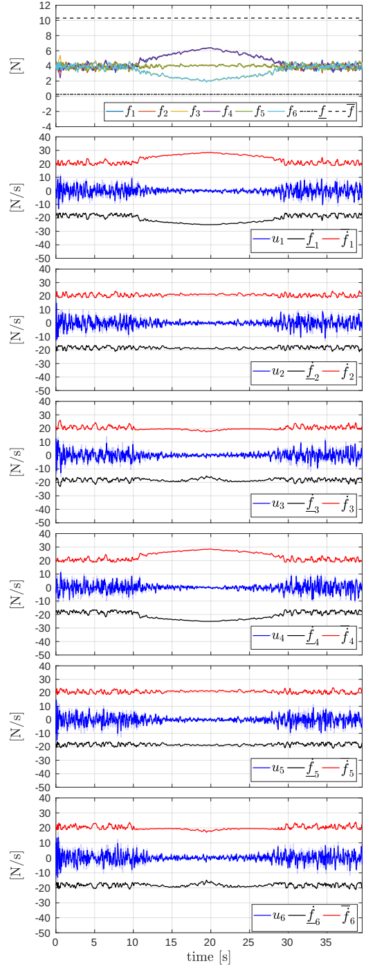
Figure 7.33 – Plots of the FAST-Hex (with variable \alpha regulated from the MPC algorithm) while hovering. The robot is disturbed with an external lateral force with a triangular profile. From top to bottom: the actuator forces and their derivatives. In particular, all the signals remain inside the feasible region delimited by the constraints.
