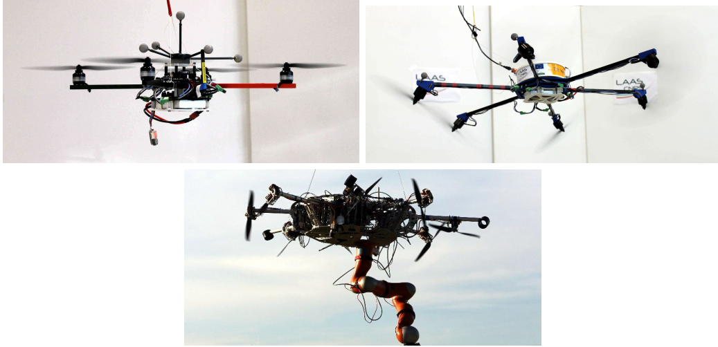
Figure 1.6 – Comparison of different UAVs. Top left : a state-of-the-art UDT quadrotor. Top right : a MDT hexarotor designed at LAAS-CNRS. Bottom : a OD (suspended) octorotor resulting from a collaboration between DLR and LAAS-CNRS.
