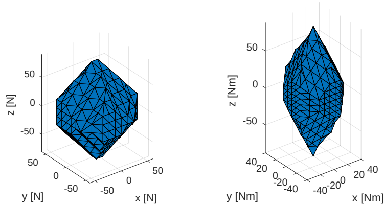
Figure 6.21 – Set of admissible forces with zero moment ( left ), used to produce a pure translation of the vehicle CoM, and set of admissible moments with zero force ( right ), used to generate a pure rotation of the body frame around the vehicle CoM.
