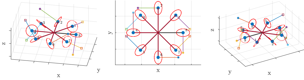
Figure 6.20 – Optimized omni-directional design for the propulsion units of the SAM. The blue spheres represent the placement of the propulsion unit motors. The colored lines point the thrust direction of each motor. The star symbol denotes the counterclockwise propeller, and the square indicates clockwise propeller.
