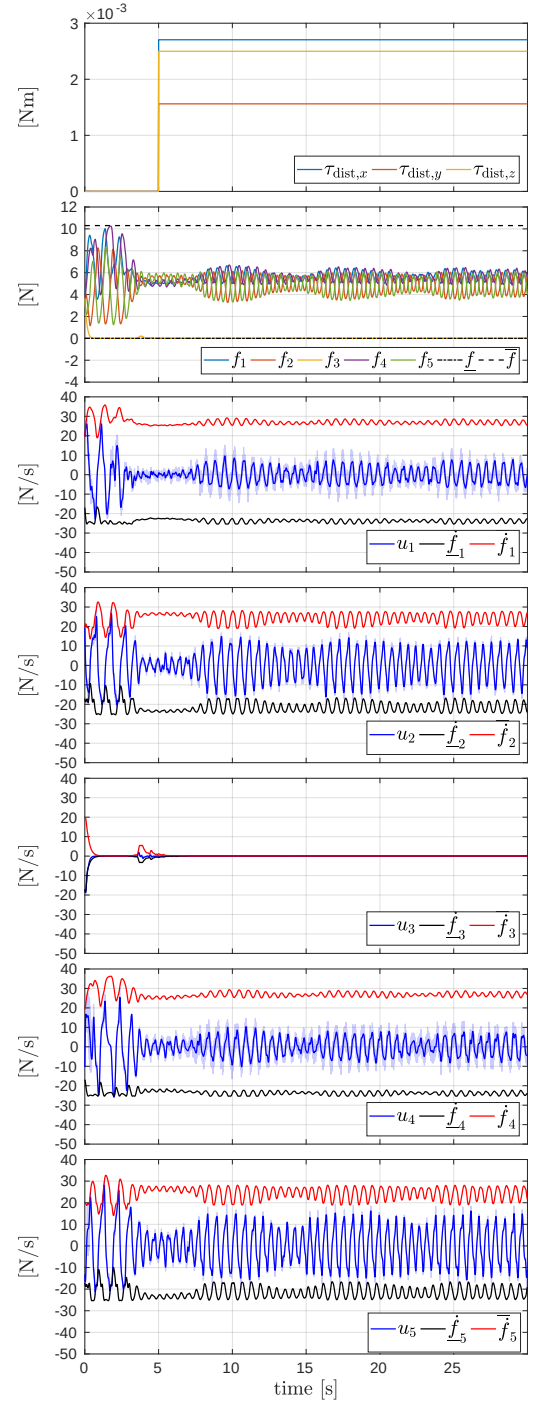
Figure 7.36 – Plots of the Tilt-Hex with rotor failure and \beta = 0 deg while hovering. The robot is disturbed with a constant external torque \tau_{\text{dist}} , activated at t = t_1 . From top to bottom : the disturbance torque, the actuator forces and their derivatives. In particular, all the signals remain inside the feasible region delimited by the constraints.
