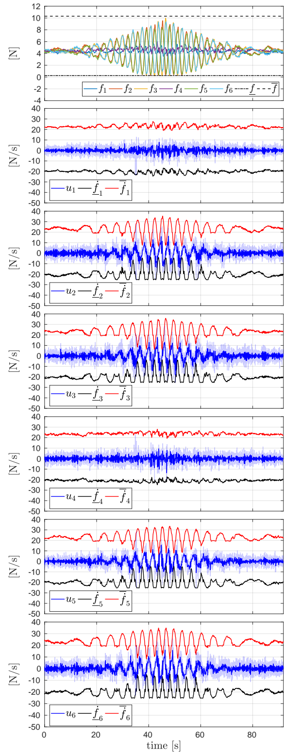
Figure 7.28 – Plots of the Tilt-Hex performing a chirp trajectory on the x-axis. From top to bottom : the actuator forces and their derivatives. In particular, all the signals remain inside the feasible region delimited by the constraints.
