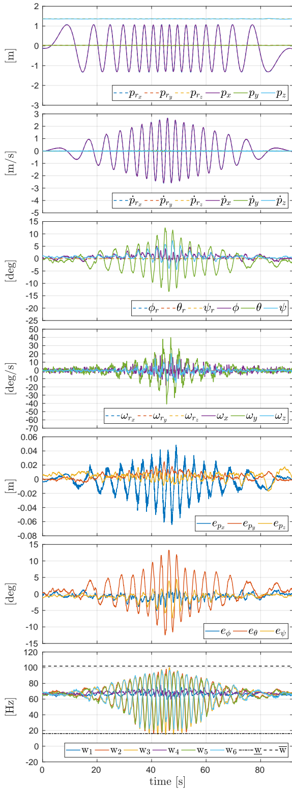
Figure 7.27 – Plots of the Tilt-Hex performing a chirp trajectory on the x-axis. From top to bottom : the position, linear velocity, orientation and angular velocity tracking, the position and orientation errors, and the rotor velocities.
