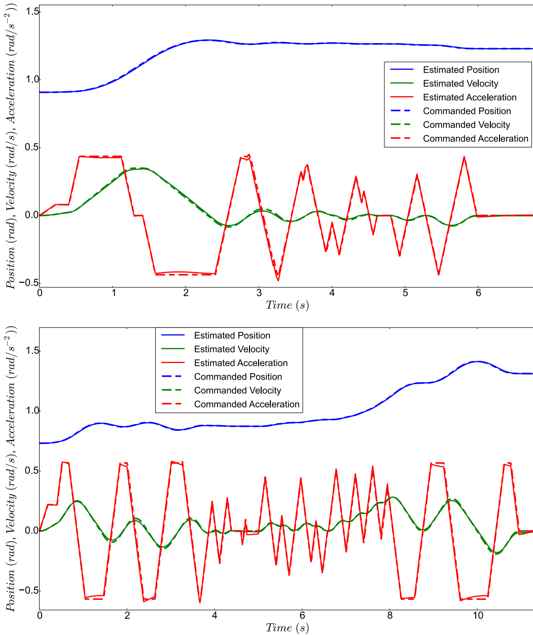
Figure 3.21: Evolution of angular trajectories during some visual servoing experiments. As the trajectory planner runs at 10Hz , trajectories are replanned multiple times while the robot is moving. Junction trajectories are used to smooth the trajectories switch.
