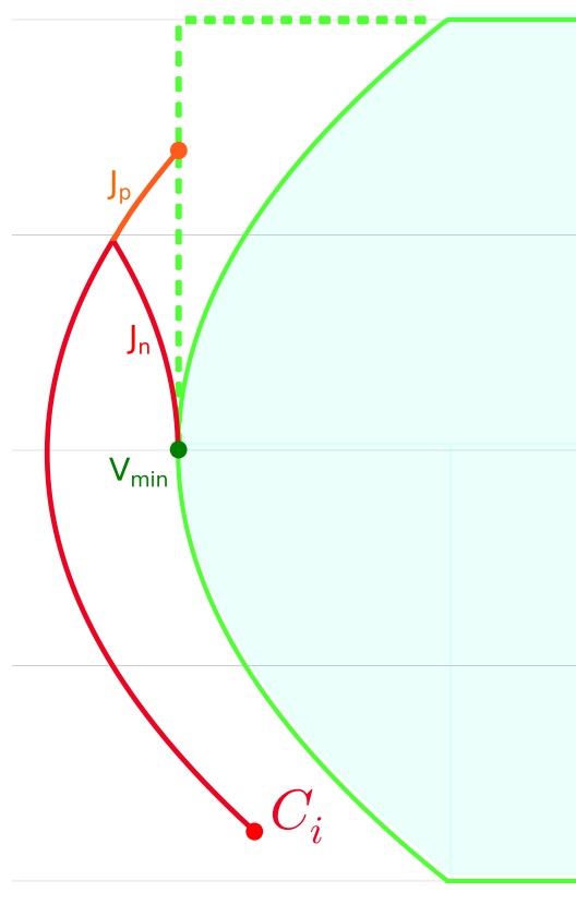
Figure 3.4: The orange trajectory represents \mathcal{T}_r computed with (Alg.2). It is the fastest trajectory the reach \mathcal{D} . The red trajectory is the fastest to reach \mathcal{V}_{min} . It is not the fastest to reach \mathcal{D} , but can be the fastest by a good margin to reach C_f if \mathcal{T}_{opt} is composed of a \mathcal{V}_{min} segment.
