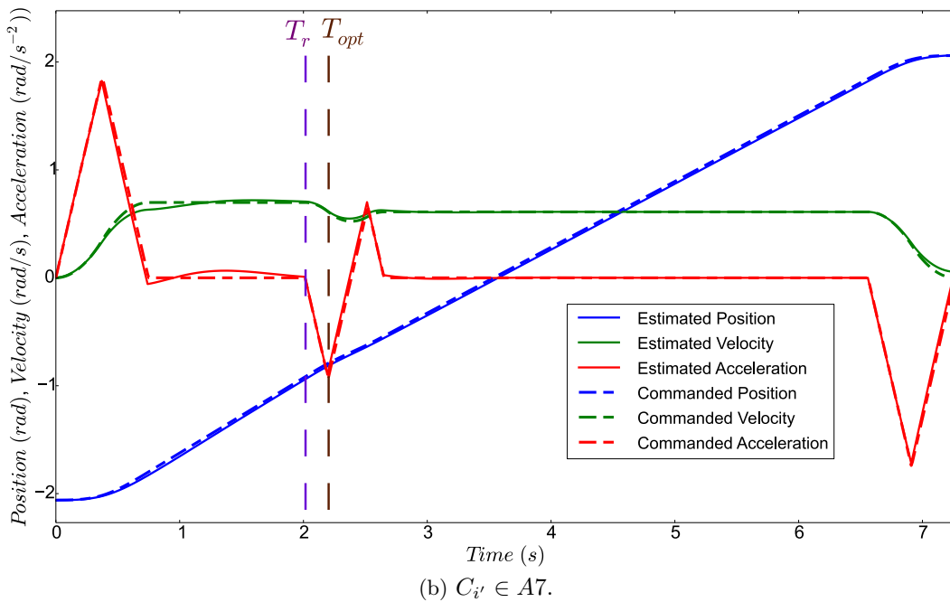
Figure 3.15: Illustration of motion constraints abrupt switch on a KUKA-LWR4 joint axis.
