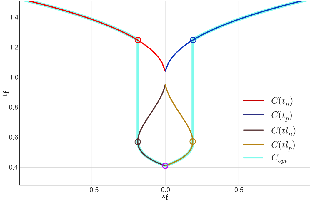
Figure 2.10: Shortcut trajectories introduce discontinuities in the time-optimal curve C_{opt} . The color circles are placed on the sides of the discontinuities that are depicted in the phase diagram in Fig. 2.11, 2.12. ( J_{min}=-40 , J_{max}=40 , A_{min}=-30 , A_{max}=30 , V_{min}=-30 , V_{max}=30 , a_i=20 , v_i=-4.99 , a_f=20 , v_f=4.99 ).
