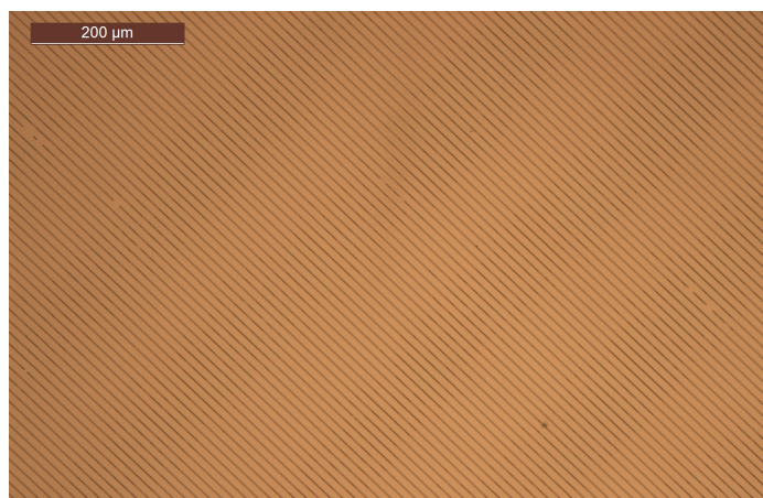
Figure 3.39.: Optical microscope observation of the center of the coverslip, 10x magnification. The sample was exposed with a dose of 100 \text{ mJ.cm}^{-2} and developed for 60 seconds in CD MF-26. Resist motifs appeared well-defined and continuous.
