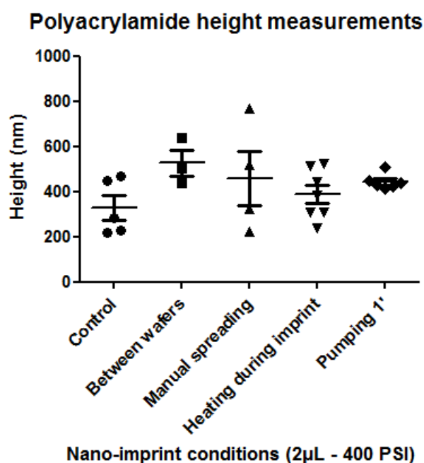
Figure 3.17.: Polyacrylamide height measurements depending on the nano-imprint conditions with NANONEX machine, corresponding to the deposition of a 2 \mu L solution volume. For the statistics corresponding to each dataset, see Table 3.2.
