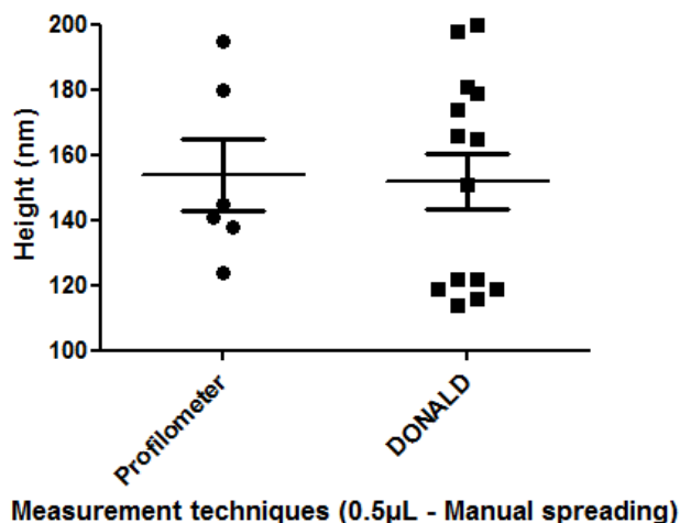
Figure 3.15.: Polyacrylamide height measurements performed with either profilometer or DONALD setup, corresponding to the deposition of a 0.5 \mu\text{L} solution volume.
