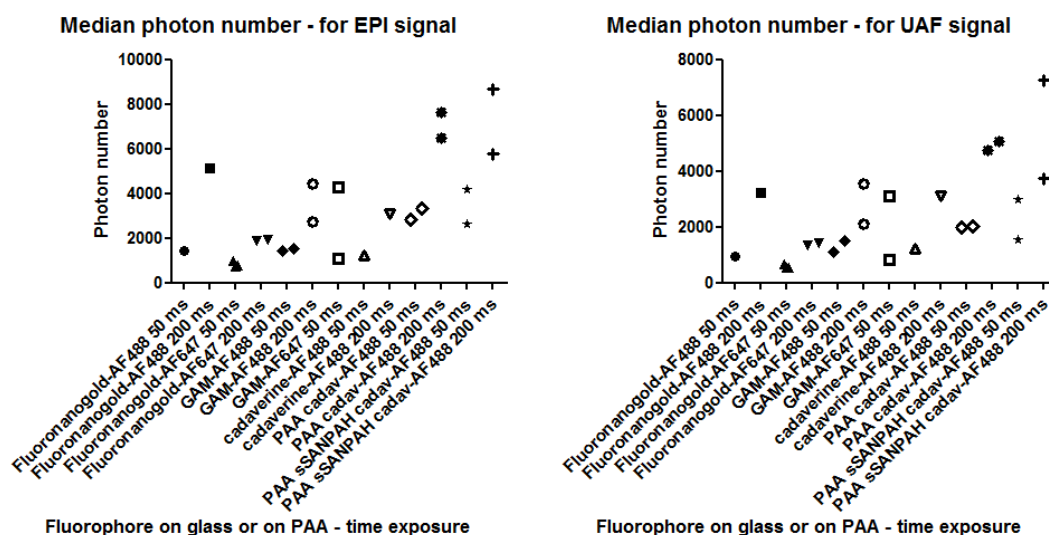
Figure 3.21.: Median photon number corresponding to EPI signal (left), and UAF signal (right), depending on the time exposure of polyacrylamide gels coated with various fluorescent markers.
