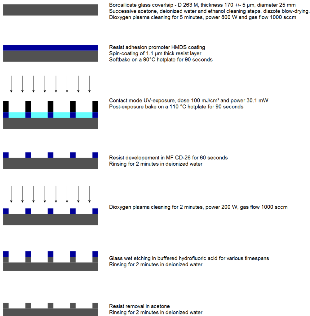
Figure 3.32.: Main steps of the optimized process to fabricate nano-topographies.
