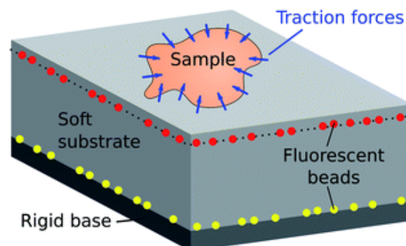
Figure 3.3.: Schematic diagram of a TFM substrate. A soft substrate (light grey) is bonded to a rigid base (dark grey). Fluorescent beads (yellow, red) are sometimes embedded at the substrate base, and near its surface. A continuous stress distribution is applied by a contractile sample, causing the displacements of fluorescent beads. Adapted from Style et al., 2014
