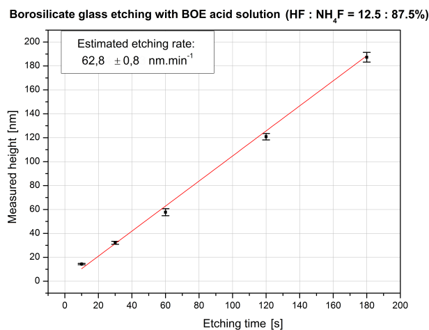
Figure 3.42.: Estimation of the etching rate of borosilicate glass by a buffered hydrofluoric acid (7:1) solution
