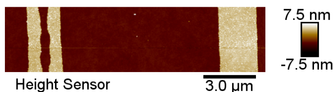
Figure 3.43.: Characteristic aspect of an etching defect observed with AFM tapping mode. The motif appeared irregular, with over-etching at its center.
