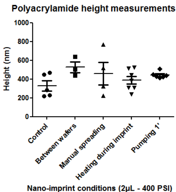
Figure 3.17.: Polyacrylamide height measurements depending on the nano-imprint conditions with NANONEX machine, corresponding to the deposition of a 2 \mu\text{L} solution volume. For the statistics corresponding to each dataset, see Table 3.2.
