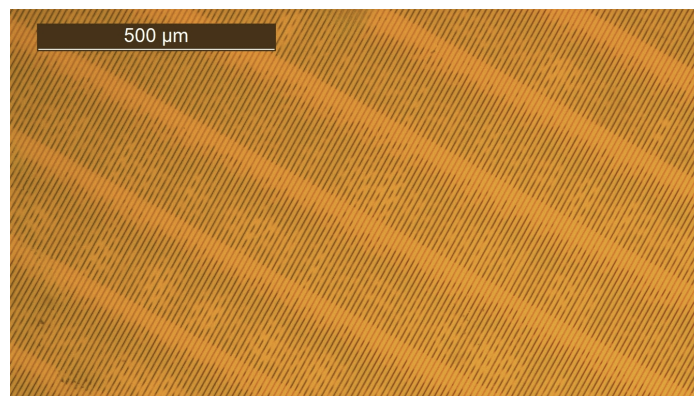
Figure 3.40.: Optical microscope observation of the center of the coverslip, 10x magnification. The sample was exposed with a dose of 100 \text{ mJ.cm}^{-2} in hard contact, and developed for 60 seconds in CD MF-26. Resist motifs discontinuities appeared periodically distributed.
