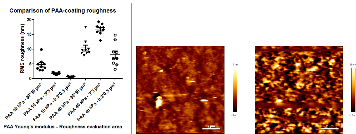
Figure 3.13.: Comparison of two polyacrylamide coating roughness with AFM (left), and the corresponding acquisitions for 10 \times 10 \mu\text{m}^2 areas for Young's modulus value of 10 kPa (center) and 40 kPa (right). For the statistics corresponding to each dataset, see Table 3.1.
