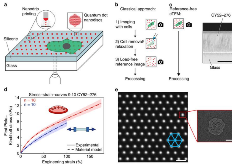
Figure 3.6.: (a) Schematic of the confocal reference-free TFM setup and involved techniques. (b) Workflow of the classical continuum approach versus the one-step confocal reference-free TFM process. (c) Scanning electron microscopy image of cross-section of elastic silicone layer on glass coverslip. Scale bar 20\mu\text{m} . (d) Results of tensile (uniaxial) and inflation (equibiaxial) testing of CY52-276 silicone. (e) Representative example of quantum dots nanodisc printing on elastic silicone substrates. Scale bar 2\mu\text{m} . Adapted from Bergert et al., 2016
