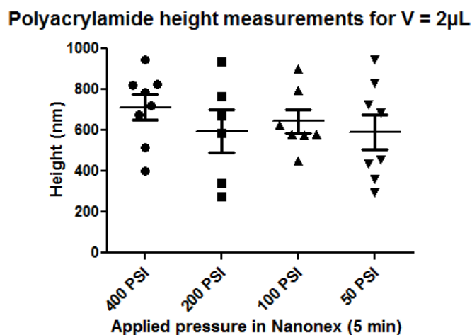
Figure 3.16.: Polyacrylamide height measurements depending on the applied pressure with NANONEX machine, corresponding to the deposition of a 2 \mu\text{L} solution volume.
