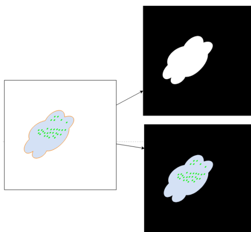
Figure 3.34.: Creation of masks based on actin fluorescence image. The binary mask allows for cell area evaluation. The other mask allows for computing mean actin intensity and podosome numbers.
