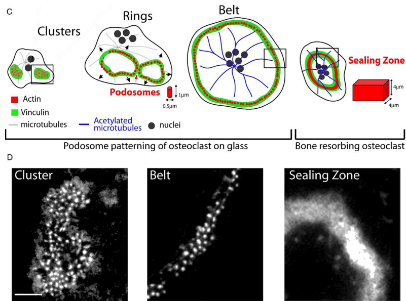
Figure 1.20.: Scheme of the different actin structures observed along osteoclast differentiation and activation. (C) At the beginning of the differentiation, podosomes are organized in clusters (C, D), which evolve into dynamics rings. These rings are stabilized at the cell periphery to form a podosome belt through the action of acetylated microtubules (C, D). When osteoclasts are adherent on surfaces containing apatite crystals, they form a sealing zone necessary for bone resorption (C, D). Adapted from Jurdic et al., 2006.
