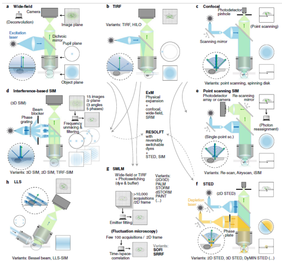
Figure 3.8.: Basic principles of super-resolution microscopy. Simplified light-paths of common conventional (a–c) and super-resolution microscopy techniques (d–h). For better comparison, all techniques are displayed in an upright configuration, though inverted configurations are more common, particularly for TIRF, SIM and SMLM systems. Adapted from Schermelleh et al., 2019
