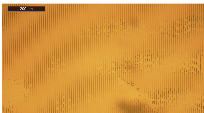
Figure 3.38.: Optical microscope observation of the center of the coverslip, 10x magnification. The sample was exposed with a dose of 100 \text{ mJ.cm}^{-2} and developed for 75 seconds in CD MF-26. Resist motifs appeared highly discontinuous and over-developed.
