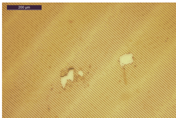
Figure 3.37.: Optical microscope observation of the center of the coverslip, 10x magnification. The sample was exposed with a dose of 100 \text{ mJ.cm}^{-2} . Resist motifs appeared more resolved and slightly under-developed.
