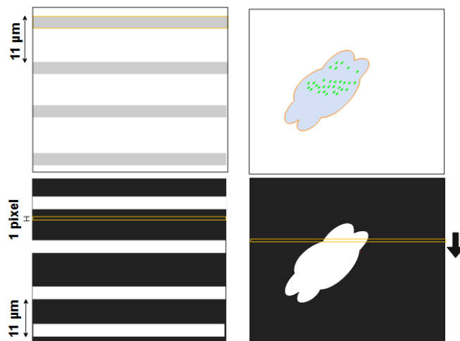
Figure 3.35.: The binary mask allows for cell area evaluation estimation by scanning the image from top to bottom and storing the mean intensity value for each scan line.
