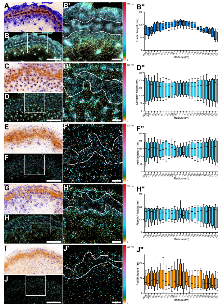
Figure 2.6.: 3D nanoscopy of F-actin, cortactin, \alpha -actinin1, filamin A and paxillin in the osteoclast podosome belt. (A) Representative dSTORM images of F-actin (purple) merged with the corresponding epifluorescence images of the F-actin cores (ochre). (B) DONALD images corresponding to (A) where the height is represented in false color (scale shown in (B')). (B') Enlarged view of (B). (B'') Height profiles of F-actin with respect to the distance to the center of the sealing zone. (C) Representative dSTORM images of cortactin (purple) merged with the corresponding epifluorescence images of the F-actin cores (ochre). (D) DONALD images corresponding to (A) where the height is represented in false color (scale shown in (D')). (D') Enlarged view of (D). (D'') Height profiles of cortactin with respect to the distance to the center of the sealing zone. (E) Representative dSTORM images of \alpha -actinin1 (purple) merged with the corresponding epifluorescence images of the F-actin cores (ochre). (F) DONALD images corresponding to (A) where the height is represented in false color (scale shown in (F')). (F') Enlarged view of (F). (F'') Height profiles of \alpha -actinin1 with respect to the distance to the center of the sealing zone. (G) Representative dSTORM images of filamin A (purple) merged with the corresponding epifluorescence images of the F-actin cores (ochre). (H) DONALD images corresponding to (A) where the height is represented in false color (scale shown in (H)). (H') Enlarged view of (H). (H'') Height profiles of filamin A with respect to the distance to the center of the sealing zone. (I) Representative dSTORM images of paxillin (purple) merged with the corresponding epifluorescence images of the F-actin cores (ochre). (J) DONALD images corresponding to (A) where the height is represented in false color (scale shown in (J')). (J') Enlarged view of (J). (J'') Height profiles of paxillin with respect to the distance to the center of the sealing zone. Scale bars: 5 \mu\text{m} (B, D, F, H, J), 1 \mu\text{m} (B', D', F', H', J').
