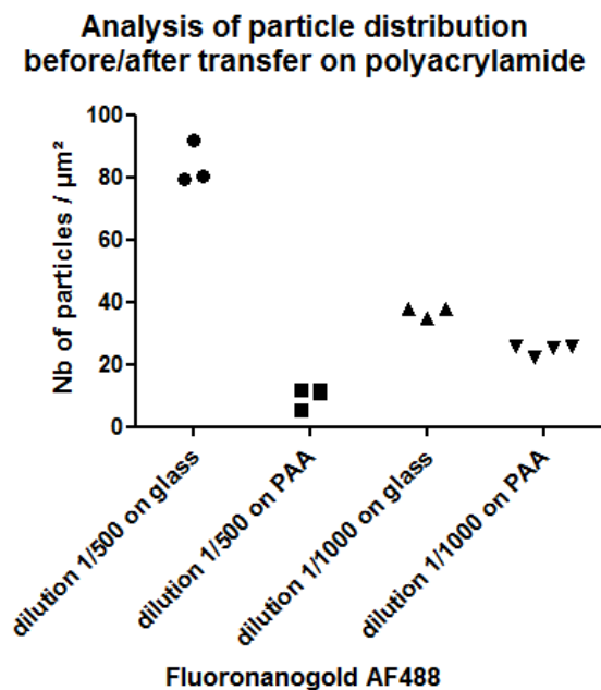
Figure 3.20.: Analysis of particle distribution before and after transfer on polyacrylamide gels, for two dilutions of AF488-coupled Fluoronanogold particles.
