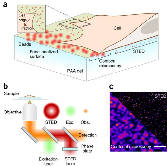
Figure 3.5.: Outline of STED-TFM. (a) Schematic representation of a typical STED-TFM setup. Traction forces applied by the cell to the top surface of the gel result in lateral displacement of the beads within the gel. (b) Schematic showing the beam path of a STED microscope. (c) Side-by-side comparison of the resolution enhancement offered by STED microscopy as compared to with confocal microscopy. Adapted from Colin-York et al., 2017
