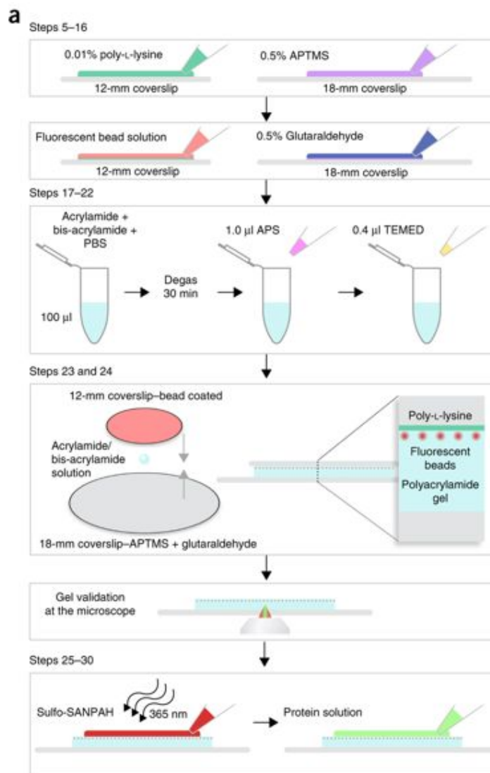
Figure 3.12.: Main steps for the preparation of polyacrylamide-coated coverslips for a traction force microscopy experiment. Adapted from Colin-York et al., 2017
