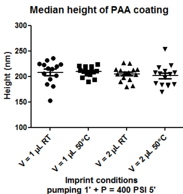
Figure 3.18.: Polyacrylamide height measurements depending on the thermal nano-imprint conditions with NANONEX machine, and the deposition of a decreasing solution volume. For the statistics corresponding to each dataset, see Table 3.3.
