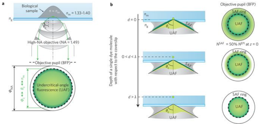
Figure 3.10.: Far and near field emission components. The far-field emission component UAF has an angular distribution determined by the law of refraction and limited by the critical angle \theta_c (left). A portion of the near field component SAF of a dye molecule located in the near-field region is collected by the objective beyond \theta_c (right). Adapted from Bourg et al., 2015
