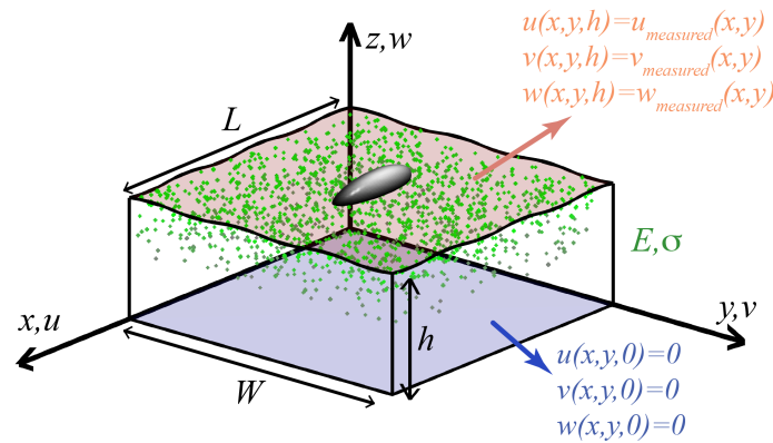
Figure 3.7.: Configuration of the 3D TFM mathematical problem. The input data are the measured three-dimensional deformation caused by the cell on the free surface of the substratum ( z = h , red), and it is assumed that the deformation of the substratum is zero at the bottom surface in contact with the glass coverslip ( z = 0 , blue). Adapted from Del Álamo et al., 2013
