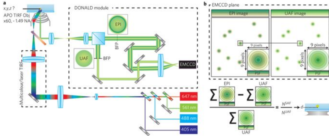
Figure 3.11.: Direct optical nanoscopy with axially localized detection setup and data analysis. A laser TIRF stage is connected to the input of a conventional wide field microscope. TIRF excitation light passes through a 4 color filter-set and an apochromatic TIRF objective of high numerical aperture. The fluorescence emission of dye molecules is collected by the objective and reflected to the DONALD module which splits the fluorescence into two parts: the EPI part is directly imaged on one half of the camera, and the UAF part is recorded on the other half (left). First, in the UAF and EPI portions of the frame, each PSF is super-localized in 2D and the number of UAF and EPI photons are computed via signal integration. Then, SAF ratio is computed and converted into the absolute dye depth d . (right) Adapted from Bourg et al., 2015
