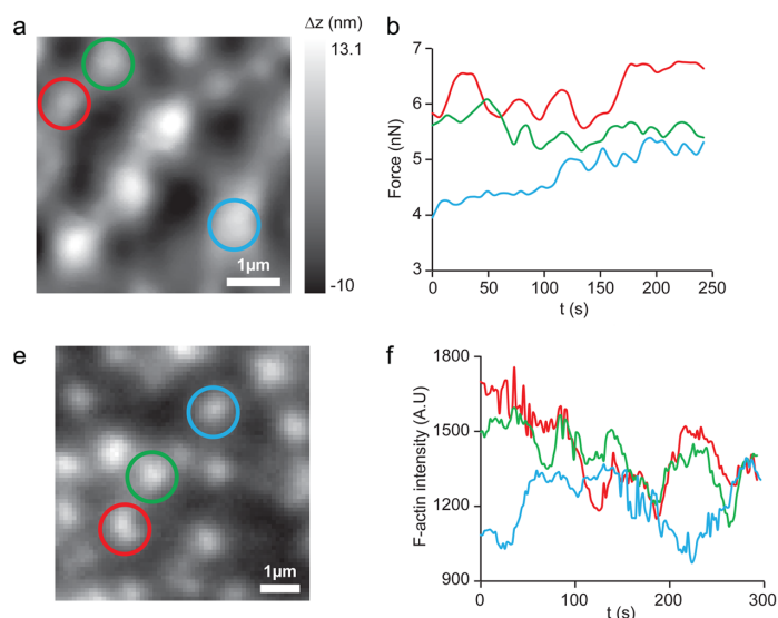
Figure 1.16.: Force and actin synchrony between close neighbors. (a,b) Time-lapse protrusion force microscopy experiments revealed oscillatory podosome-induced deformations. The synchrony coefficient is highest for red versus green and no significant synchrony was reported for red/blue and for green/blue. (e,f) Time-lapse TIRF imaging of podosome F-actin cores within a live mCherry-Lifeact-expressing macrophage. The synchrony coefficient is highest for red versus green and no significant synchrony was reported for red/blue and for green/blue. Adapted from Proag et al., 2015.
