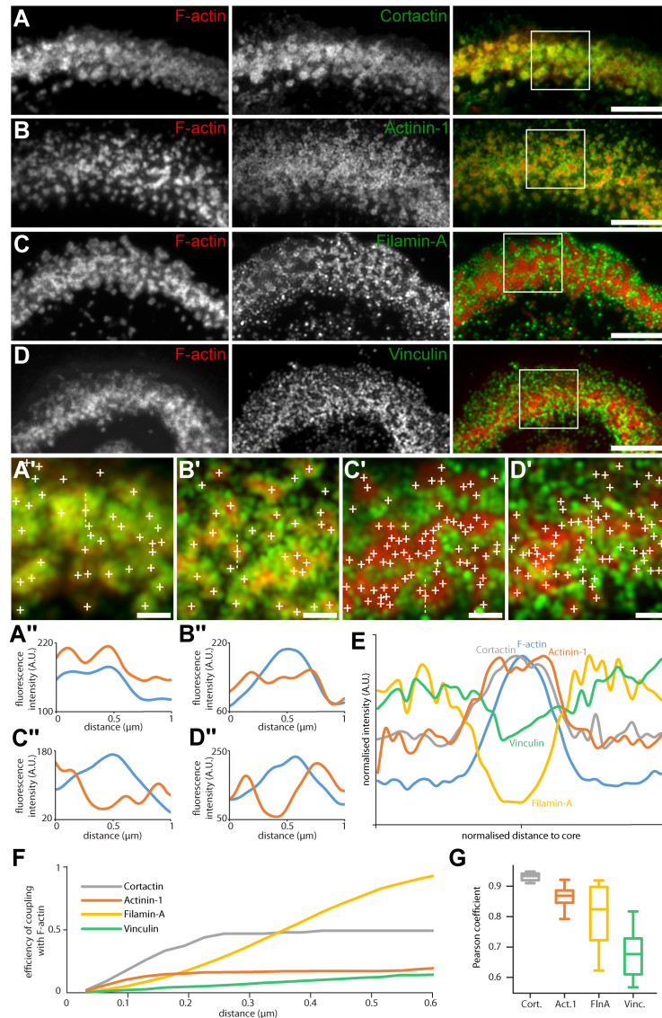
Figure 2.4.: Localization in the sealing zone of cortactin, \alpha -actinin 1, filamin A and vinculin. (A) Representative immunofluorescence images of sealing zones co-stained for F-actin (red) and cortactin (green). (A') Enlarged view of (A). (A'') Intensity profiles along the dotted lines marked in (A'). (B) Representative immunofluorescence images of sealing zones co-stained for F-actin (red) and \alpha -actinin1 (green). (B') Enlarged view of (B). (B'') Intensity profiles along the dotted lines marked in (B'). (C) Representative immunofluorescence images of sealing zones co-stained for F-actin (red) and filamin A (green). (C') Enlarged view of (C). (C'') Intensity profiles along the dotted lines marked in (C'). (D) Representative immunofluorescence images of sealing zones co-stained for F-actin (red) and vinculin (green). (D') Enlarged view of (D). (D'') Intensity profiles along the dotted lines marked in (D'). (E) Normalized intensity profiles of F-actin, cortactin, \alpha -actinin1, filamin A and vinculin (medians of 1080, 239, 265, 277, and 299 cores for each staining, respectively). (F) Efficiency of coupling with F-actin of cortactin, \alpha -actinin1, filamin A and vinculin. The curves result from a colocalization method based on the evaluation of Ripley's K function. (G) Pearson coefficient expressing the spatial correlation of cortactin-, \alpha -actinin1-, filamin A- and vinculin-associated signal intensity with actin signal intensity, respectively. Scale bars: 5 \mu\text{m} (A, B, C, D), 1 \mu\text{m} (A', B', C', D').
