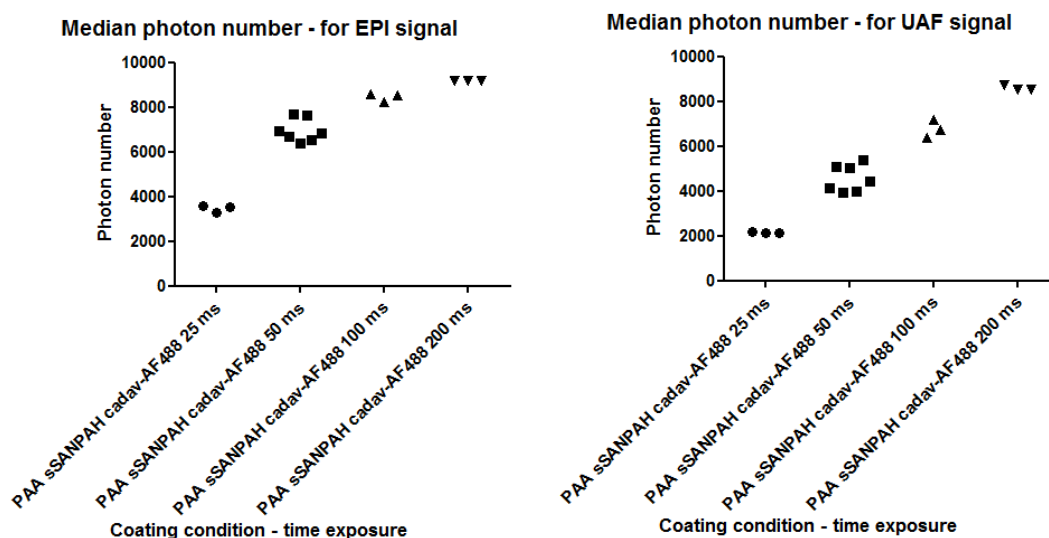
Figure 3.22.: Median photon number corresponding to EPI signal (left), and UAF signal (right), depending on the time exposure of polyacrylamide gels coated with AF488-coupled cadaverine.
