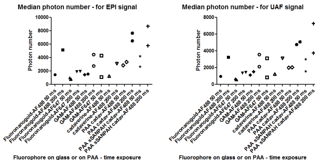
Figure 3.21.: Median photon number corresponding to EPI signal (left), and UAF signal (right), depending on the time exposure of polyacrylamide gels coated with various fluorescent markers.
