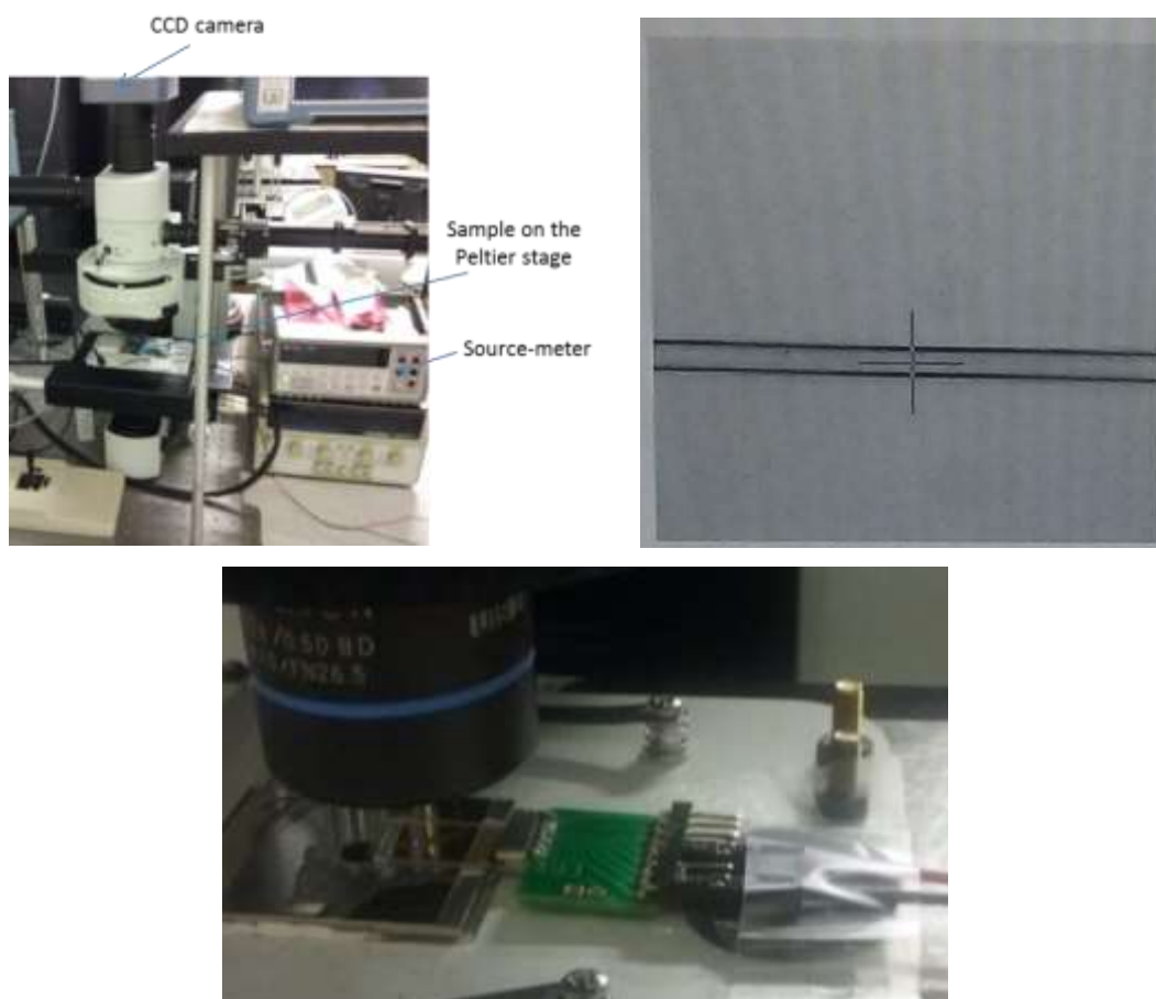
Figure 3.14: (Top, left) Photo of the experimental setup, (Top, right) Optical microscopy image of a section of a gold microwire used in our experiment. The width of the wire is 1 \mu\text{m} , its thickness is 300 nm and its length is 80 \mu\text{m} . (Bottom) Photo of the chip with the connector below the microscope objective.
