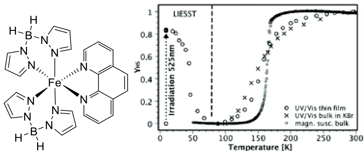
Figure 5.7: Molecular structure and spin crossover properties of the compound [\text{Fe}(\text{H}_2\text{B}(\text{pz})_2)_2(\text{phen})] . The thermal spin crossover is shown both for the bulk powder and for a thin film sample [82, 83].
