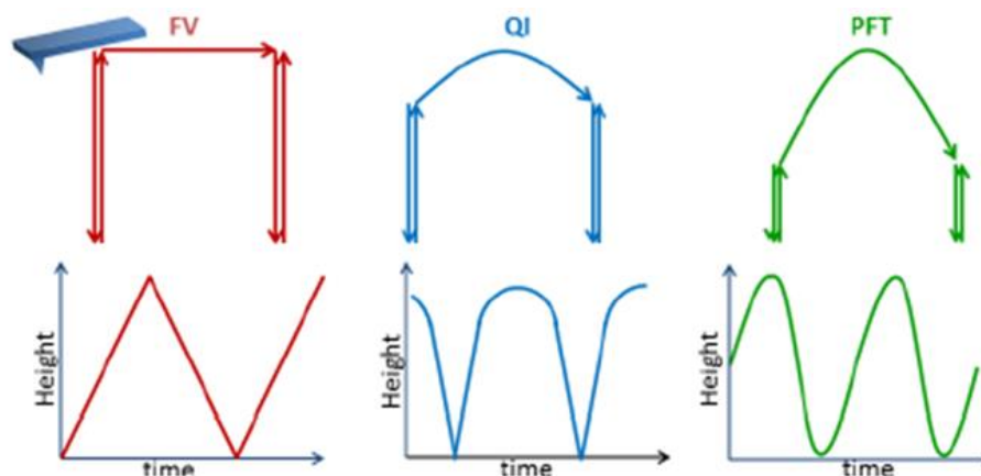
Figure 5.4: Schematic representation of the tip movement in force-volume mapping (FV), quantitative imaging (QI) and peak force tapping (PFT). The arrows show the tip movement.
