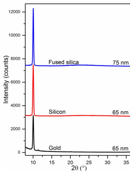
Figure 2.17: XRD patterns of solvent annealed films of [\text{Fe}(\text{HB}(\text{tz})_3)_2] on different substrates (fused silica, single crystalline silicon and polycrystalline gold).
