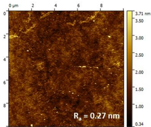
Figure A4.3.1: (Top side) AFM image of ca.30 nm film with roughness 0.27 nm; (Bottom side) Film thickness evaluation
