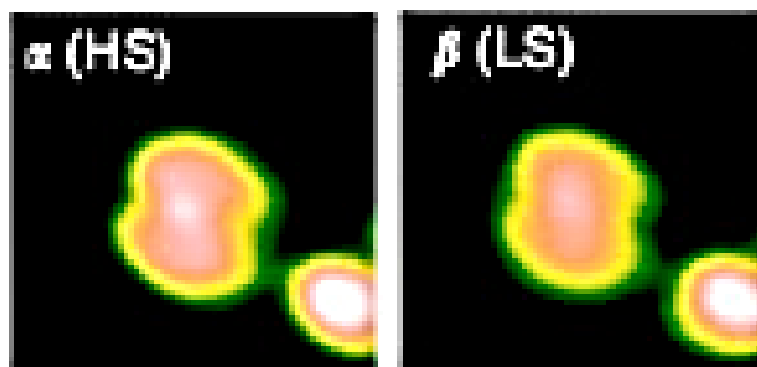
Figure 1.27: STM topographic images of a single \text{Fe}(\text{phen})_2(\text{NCS})_2 molecule in the HS and LS states. Molecules were deposited on a \text{Cu}_2\text{N}/\text{Cu}(100) substrate. Each image is 3.7 \times 3.7 \text{ nm}^2 large [91].
