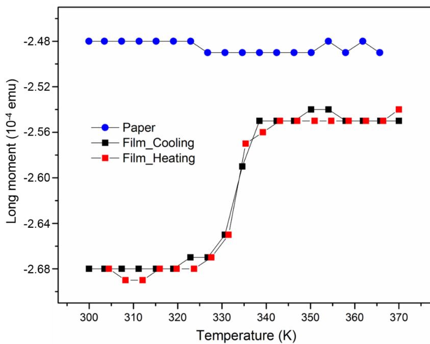
Figure A2.2.3: Temperature dependent magnetic measurements for a crystalline film of ca. 200 nm thickness, deposited on a paper substrate and rolled-on to increase the quantity of matter analyzed. Measurements were done at 2 K/min heating-cooling rate.
