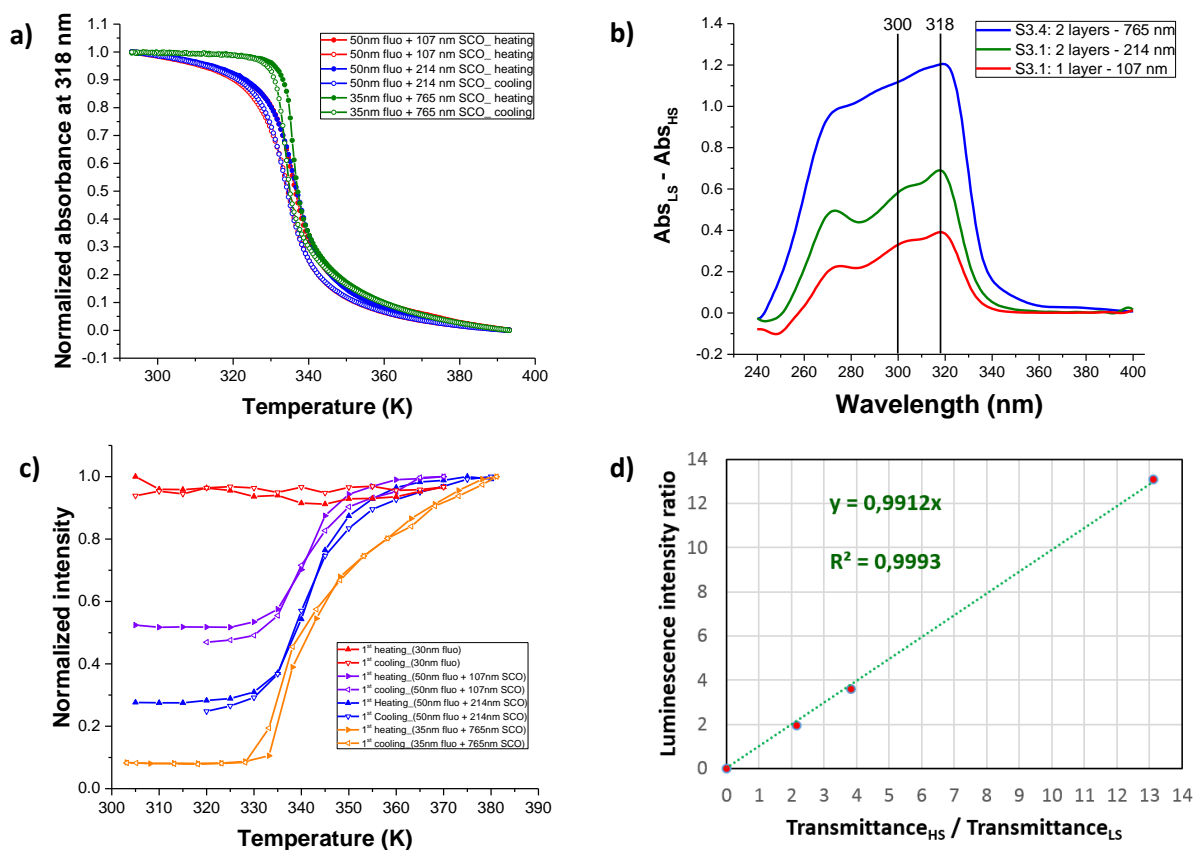
Figure 4.8: Correlation between the absorbance of [\text{Fe}(\text{HB}(\text{tz})_3)_2] and the luminescence of \text{Ir}(\text{ppy})_3 . (a) Normalized temperature dependence of the UV absorbance (at 318 nm) for three bilayer samples with different SCO layer thicknesses (107, 214 and 765 nm). (b) Absorbance changes associated with the SCO for different SCO film thickness. (c) Normalized temperature dependence of the luminescence intensity for different SCO film thickness. (d) Plot of the luminescence intensity ratio vs. the UV transmittance ratio between the HS and LS states.
