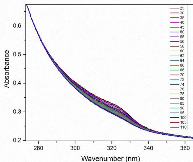
Figure 2.5: Variable temperature (in °C) UV absorbance spectra of a 30 nm thick pristine evaporated film of [\text{Fe}(\text{HB}(\text{tz})_3)_2] deposited on a fused silica substrate.
