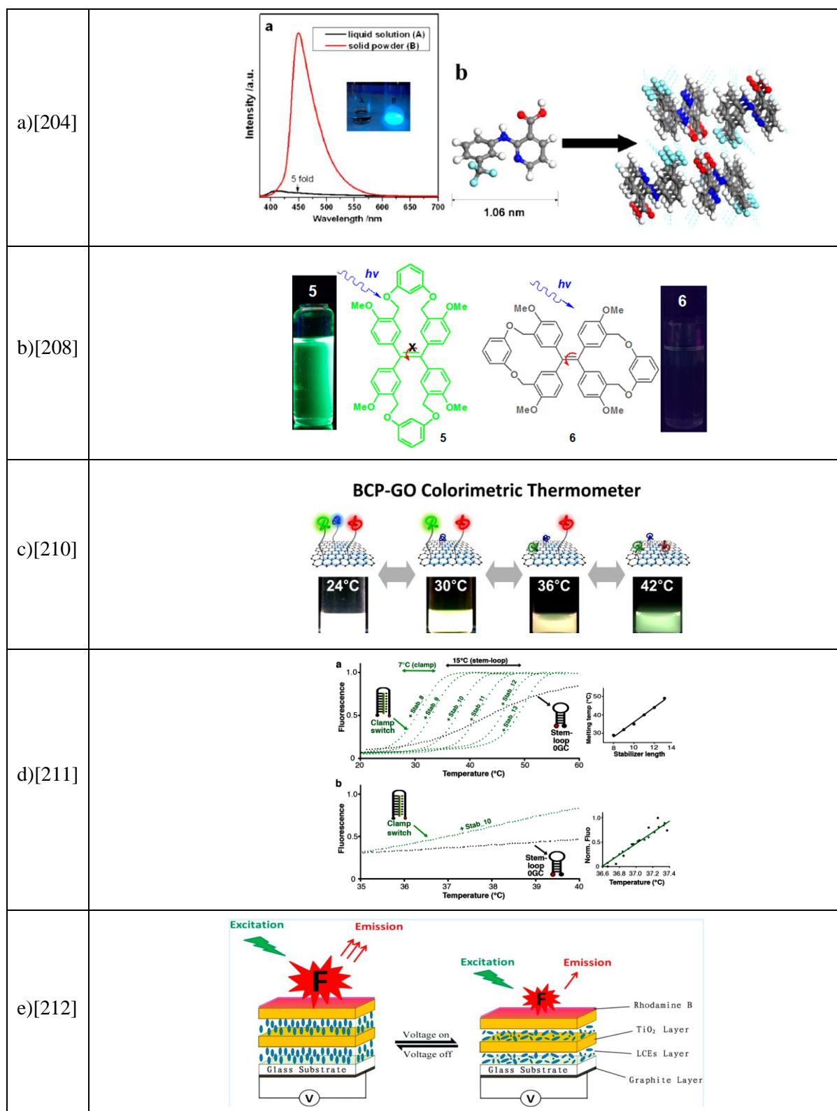
Figure 4.2: Selected examples of fluorescence switches working with physical stimuli.
