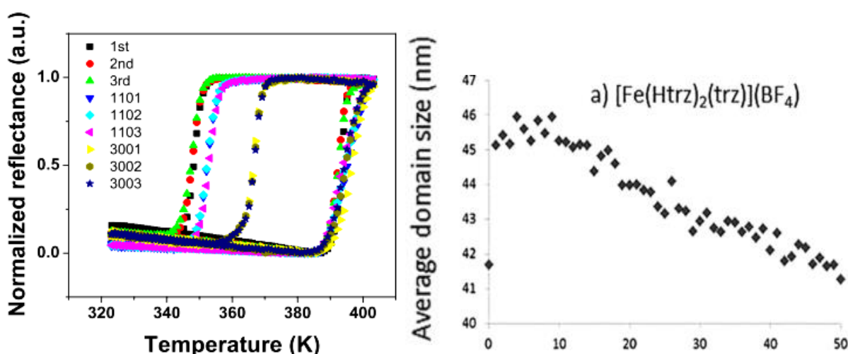
Figure 3.10: (Left panel) Thermal SCO hysteresis of [\text{Fe}(\text{Htrz})_2(\text{trz})](\text{BF}_4) before and after 1100 and 3000 consecutive cycling.[146] (Right panel) Evolution of the average crystallographic domain size in [\text{Fe}(\text{Htrz})_2(\text{trz})](\text{BF}_4) particles over 50 thermal cycles [147].
