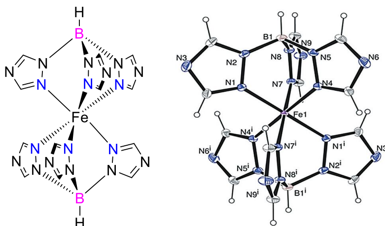
Figure 2.1: Structure du complexe [\text{Fe}(\text{HB}(\text{tz})_3)_2] .
