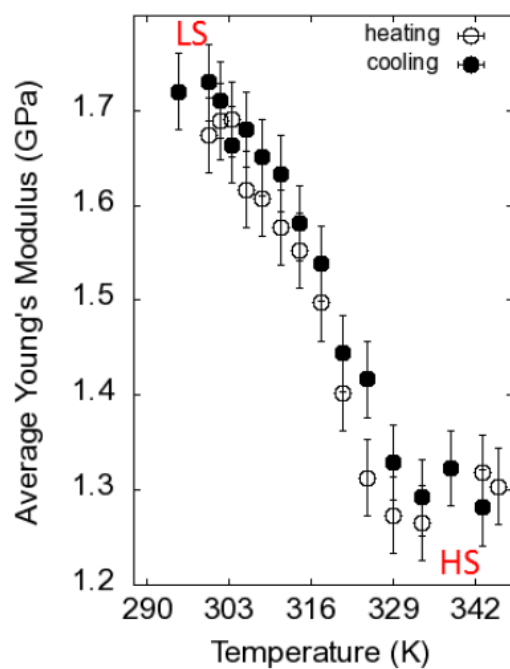
Figure 1.30: Temperature dependence of the Young's modulus of a 40 nm thick film of [Fe(hptrz) 3 ](OTs) 2 in the heating and cooling modes determined by AFM [126].
