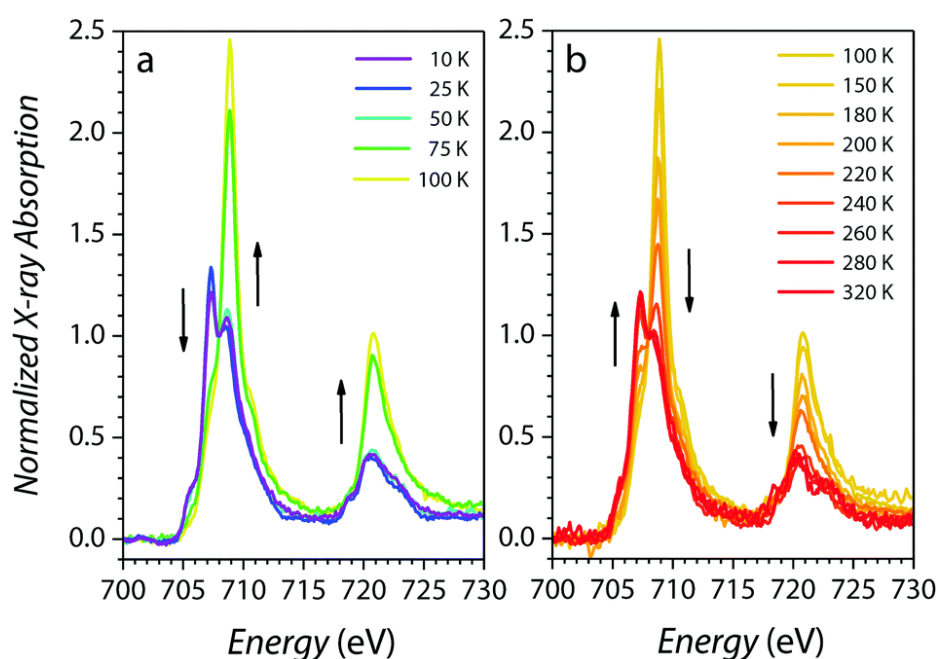
Figure 1.26: Temperature dependent XAS spectra of the SCO film [\text{Fe}(\text{qnal})_2] revealing both X-ray induced (a) and temperature induced (b) spin state changes [118].
