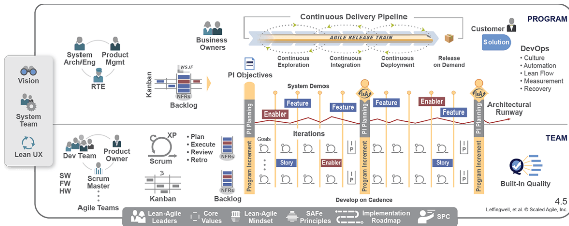
Figure 14. Essential SAFe configuration (Knaster & Leffingwell, 2017).
