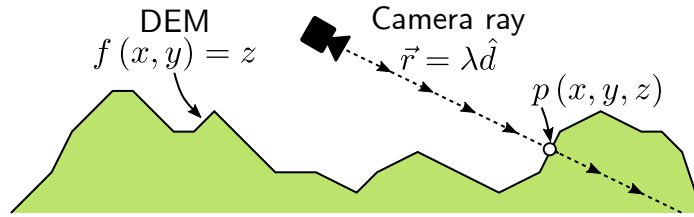
Figure 5.2: Mapping of a 2D point to a 3D earth location. It can be obtained by calculating the intersection between a ray \vec{r} cast from the camera in the direction \hat{d} of the pixel and the surface f defined by the Digital Elevation Map (DEM).
