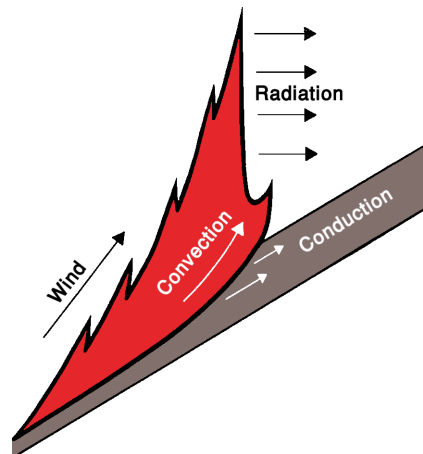
Figure 3.4: Illustration of the heat transfer mechanisms of an uphill wind-driven surface fire. Adapted from [Rothermel 1972].
