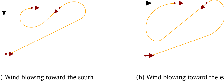
Figure 4.4: Depiction of the effect of wind over Dubins paths. Depending on the wind speed and direction, the path linking the same waypoint sequence can drastically change in shape and length. Steering while facing wind results in a tighter turn radius due to the slower ground speed. Conversely, turning in the direction of wind leads to a wider turns.
