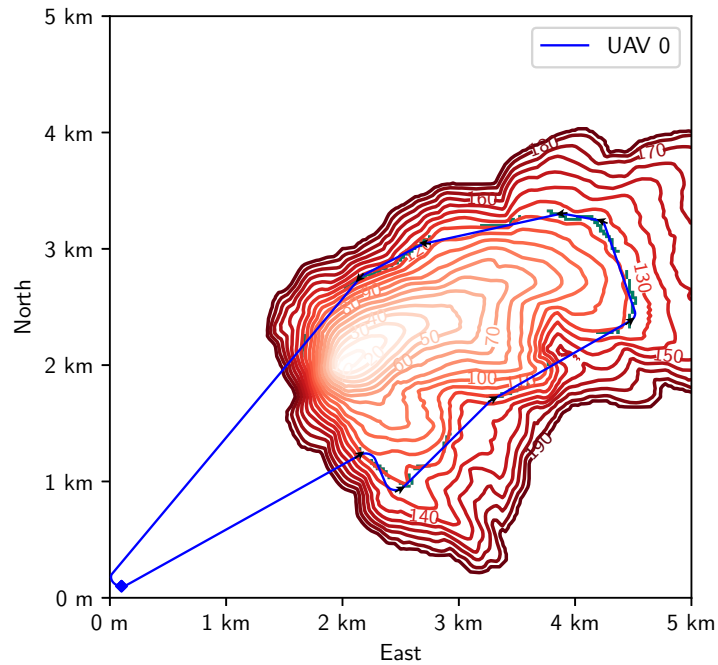
Figure 6.13: Illustration of an observation plan with strong wind blowing from the west. Note the turn radius is wider in the outbound part of the trip (south) than in the return section (north) due to the effect of wind.
