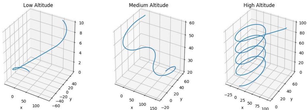
Figure 8.1: Illustration of the three types of Dubins 3D paths. The choice is derived from the difference in altitude between the origin and destination points.
