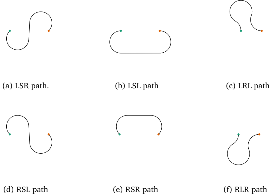
Figure 4.2: The six possible optimal standard Dubins path configurations linking two oriented points.
