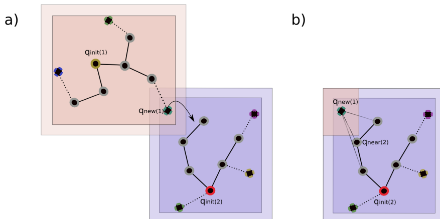
Figure 7.4. Illustration of the tree junction process. a) The extension of \mathcal{T}_1 generates a new node q_{new(1)} in the intersection of bounding n-polytopes \mathcal{S}_{1,2} . b) The processor in charge of the construction of \mathcal{T}_2 tries to connect q_{new(1)} to the nearest neighbor.
