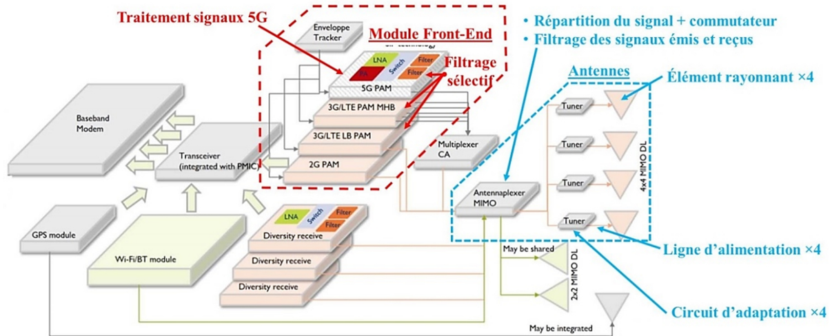
Figure I-2 : Architecture front-end d'un smartphone 5G [14].
