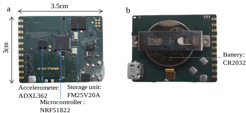
Figure 12. The sensor's basic electronic board. (a) Front side; (b) Back side.
