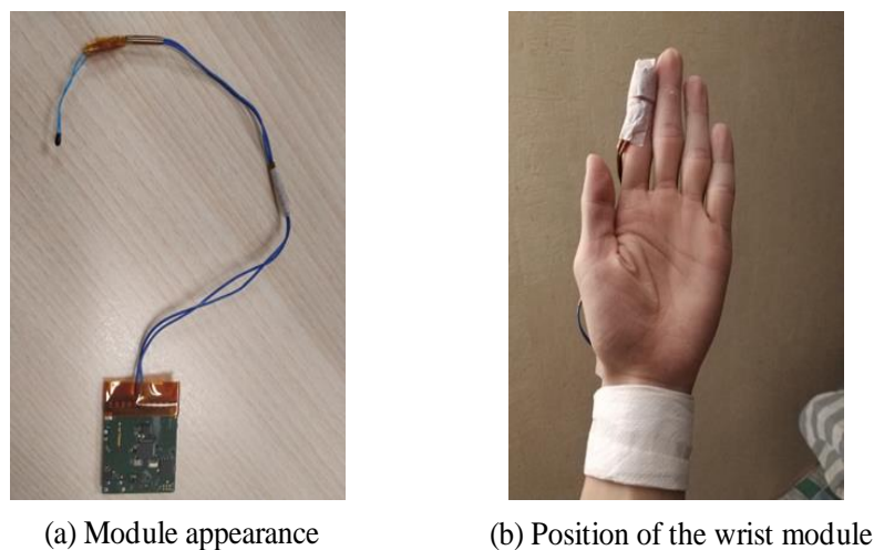
Figure 21. Wrist module.
