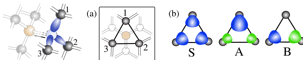
Figure 4.1: The silicon E-center projected on the vacancy-dopant axis (a) and the eigenstates of the trimer (b) constituted by the first silicon neighbours of the vacancy or atoms 1, 2 and 3.
