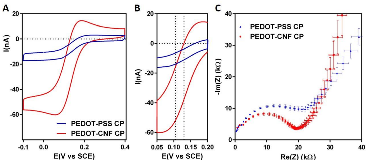
Fig. 2: Electron transfer characterization with ferri-ferrocyanide probes. (A) Cyclic voltammetry between -0.1 and 0.4V vs SCE at 50mV/s of PEDOT-PSS and PEDOT-CNF-modified microelectrode in 5mM \text{K}_3\text{Fe}(\text{CN})_6 , 100mM KCl. (B) Zoom in on the wave region. (C) Nyquist plot of modified microelectrodes at 105mV vs SCE (PEDOT-CNF) and 130mV vs SCE (PEDOT-PSS) of PEDOT-PSS and PEDOT-CNF-modified microelectrodes ( N=3 ) in 5mM \text{K}_3\text{Fe}(\text{CN})_6 , 100mM KCl. Frequency sweep between 10Hz and 7MHz, 10mV sinus, at 0V vs SCE.
