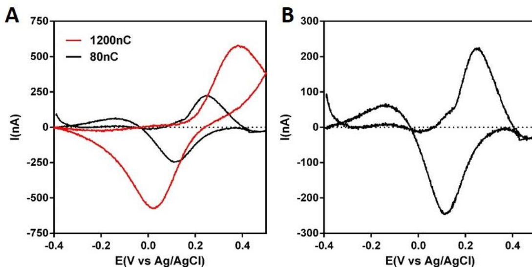
Fig. 15: FSCV electro detection of FcOH on PEDOT-CNF microelectrodes. Background subtracted voltammograms of 1mM FcOH in PBS (pH=7.2) on PEDOT-CNF deposited on gold microelectrodes (20 \mu m-diameter) by chronopotentiometry at 3.14nA with a deposition charge of A) 1200nC (red trace) and 80nC (black trace) and B) 80nC only.
