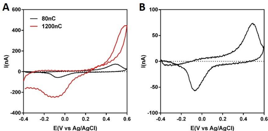
Fig. 16: FSCV electroredetection of DA on PEDOT-PSS microelectrodes. Background subtracted voltamograms of 100 \mu M DA in PBS (pH=7.2) on PEDOT-CNF deposited on gold microelectrodes (20 \mu m-diameter) by chronopotentiometry at 3.14nA with a deposition charge of A) 1200nC (red trace) and 80nC (black trace) and B) 80nC only.
