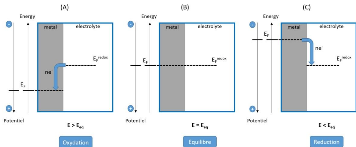
Fig. 10: Electro detection working principle. (A) The potential of the electrode (metal) is higher than the reaction potential of the redox couple in the electrolyte ( E_F^{redox} ), the electrons are then flowing from the electrolyte (which is oxidized) to the electrode. (B) Both potentials are equal, no electron flux is observed. (C) Opposite to the first scenario, the electrons are then flowing from the metal to the electrolyte, which is reduced [59].
