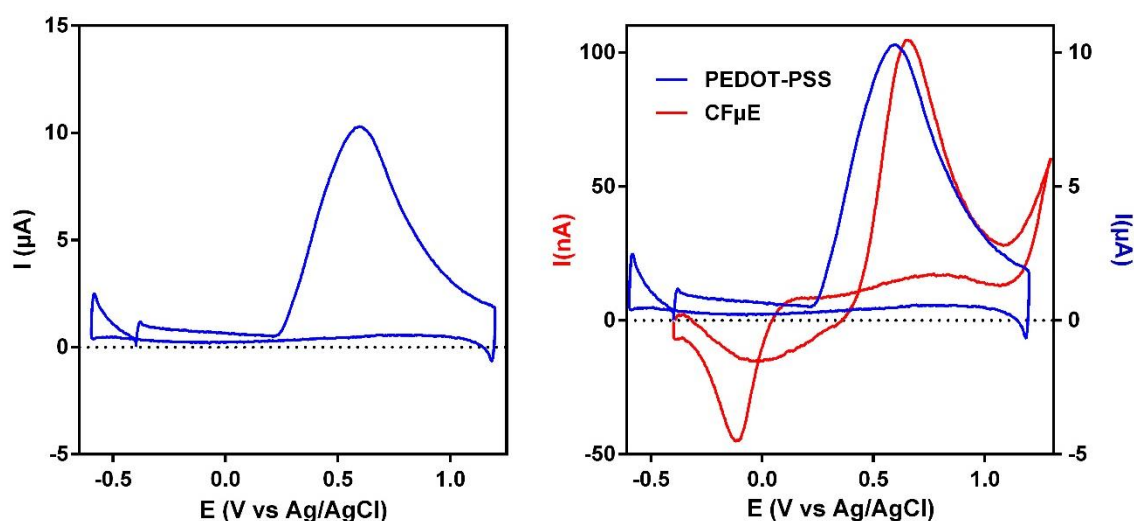
Fig. 1: Background-subtracted voltammograms (BS-V) of DA on PEDOT-PSS and CF \mu E. A) BS-V of 50\text{nM} of DA on a PEDOT-PSS microelectrode. B) Comparison of DA FSCV signature on CF \mu E (red trace) and PEDOT-PSS (blue trace).
