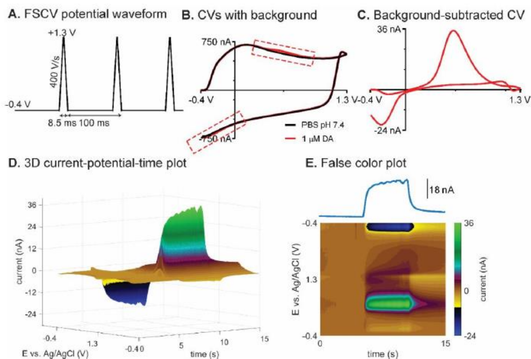
Fig. 5: FSCV realization steps exemplified with dopamine. A) FSCV potential waveform, showing the temporal progression of the potential during FSCV at 10Hz. B) CV of a CFμE with (red trace) and without (black trace) 1μM DA in PBS (pH=7.4), with the redox peaks from DA. C) Background-subtracted voltammograms, revealing the faradaic component from DA in the raw signal. D) 15s-long FSCV data set plotted in a 3D-color plot showing the rise of the DA peaks. E) Same data set as a 2D-color plot. Adapted from [1].
