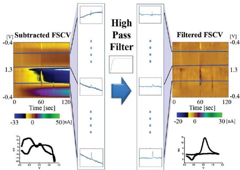
Fig. 7: Drift removal by high pass filtering. A zero-phase IIR Butterworth HPF was applied to \text{current} = f(\text{time}) data recorded at each voltage (horizontal blue lines). In this illustration, a 1 \mu\text{M} bolus of dopamine in a Tris buffer was injected in a flow cell and the background drift was removed by the filter leaving only the signal due to the presence of dopamine. [17]
