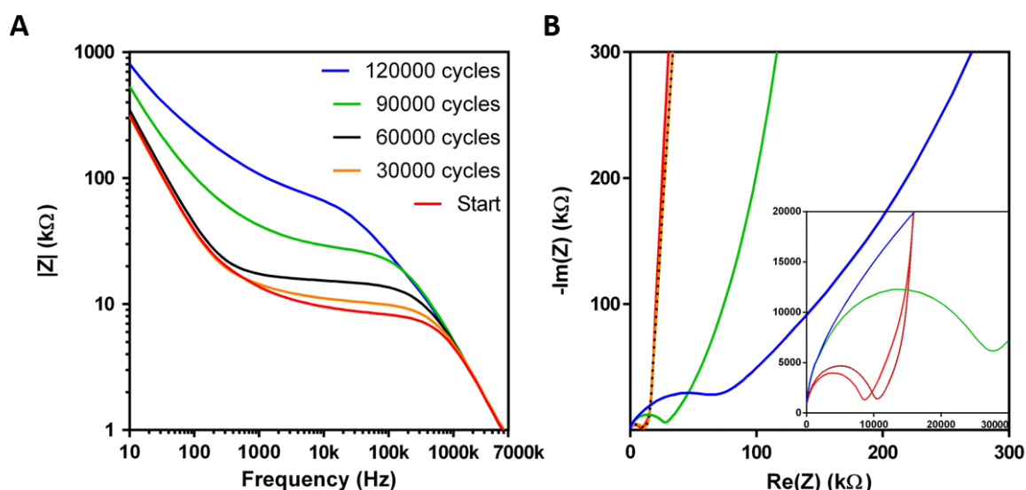
Fig. 10: EIS monitoring of a PEDOT-CNF microelectrode during in-vitro stimulation, pulsing at CIL/10 ( \approx 3,15\mu A ), at 1Hz in PBS (pH=7,2). EIS realized at 0V vs SCE, with a 10mV sinus, between 10Hz and 7MHz. A) Bode plot change and B) Nyquist plot change in function of number of cycles passed through the electrode.
