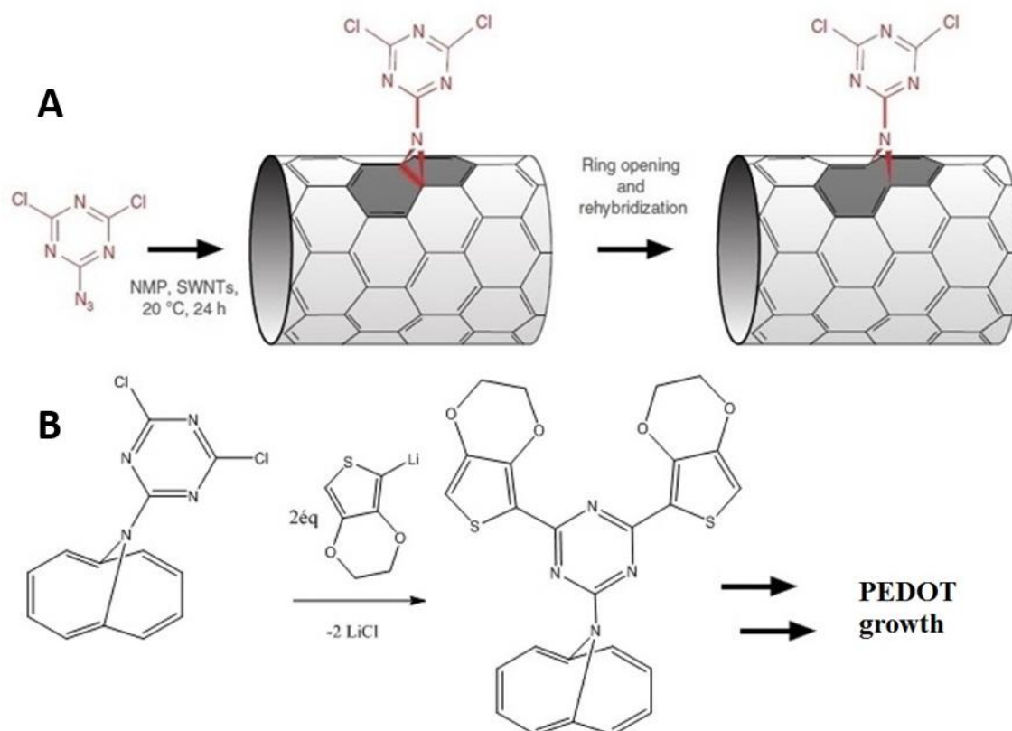
Fig. 4: Functionalization pathway of a carbon nanomaterial (here SWNTs as model for representation) to covalently graft EDOT moieties on its surface by using a delocalized spacer, to connect PEDOT chains to the carbon nanomaterial and take advantage of its conductive skeleton for electron/hole transfer and potential recording.
