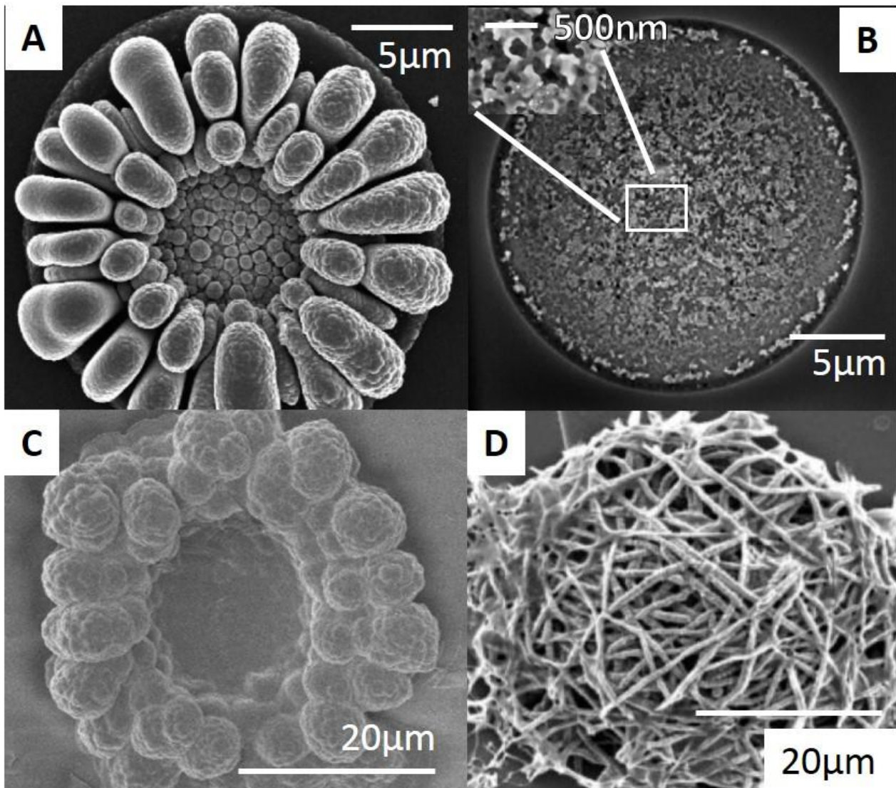
Fig. 7: Modified microelectrodes examples from the literature. (A) Sun flower-shaped nanostructured gold deposit on a gold 10μm-diameter microelectrode, reproduced from [36], (B) Gold nanoporous microelectrodes obtained after removal of an aluminum matrix by chemical etching [38], (C) PEDOT-PSS coating obtained using the protocol from [37] on a gold 20μm-diameter microelectrode. (D) Conducting polymer nanotubes grown on a metallic microelectrode from [39].
