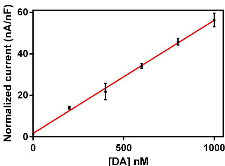
Fig. 13: Calibration curve of FSCV electrodetected dopamine on carbon fiber microelectrodes (N=3). Current measured at the oxidation peak maximum and normalized by the integration of the current in the CF \mu\text{E} voltammogram on the measured cycle. Dopamine concentrations: 200, 400, 600, 800 and 1000nM. Same FSCV parameters. R^2=0.9975 and S=54.49 \text{ nA}/\mu\text{M} .
