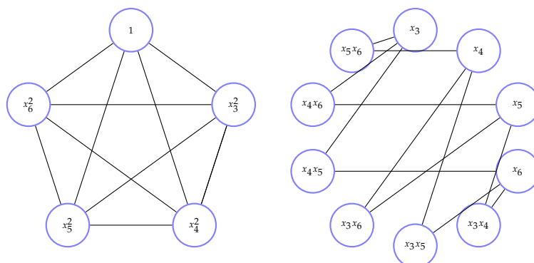
Figure 3.13: The \text{tsp} graph for the second clique of Example 3.5.2
