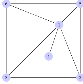
Figure 3.2: csp graph for the variables of f from Example 3.1.1.
