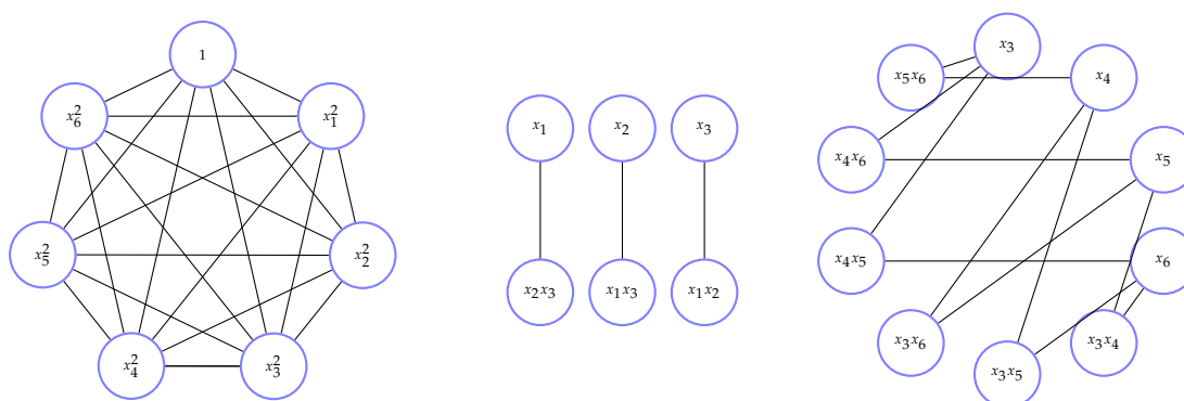
Figure 3.14: The \text{tsp} graph without partitioning variables of Example 3.5.2
