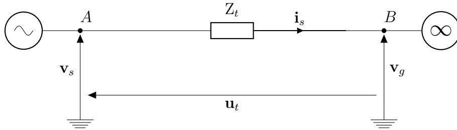
Figure 3.7 – The equivalent simplified SMIB model.
