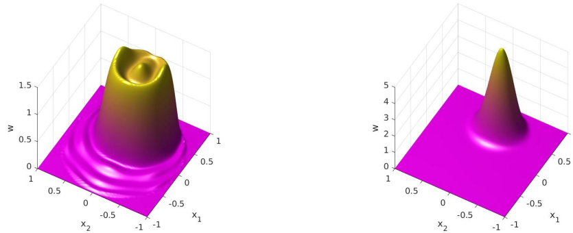
Figure 4.2 – Polynomials obtained with and without Stokes constraints.
