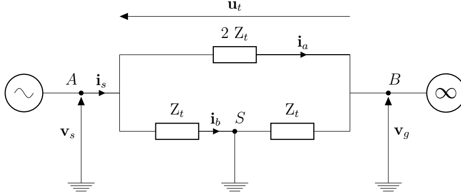
Figure 3.8 – The short-circuited system.
