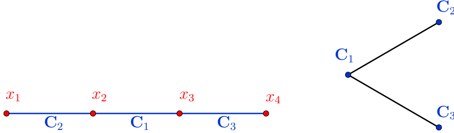
(b) branched clique tree.
