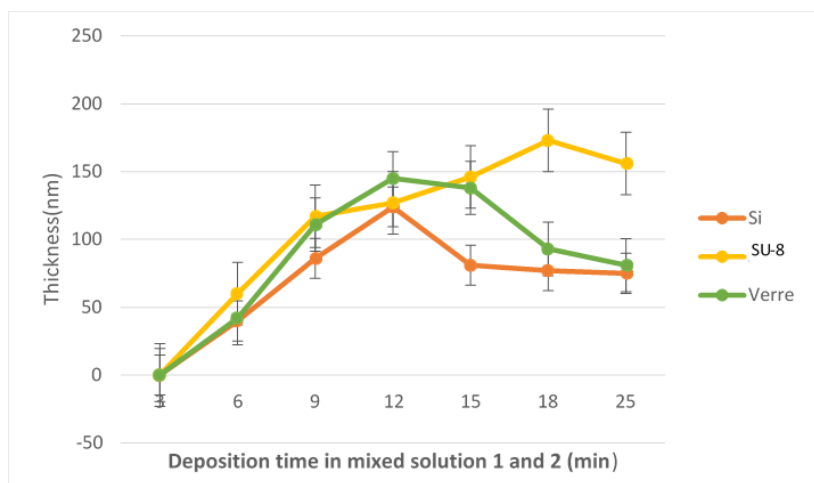
Figure 107. The evolution in the thickness of the PANI layer, deposited on Si, SU-8 and glass substrates over deposition time.
