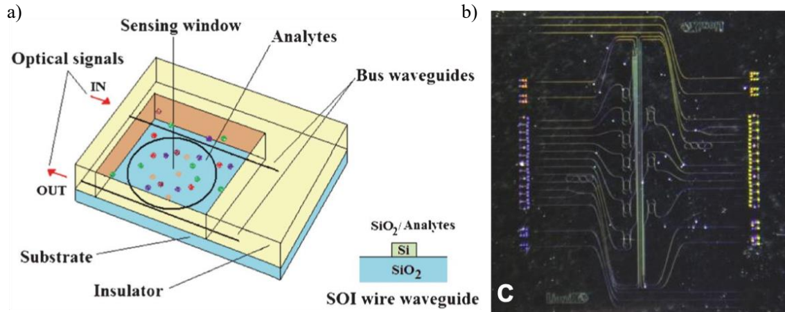
Figure 1. a) Schematic of a planar micro-resonator implemented in Silicon On Insulator technology [7]. b) Illustration of high density integration of micro ring resonators on a 1x1 cm chip using the TriPlex technology [8].
