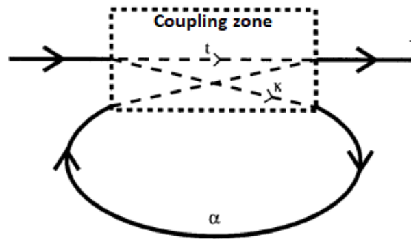
Figure 60. Energy coupling schematic between a waveguide and a lateral micro resonator.
