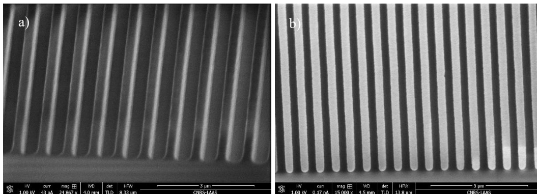
Figure 84. a) Grating coupler patterns in LOR+ECl obtained after photolithography with exposure doses between 1000 to 1100 J/m 2 . b) Aluminium grating coupler obtained after completion of the lift-off process.
