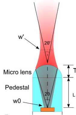
Figure 17. Dimensions involved in microlens design
