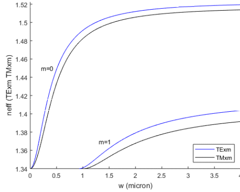
Figure 53. Dispersion curves at 850nm of TE_{xm} and TM_{xn} modes in a three-layer structure CYTOP/SU-8/CYTOP. The thickness of layer SU-8 is less than 800nm.
