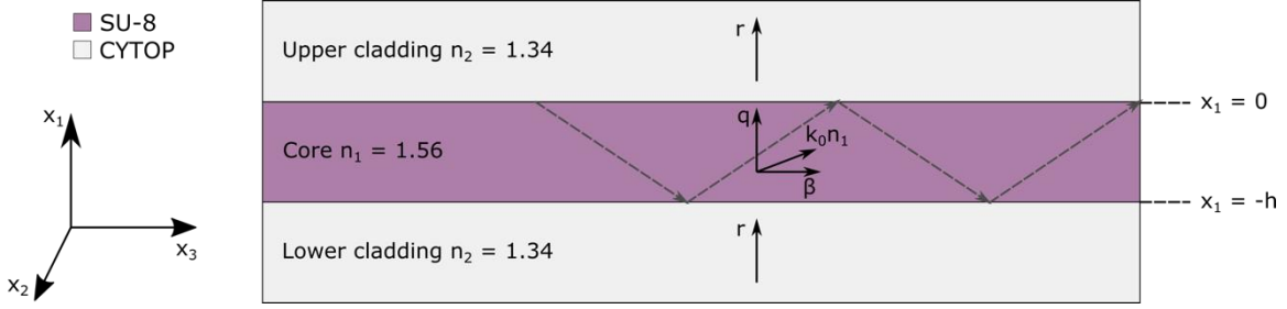
Figure 50. The 3-layer planar waveguide and its associated relative wave vectors.
