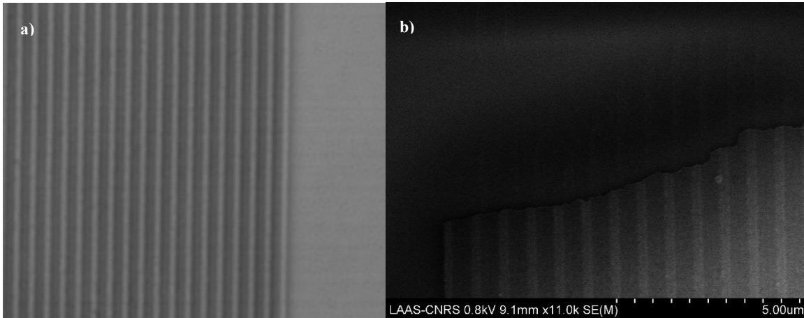
Figure 77. a) nLOF grating couplers after photolithography, without formed undercut. b) The evaporated Al forms a slice of film rather than separated stripes after etching.
