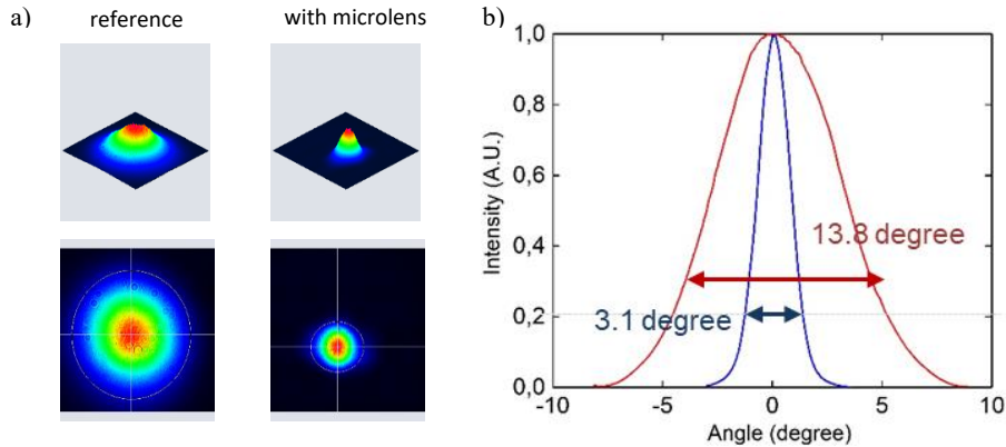
Figure 47. a) Beam profiles without and without microlens measured at 3mA. b) Divergence of VCSEL with or without micro lens fabricated by 2PP 3D printing.
