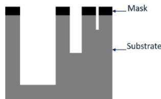
Figure 97. For the same material, the etch rate is lower on a smaller pattern during the plasma etching.
