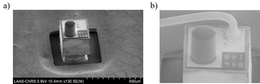
Figure 44. View of a VCSEL chip with a 3D printed lens in single step before (a) and after (b) wire bonding.
