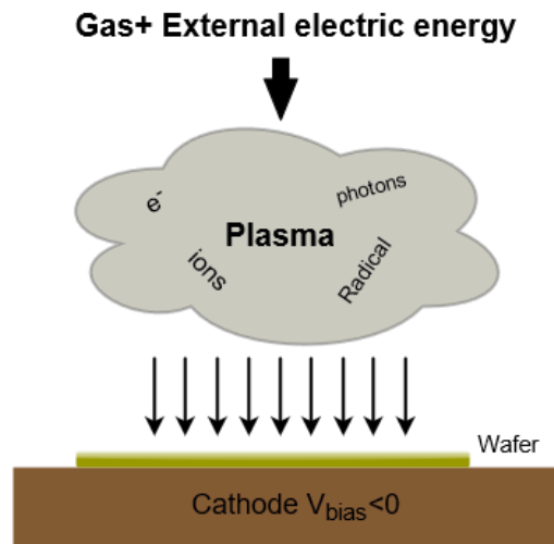
Figure 94. Schema of plasma etching.
