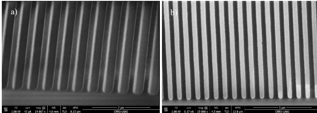
Figure 84. a) Grating coupler patterns in LOR+ECI obtained after photolithography with exposure doses between 1000 to 1100 J/m 2 . b) Aluminium grating coupler obtained after completion of the lift-off process.
