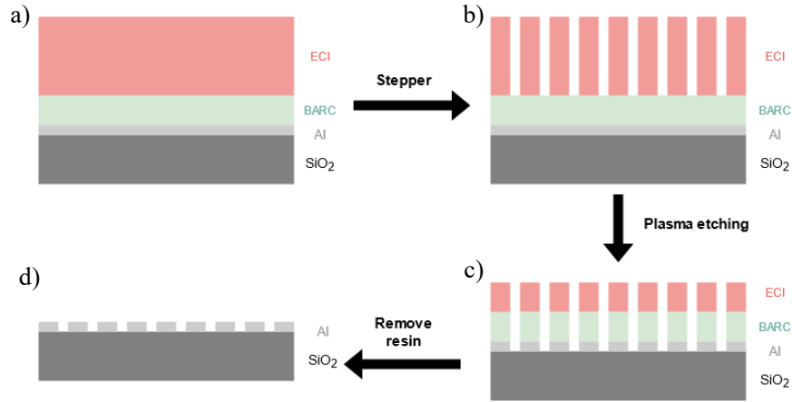
Figure 96. Process workflow for the fabrication of Al grating couplers over the SiO_2 lower cladding.
