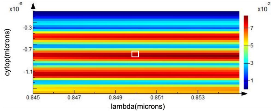
Figure 62. The variation of coupling efficiency versus CYTOP bottom cladding thickness.
