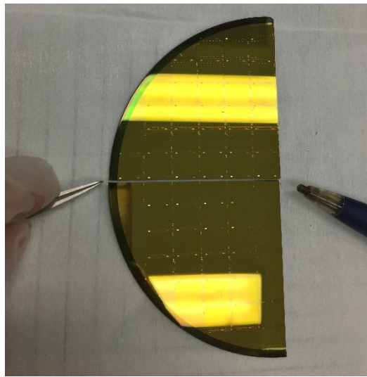
Figure 90. Two-point pressing method for wafer cutting without damaging the patterns.
