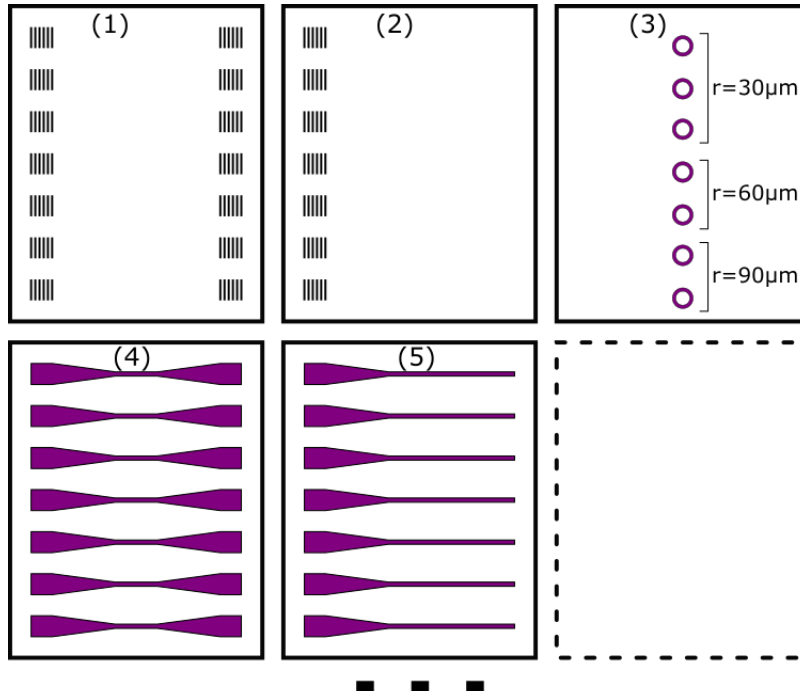
Figure 65. Schematic representation of the five over nine areas available on the reticle. Each pattern will cover a 6.2x7.2mm 2 on the wafer. A complete micro-resonator will be a combination of three areas of the reticle. Note: the polarity is not respected for better graphic rendering of the schematic.
