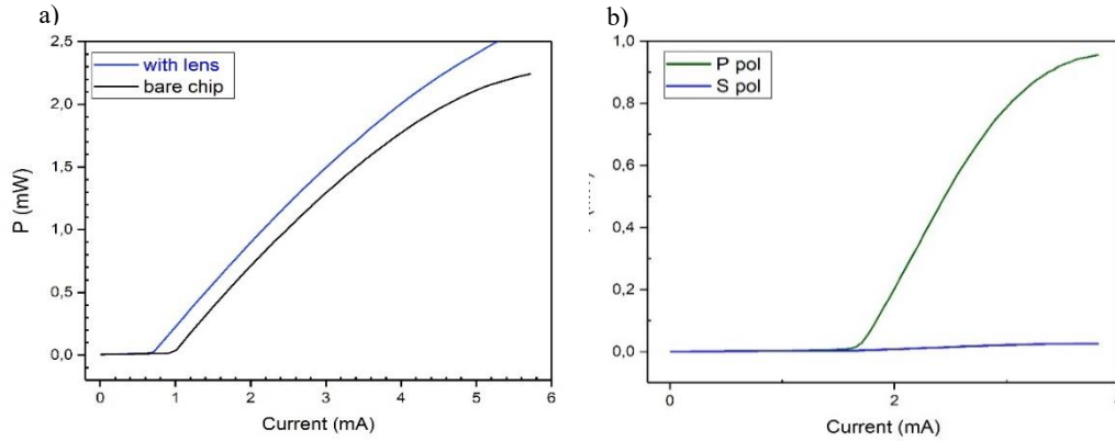
Figure 46. a) L(I) curve of VCSEL with and without 3D printed micro lens. b) Polarization-resolved L(I) curve of VCSEL with 2PP 3D printed micro lens.
