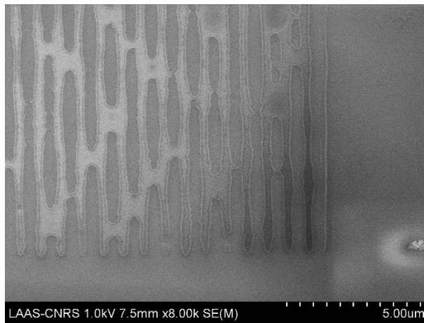
Figure 73. Irregular aluminum grating coupler lines after wet etching.
