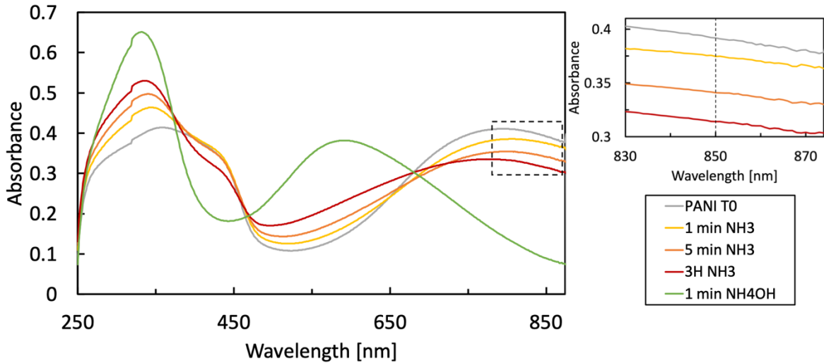
Figure 111. UV-VIS absorption spectra of PANI coated glass substrates upon different exposure times to \text{NH}_3 and \text{NH}_4\text{OH} . Inset focuses on the absorbance variation around 850 nm.
