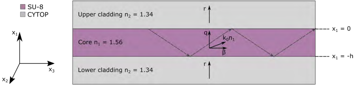
Figure 50. The 3-layer planar waveguide and its associated relative wave vectors.
