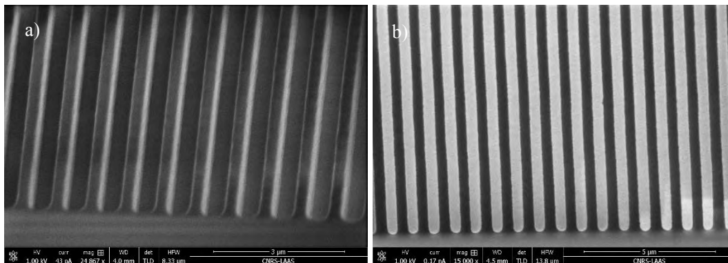
Figure 84. a) Grating coupler patterns in LOR+ECI obtained after photolithography with exposure doses between 1000 to 1100 J/m 2 . b) Aluminium grating coupler obtained after completion of the lift-off process.
