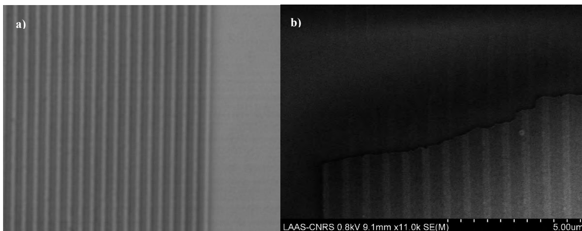
Figure 77. a) nLOF grating couplers after photolithography, without formed undercut. b) The evaporated Al forms a slice of film rather than separated stripes after etching.
