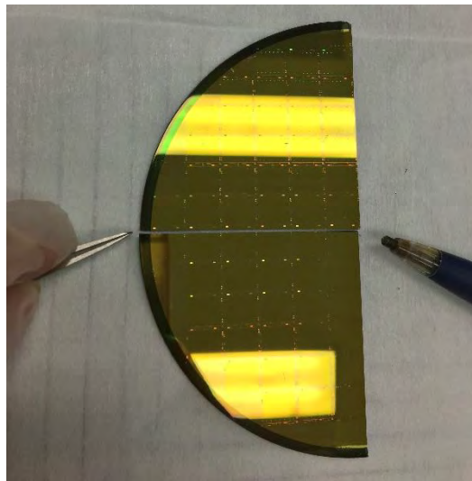
Figure 90. Two-point pressing method for wafer cutting without damaging the patterns.
