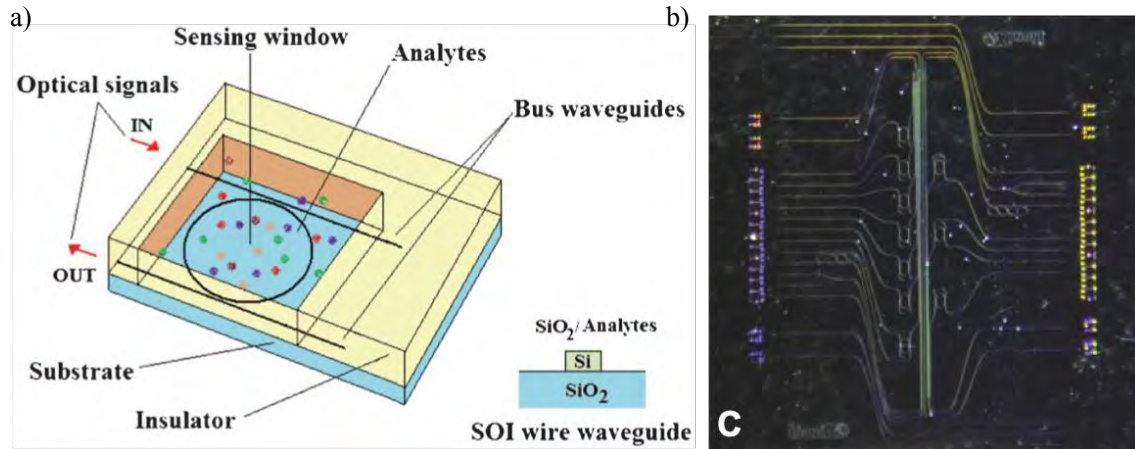
Figure 1. a) Schematic of a planar micro-resonator implemented in Silicon On Insulator technology [7]. b) Illustration of high density integration of micro ring resonators on a 1x1 cm chip using the TriPlex technology [8].
