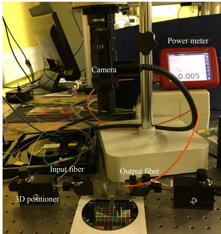
Figure 103. Improved optical bench for characterization of components.
