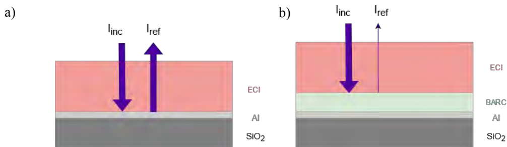
Figure 93. The incident light reflected on the substrate has nearly the same intensity as before, it will interfere the final resolution of the photoresist pattern (a), while using an anti-reflective coating (BARC) on the substrate will markedly minimised this effect, to keep the final pattern as neat as possible.
