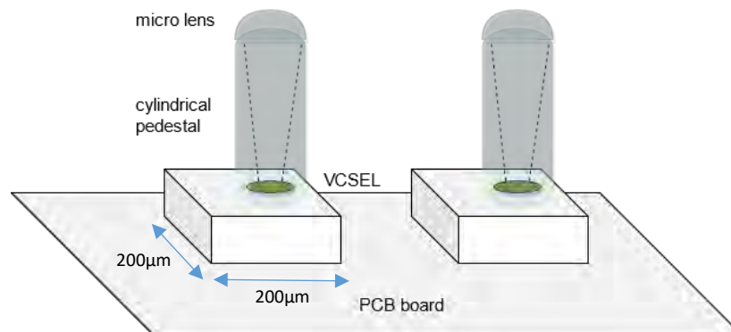
Figure 16. Schematic view of integrated polymer micro lens on VCSEL arrays
