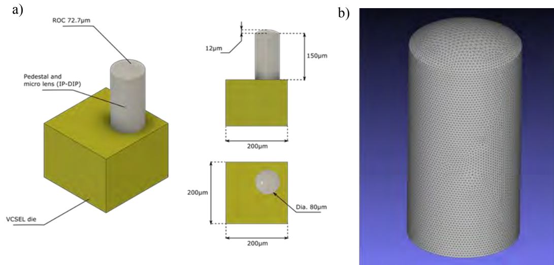
Figure 41. a). 3D CAD representation of the pedestal and micro lens over a dummy VCSEL die, highlighting the dimensions of the micro optical components compared to the VCSEL. b). Illustration of the STL file mesh to be used for the Nanoscribe 2PP equipment, comprising 22284 faces and 11414 vertices.
