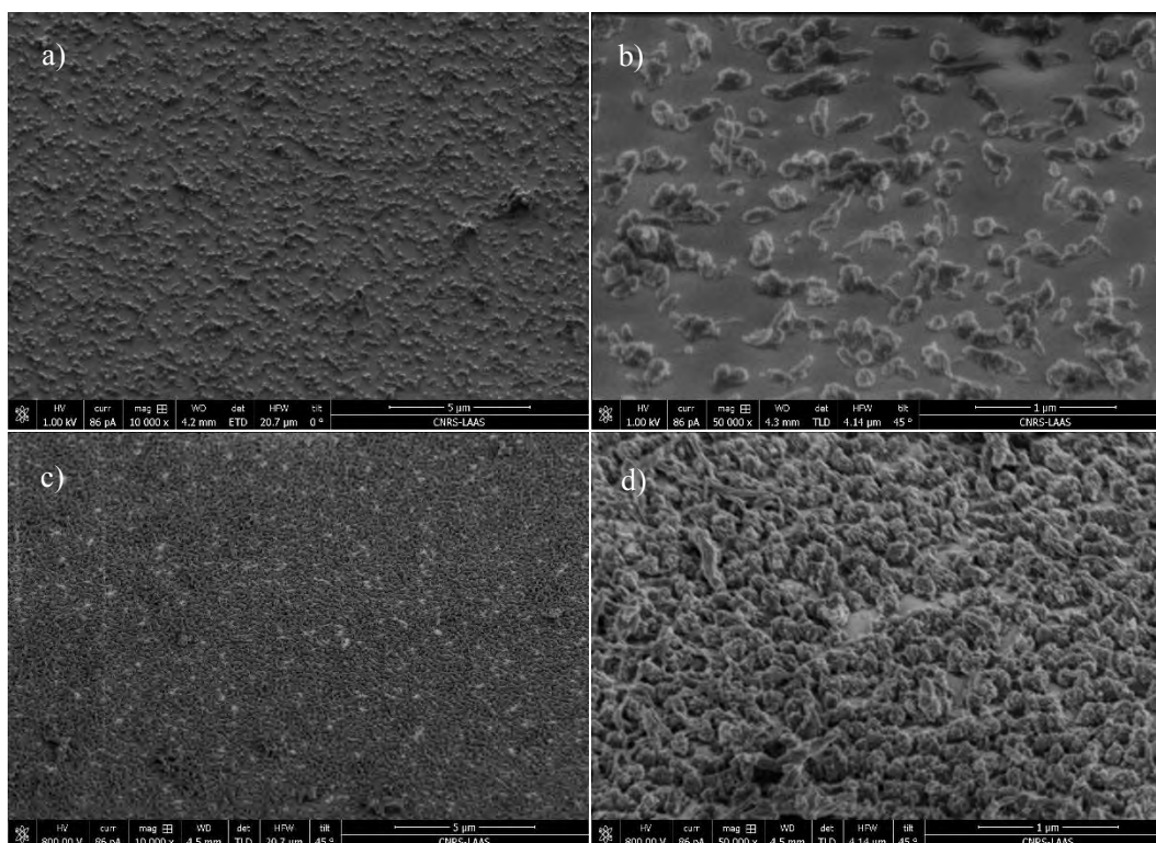
Figure 108. PANI coating produced in situ without (a,b) /with (c,d) an agitation of 80rpm.
