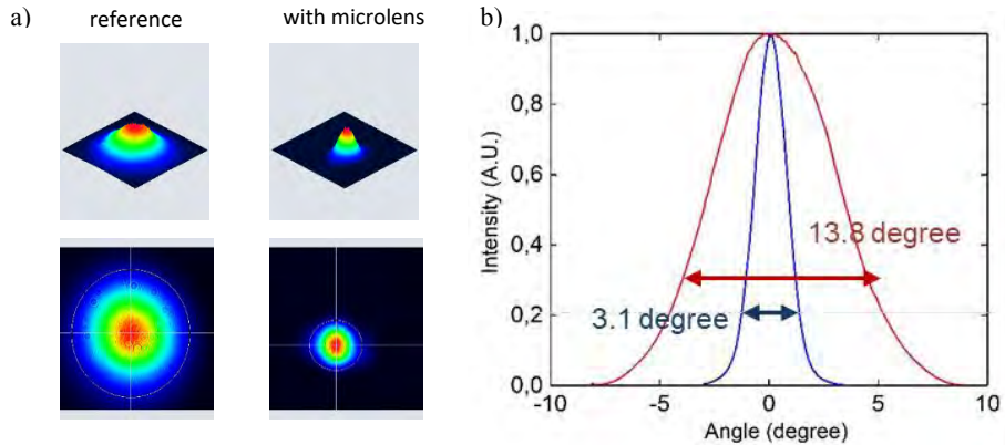
Figure 47. a) Beam profiles without and with microlens measured at 3mA. b) Divergence of VCSEL with or without micro lens fabricated by 2PP 3D printing.
