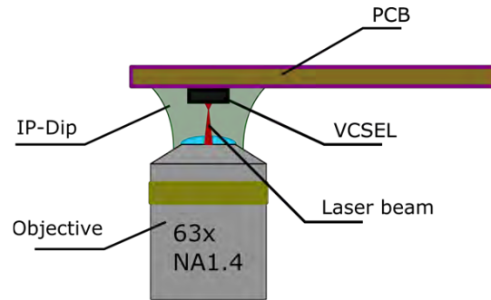
Figure 39. Working diagram of the 2-photon polymerization Nanoscribe 3D printing machine. The substrate (here a VCSEL mounted onto a PCB) is dipped into the photoresist which is in direct contact with the objective lens.
