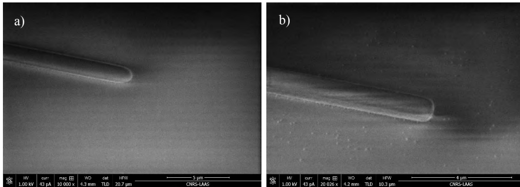
Figure 87. a) Waveguide exit port by regular photolithography. b) Waveguide exit port improved by GenISys design.
