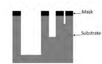
Figure 97. For the same material, the etch rate is lower on a smaller pattern during the plasma etching.
