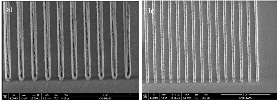
Figure 98. A 30s over etching time does not affect too much on the profile and duty cycle of pattern. a) Over etching time is 30s. b) Over etching time is 90s.
