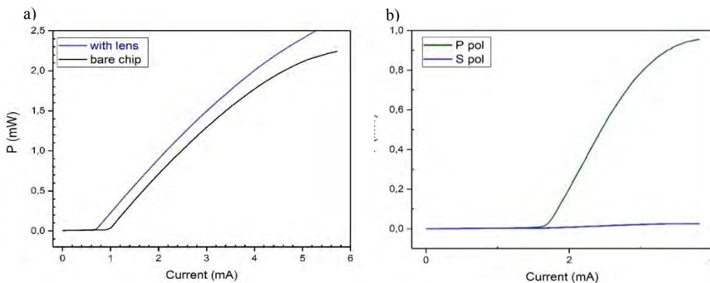
Figure 46. a) L(I) curve of VCSEL with and without 3D printed micro lens. b) Polarization-resolved L(I) curve of VCSEL with 2PP 3D printed micro lens.
