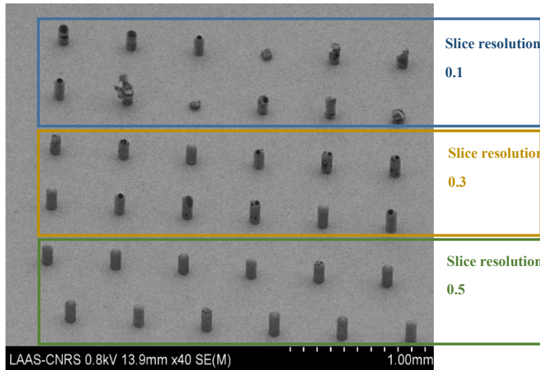
Figure 42. Calibration of exposure parameters for Nanoscribe writing.
