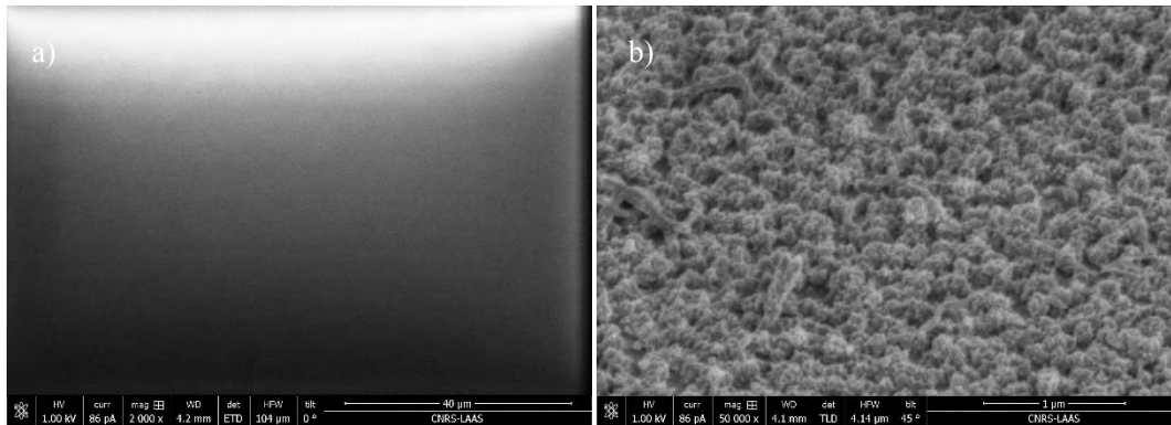
Figure 109. SU-8 surface without (a) / with (b) PANI coating.
