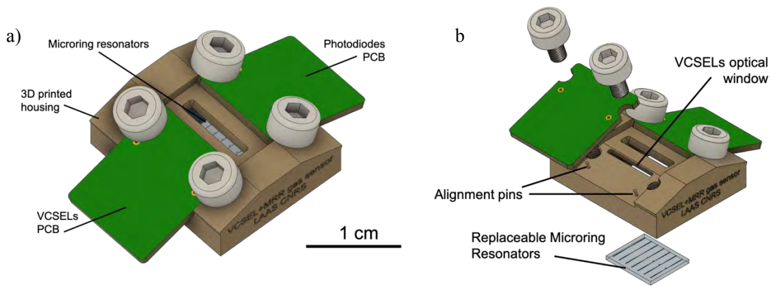
Figure 112. a) CAD rendering of the fully integrated optical gas sensor. b) Exploded view showing the alignment pins, the microring resonators chip, and the VCSEL optical window.
