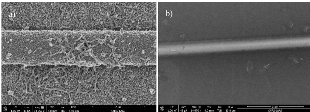
Figure 110. PANI coating on SU-8 waveguide which is deposited on the CYTOP lower cladding. a) PANI is coated by method in-situ. b) PANI is coated by method spin coating.
