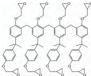
Figure 12. Chemical structure of SU-8.
