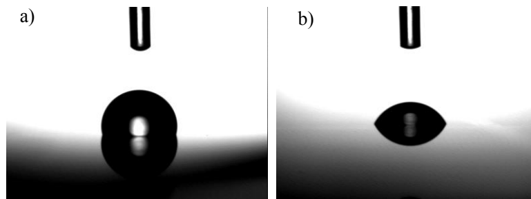
Figure 10. Contact angle of deionized water on the CYTOP surface. a) Water droplet before Al treatment. b) Water droplet after Al treatment.
