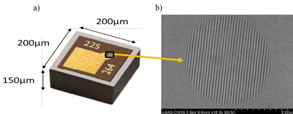
Figure 19. Single 850\text{nm} VCSEL chip with shallow etched grating at its surface (Trumpf).
