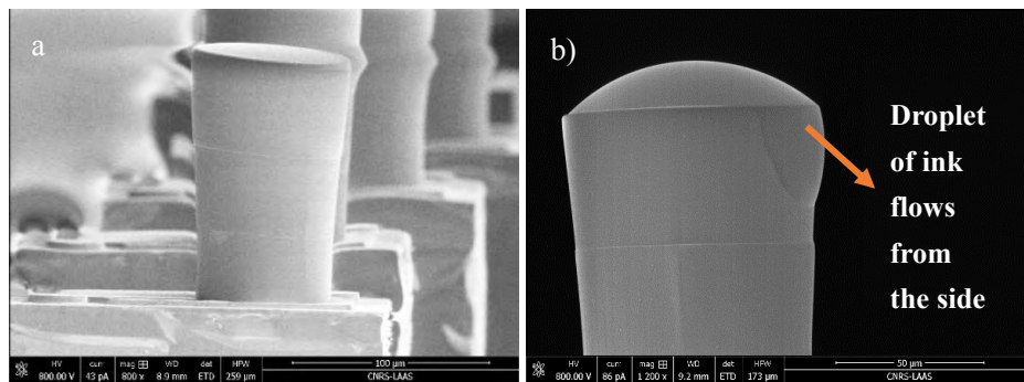
Figure 33. Inclined pedestal surface caused by the surface flatness defects under VCSEL chip during assembly.
