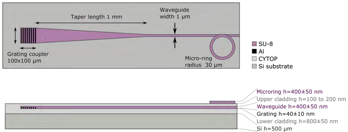
Figure 63. Top view and side view of the detection area of the microsystem.
