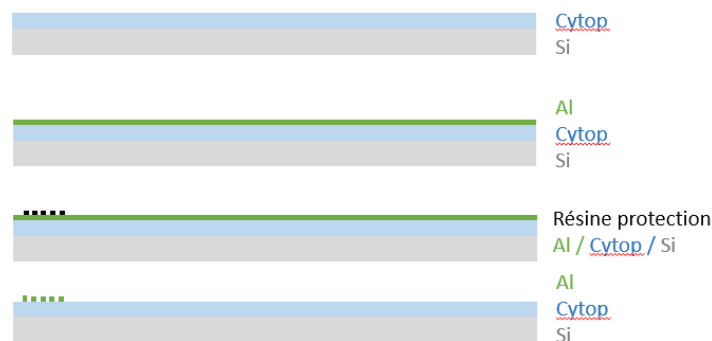
Figure 70. First approach adopted for manufacturing the aluminum grating couplers.
