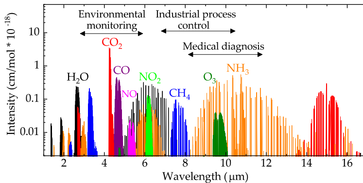
Figure 3. Absorption spectra of common gas molecules. [11]
