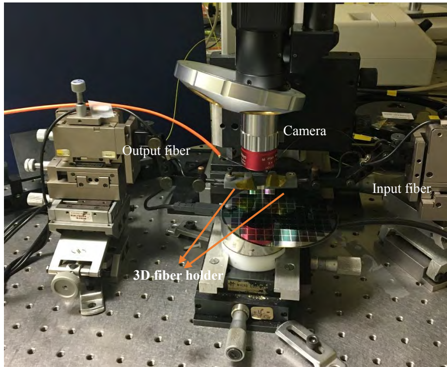
Figure 104. Upgraded optical bench for characterization of components.
