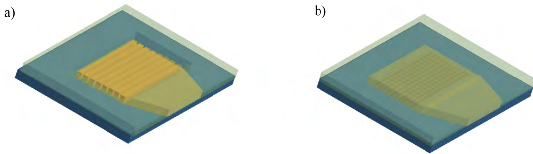
Figure 11. a) Polymer grating coupler, needs to etch the upper cladding leaving gratings unprotected. b) Al metallic grating coupler, where the grating is protected by both the waveguide and upper cladding.
