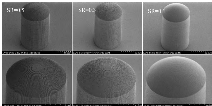
Figure 43. Micro pedestal and micro lens fabricated by 3D printing in three different slice resolutions.
