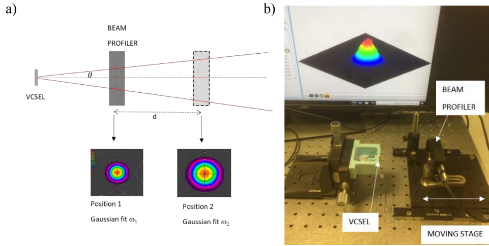
Figure 36. Measurement set-up of the beam divergence of single mode VCSELs
