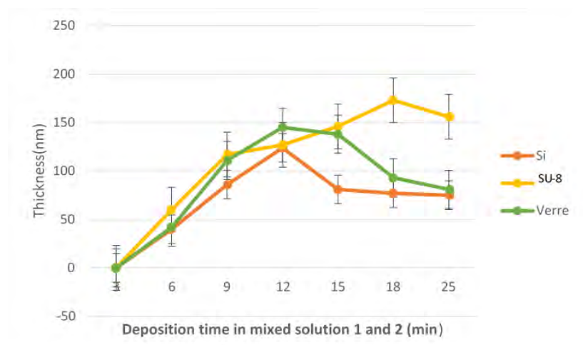
Figure 107. The evolution in the thickness of the PANI layer, deposited on Si, SU-8 and glass substrates over deposition time.
