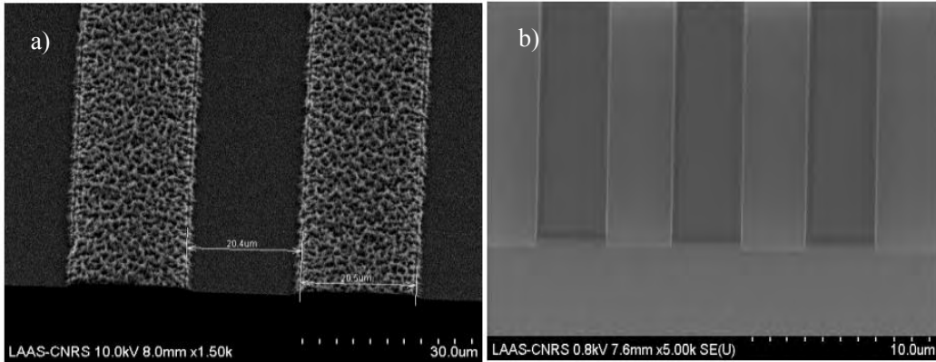
Figure 95. ECI patterns after plasma etching, a) with electrostatic clamping to the substrate holder, and b) with thermal conductive adhesive on the substrate holder. The roughness after etching is much lower in b).
