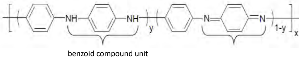
Figure 13. General structure of polyaniline. The term y denotes the degree of oxidation of the material.
