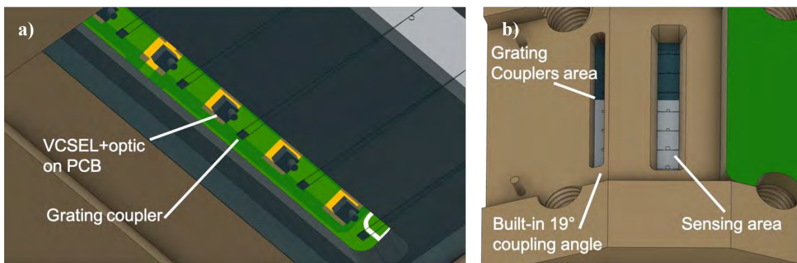
Figure 113. a) Detailed view of the collimated VCSEL matrix and the grating couplers observed from the bottom (through the Si substrate). b) Close-up view of the optical port showing the input grating couplers area, and the exposed sensing area with the microring resonators. A built-in slope of 19^\circ ensures the injection angle is guaranteed.
