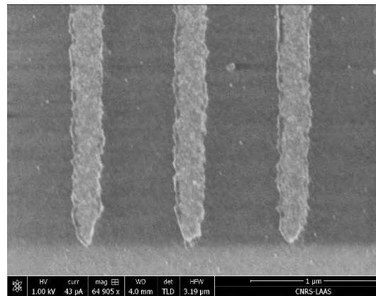
Figure 102. Al grating coupler fabricated by plasma etching and then stripped by UV-Ozone.
