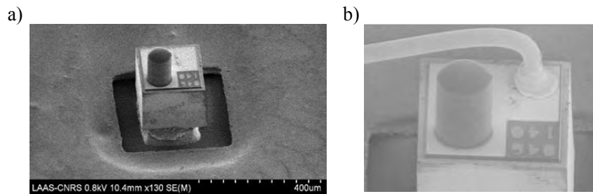
Figure 44. View of a VCSEL chip with a 3D printed lens in single step before (a) and after (b) wire bonding.
