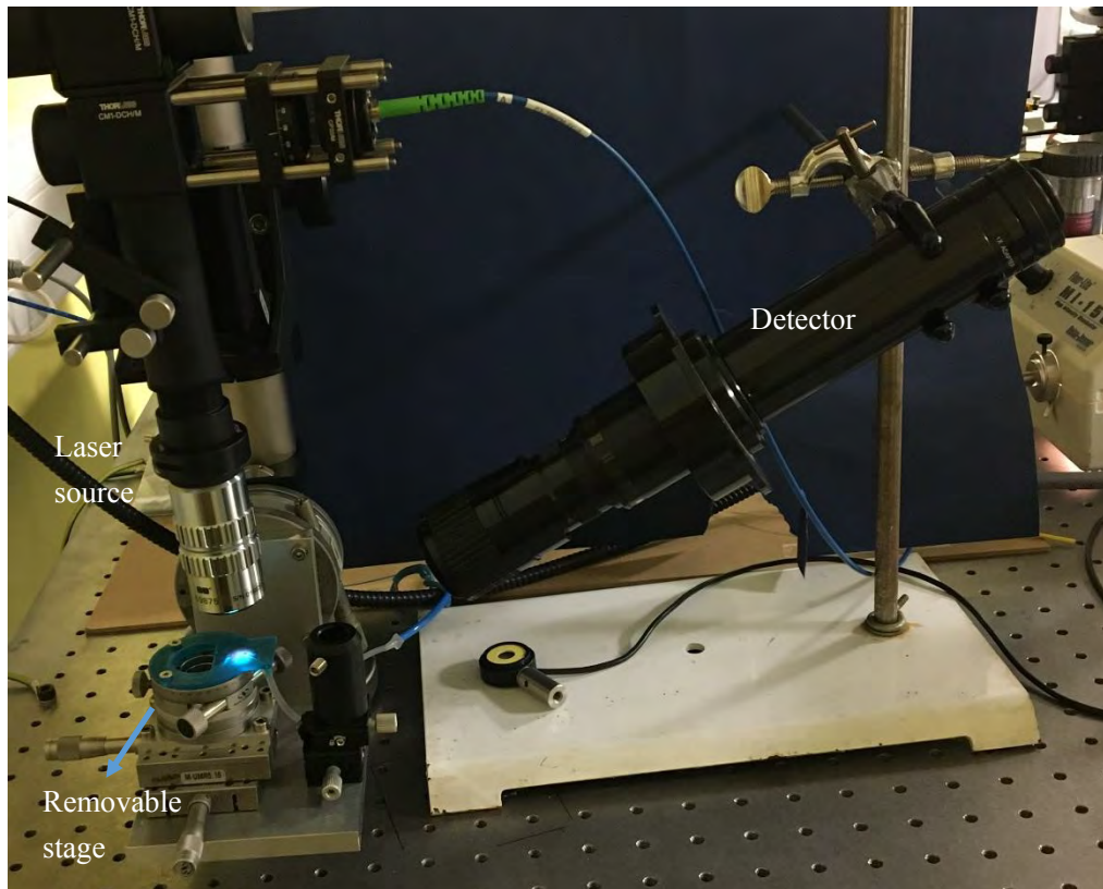
Figure 91. Optical bench for the characterization of the grating couplers.
