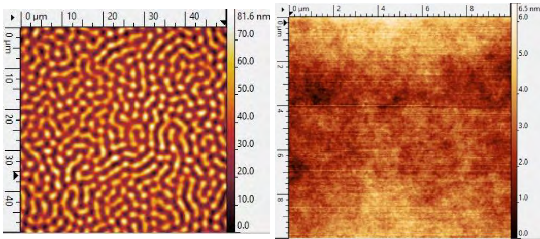
Figure 89. CYTOP surface before/after plasma oxygen etching.
