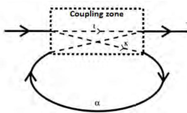
Figure 60. Energy coupling schematic between a waveguide and a lateral micro resonator.
