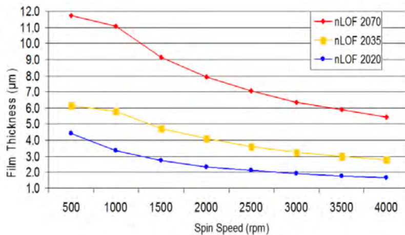
Figure 76. Coating thickness of nLOF 2000 series photoresists versus spin speed. [97]
