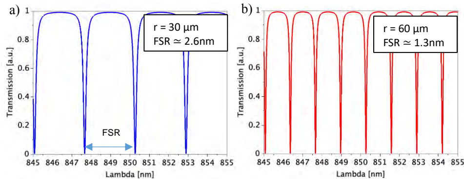
Figure 59. Quantized resonance modes of a conventional micro resonator besides a mono-mode waveguide
