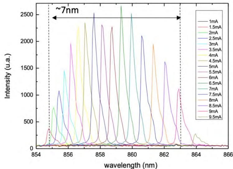
Figure 23. Measurement of the evolution of the emission spectrum of a typical single mode VCSEL chip according to the applied current.
