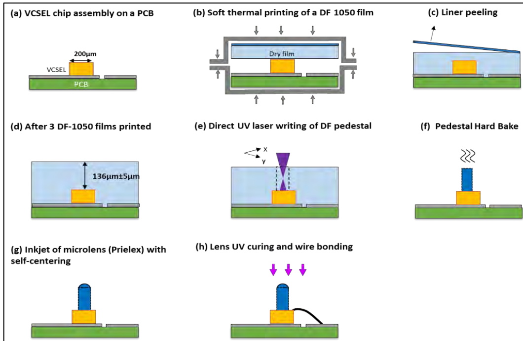
Figure 24. Procedure of VCSEL based micro-optical system fabrication. [82]
