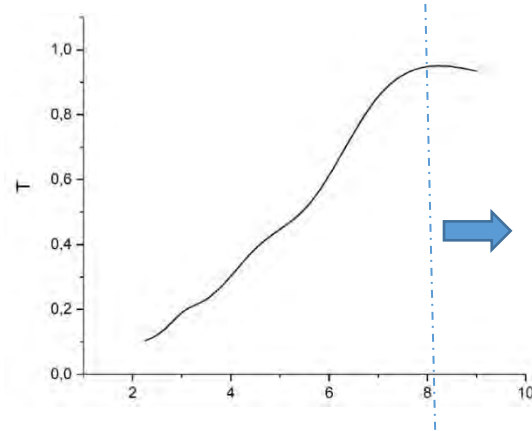
Figure 58. Taper guide transmission efficiency as a function of the length to width ratio.
