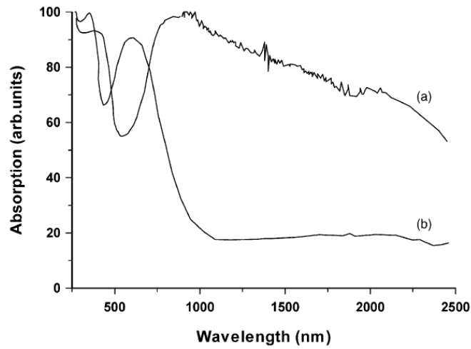
Figure 14. Absorption spectra of the polyaniline with (a) and without (b) gaseous ammonia. [57]
