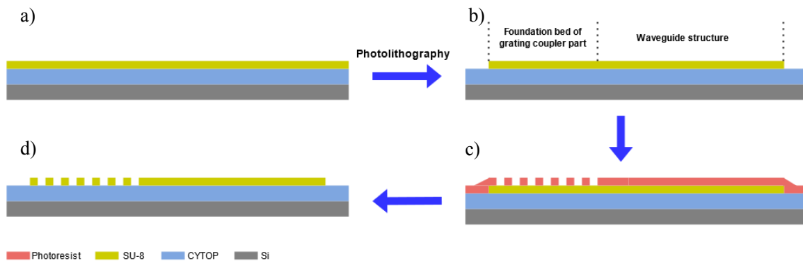
Figure 9. Schematic diagram of manufacturing process of SU-8 grating coupler by using stepper.
