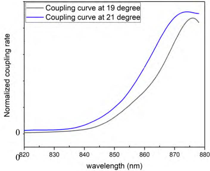
Figure 105. Normalized coupling rate of semi-manufactured wafer for the performance testing of upgraded optical bench.
