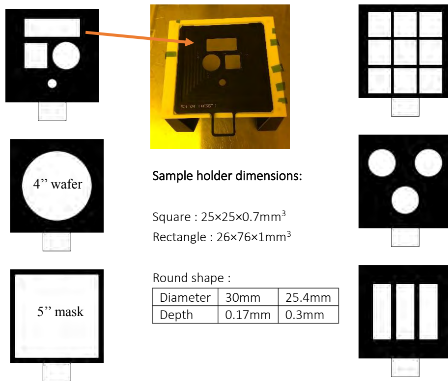
Figure 40. Different sample holders provided by Nanoscribe.
