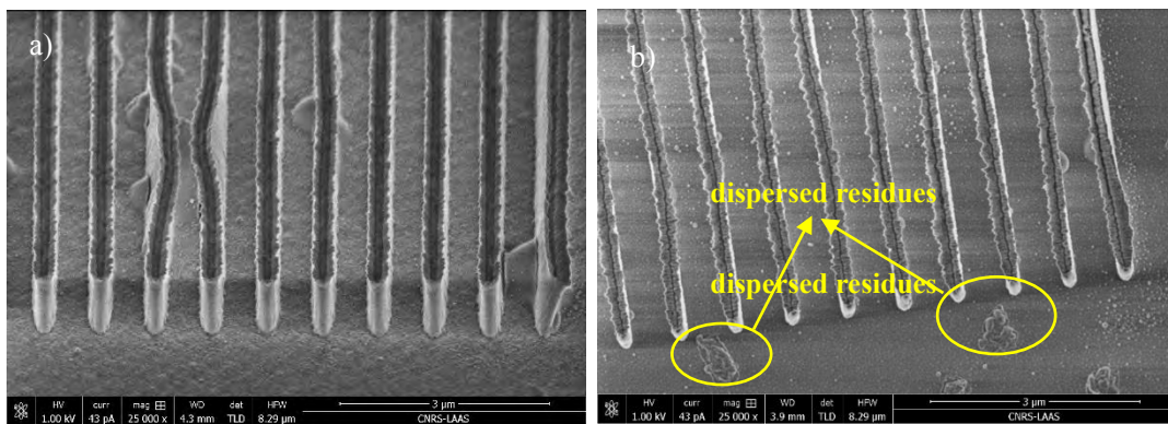
Figure 99. a) Protrusions appear next to grating coupler lines and pull the patterns to be distorted. b) A re-added plasma O 2 disperse the residues and contaminates the surface of sample.
