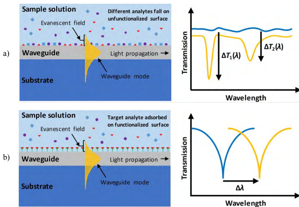
Figure 4. Two detection modes of microresonator sensors. [28]
