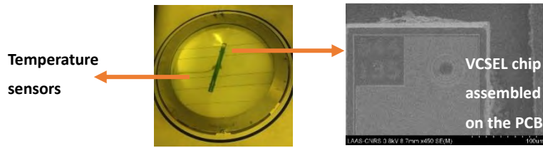
Figure 25. View of the VCSEL chip assembled on a PCB is sandwiched by two elastic films. A sufficient vacuum is used to imprint dry film on the non-planar sample. A temperature detector is used to control the temperature in the pressure chamber.
