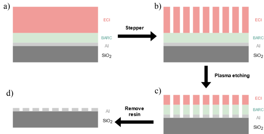
Figure 96. Process workflow for the fabrication of Al grating couplers over the SiO_2 lower cladding.
