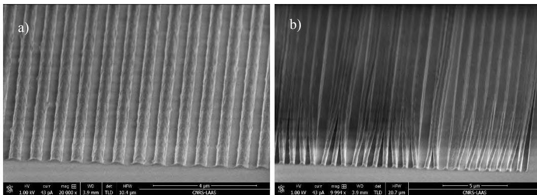
Figure 82. Underexposed (a) and overexposed (b) patterns of grating coupler after development.
