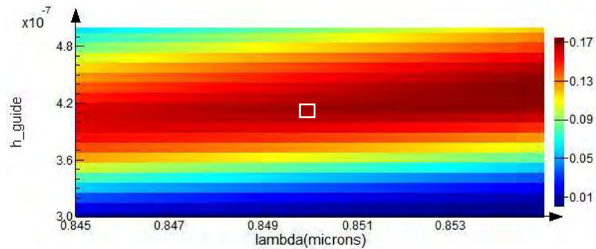
Figure 56. Coupling efficiency of the grating coupler versus waveguide thickness.
