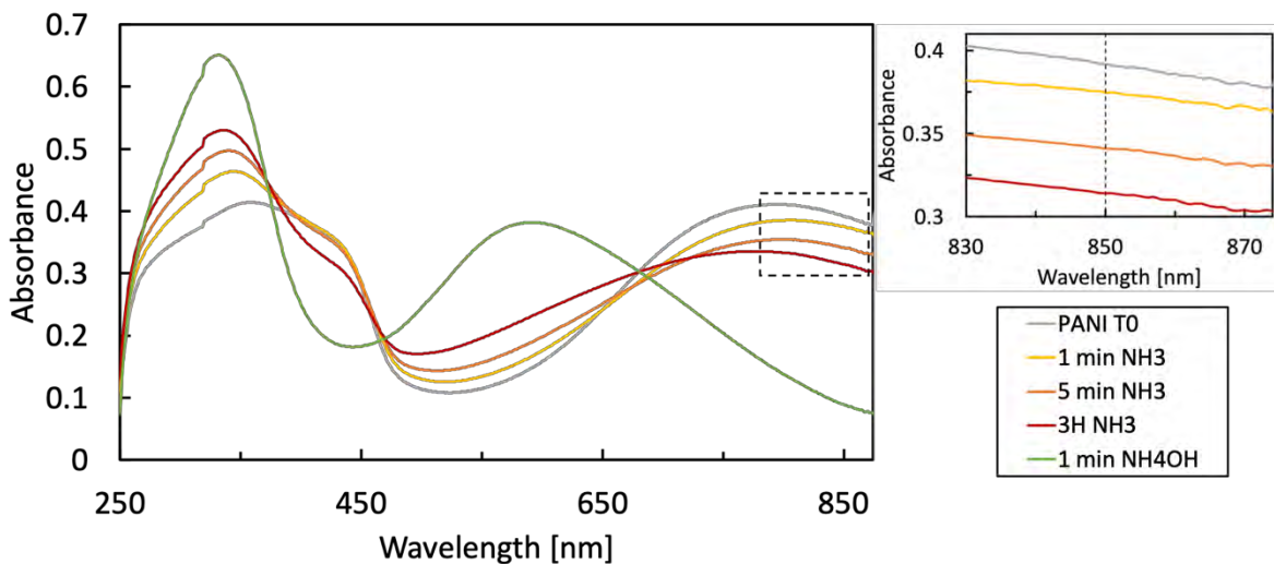
Figure 111. UV-VIS absorption spectra of PANI coated glass substrates upon different exposure times to NH 3 and NH 4 OH. Inset focuses on the absorbance variation around 850 nm.
