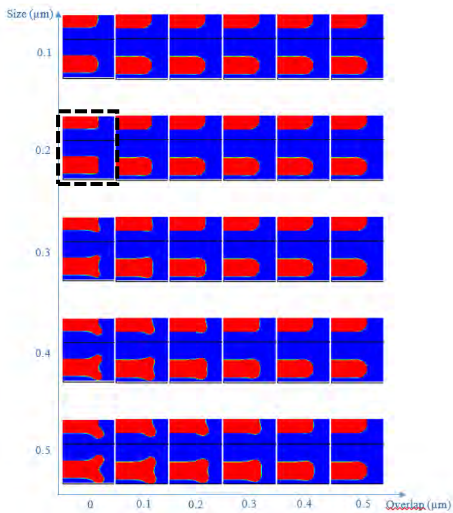
Figure 67. Simulation results obtained with GenISys for different additional square size and overlap with the waveguide extremity. The best configuration obtained at 0 \mu\text{m} overlap and 0.2 \mu\text{m} square size is highlighted.
