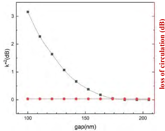
Figure 61. Energy coupling curve of a micro resonator system for different gaps.
