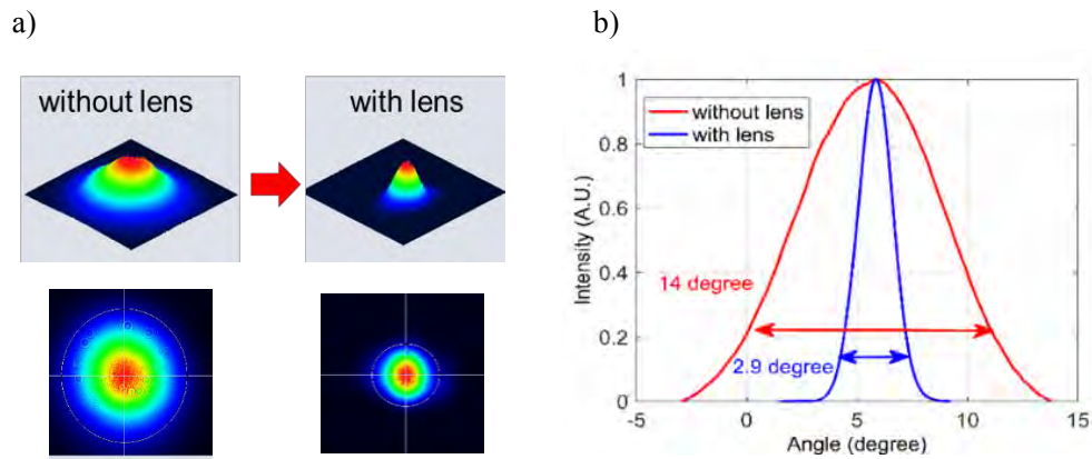
Figure 37. a) Intensity profiles measured with the beam profiler ( I=3\text{mA} ). b) Divergence of VCSEL with or without micro lens fabricated by inkjet writing.
