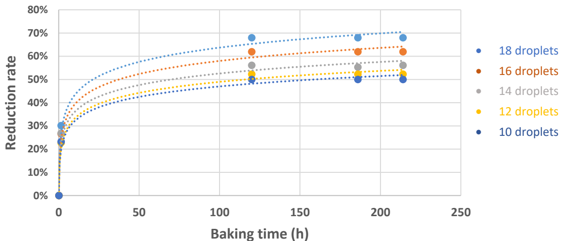
Figure 30. Measurement by confocal microscopy of the reduction rate of heights of micro lens as function of the baking time and number of jetted droplets.
