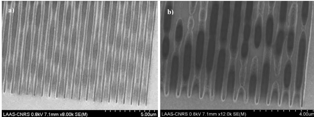
Figure 71. a) Wave shaped ECI stripes after photolithography. b) Uneven pattern of grating coupler after photolithography.
