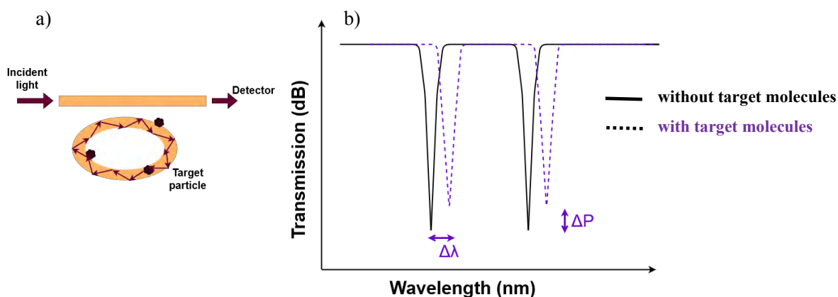
Figure 5. a) Specific wavelengths trapped by the micro resonator light path circulation. b) The presence of target molecules at the surface of the micro resonator will lead to a red shift in the resonance mode.
