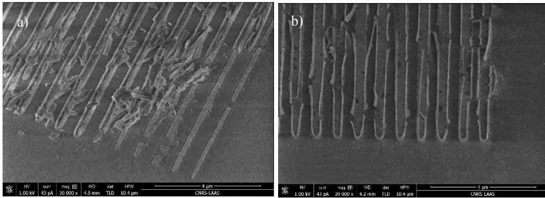
Figure 101. Illustration of the damages caused by (a) an ultrasonic bath with PG remover and (b) oxygen plasma on the nanometric features of the grating couplers.
