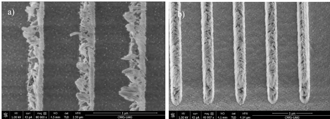
Figure 100. Grating coupler before stripping. a) A deionized water flow is used to avoid residue bumps. b) A chaining oxygen plasma without interruption of vacuum is used to avoid the formation of residue.
