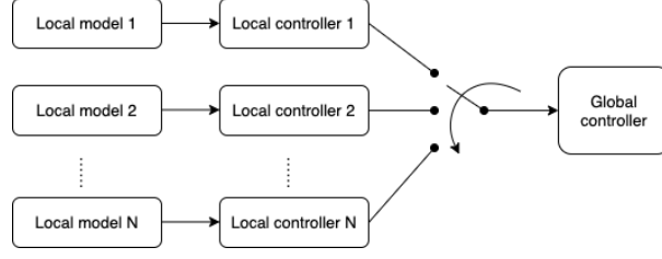
Figure 3.2: Local controller structure of multiple model method
