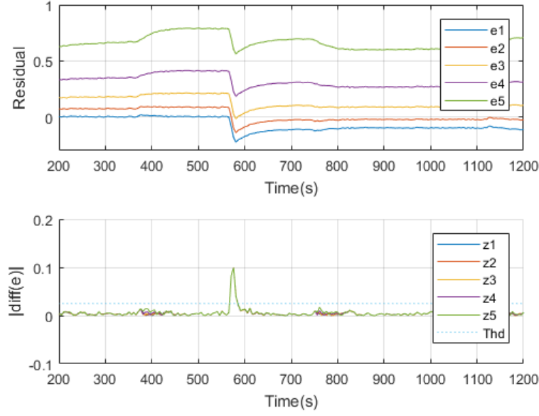
Figure 5.6: FDI process using interval unscented Kalman filters
