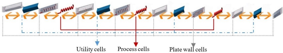
Figure 4.4: Internal description of one computing unit and convective heat exchange
