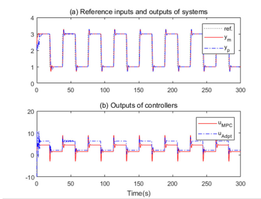
Figure 6.6: Simulation result of multiple adaptive models under normal condition
