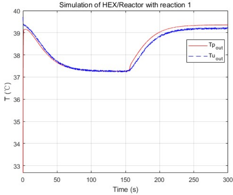
Figure 4.15: Simulated temperature profiles for experiment 1 (reaction was introduced at 150s)
