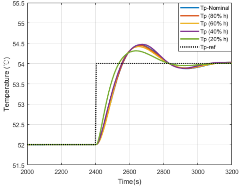
Figure 5.5: Performances of controller banks under the same reference T_{p-ref} after tuning.
