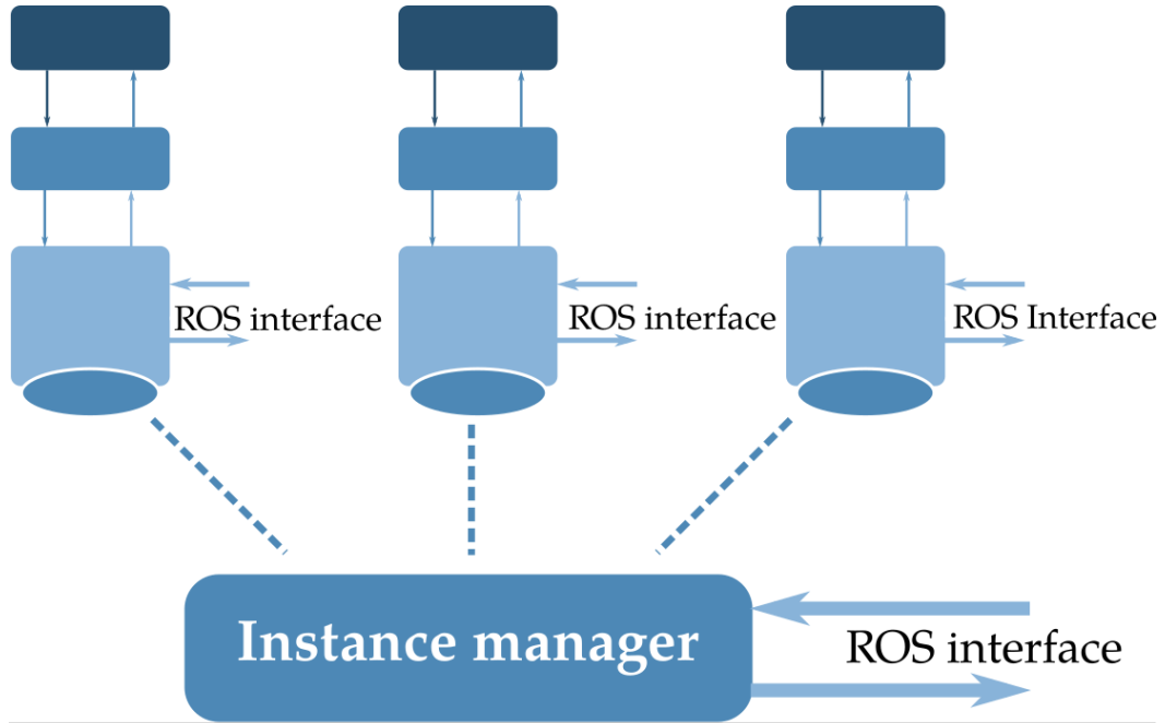
Figure 2.7: The software architecture of Ontologienius to manage multiple Knowledge Bases in the form of an ontology. An instance manager makes the link between each instance (see Figure 2.4) and has a direct access to each semantic graph to propose queries.
