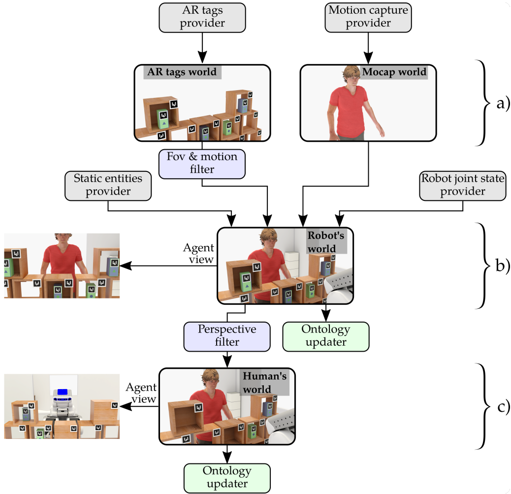
Figure 9.6: The world cascading structure of the geometrical situation assessment system. The two worlds at the top (a) are build from the perception systems and filtered. The world of the middle (b) merges the different perception information and computes symbolic facts on it. The world at the bottom (c) is the estimation of the human world representation and is computed from perspective-taking in the robot's world. Like for the world of the middle, symbolic facts are computed and sent to the semantic knowledge base.
