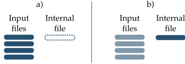
Figure 2.5: a) In the case where no internal file already exists, the input files are considered as the default Knowledge Base of the agent b) In the case where an internal file exists for a given agent, this means that the robot is already interacting with this agent. In the latter case, the input files are not taken into account and the previously estimated Knowledge Base of the agent is loaded. If the current Knowledge Base represents that the robot’s one, the robot simply restarts with its previous knowledge base.
