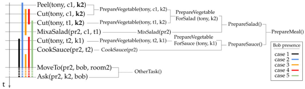
Figure 6.9: The hierarchical execution trace to prepare the meal and a trace for another subsequent high-level task, organized according to a timeline. In the current instant, PR2 is asking Bob, a second human, for knife k2 . The five cases are represented by five colors at the left of the tasks and correspond to tasks seen by Bob, the human spectator. In case 1, Bob did not see any tasks involved in the preparation of the salad but was present during the sauce preparation. In the second case, he observed all the activities.
