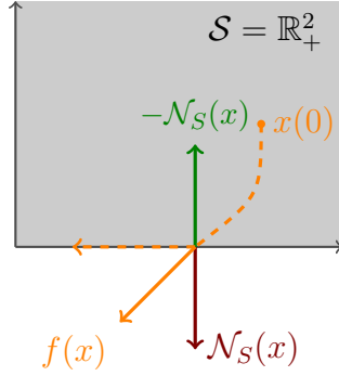
Figure 2.1: State trajectories in constrained system with S = \mathbb{R}_+^2 .
