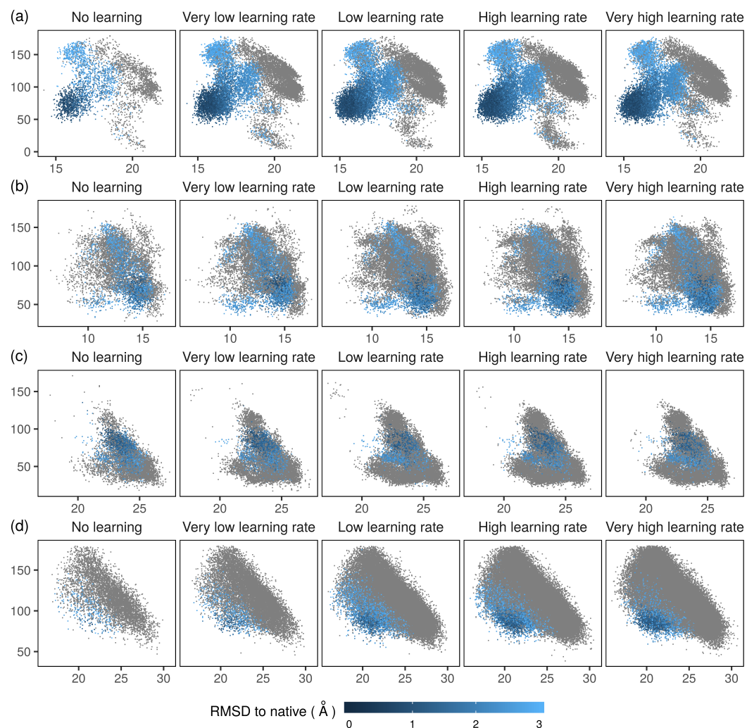
Figure 3.18. Two-dimensional projections of the sampled loops at different levels of reinforcement learning. Each point represents a loop. Points are colored according to the distance to native of the corresponding loop, or in grey if their RMSD to native is above 3 Å. The x-axis gives the first projection descriptor d_1 (in Å), while the y-axis gives the second projection descriptor, d_2 (°). (a) Loop 21, (b) Loop 26, (c) Loop 40, (d) Loop 68.
