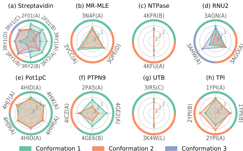
Figure 4.2. Lowest RMSD to each known stable conformations among sampled states, for each scaffold. RMSDs are calculated on the heavy atoms of the backbone. Scaffolds are distributed around the disk and their names indicated outside the disk. The outer circle is colored according to the conformation present in the X-Ray structure the scaffold originated from. The outer circle corresponds to a RMSD of 0 Å, while the center corresponds to RMSDs of 4 Å and above: a larger colored area indicates that the corresponding stable conformation is found with greater accuracy in the sampled ensemble.
