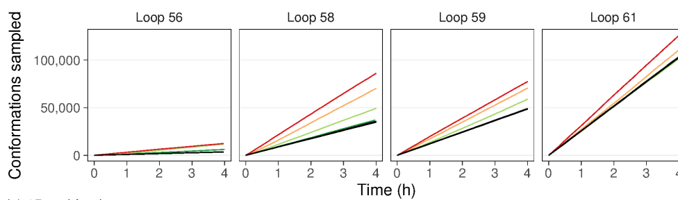
(c) 15-residue loops
