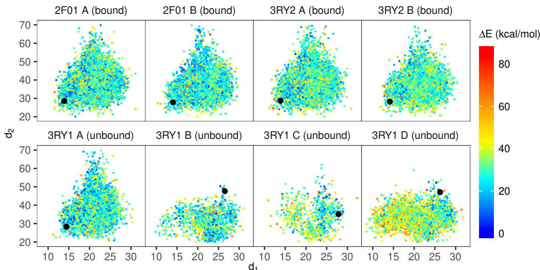
Figure 3.12. 2D projections of conformations sampled using D1SGRO for a loop in the streptavidin protein, from eight starting X-ray protein structures. The first dimension, d_1 (x-axis), is the distance (Å) between an atom located in the middle of the loop and a fixed atom in the protein. The second dimension, d_2 (y-axis), is the angle (degrees) formed by three atoms: an atom at approximately one quarter, one half, and three quarters of the way down of the loop. The conformations from the crystallographic structures are shown in black. For each system, the loop with the lowest energy was identified and each conformation was then colored according to the difference between its energy and this lowest energy.
