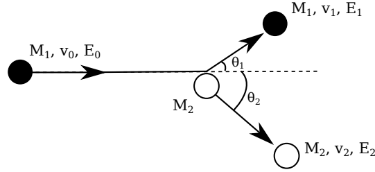
Figure 3.1: Schematic view of the situation modeled by the BCA in the laboratory system. The projectile atom is depicted by the black circle and the target atom by the white circle. The signification of all the letters and symbols are given in the text.
