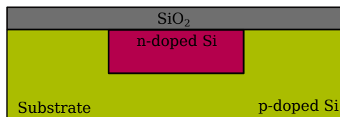
Figure 1.7: Cross-section view of a CMOS photodiode.
