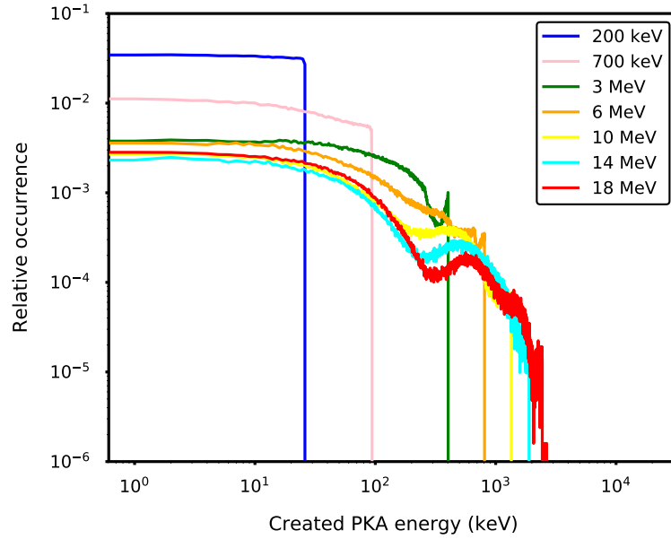
Figure 6.12: Relative occurrence of strictly Si PKAs ( Z = 10 ) created in \text{Si}_{0.8}\text{Ge}_{0.2} as a function of their energy following collision with a neutron, for neutrons energy ranging from 200 keV to 18 MeV. For each neutron energy, 10^6 simulations have been launched.
