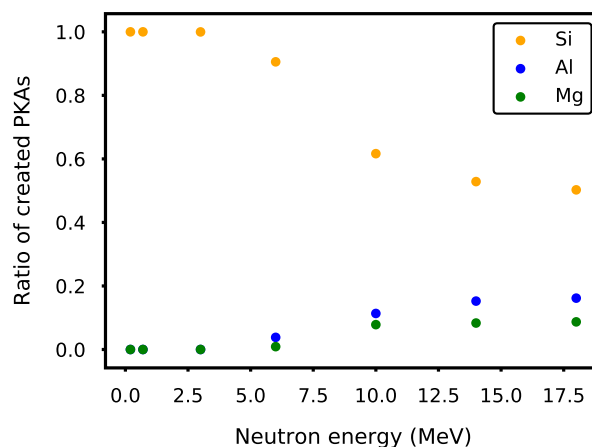
Figure 6.2: Ratio of PKAs created in Si as a function of their type after collisions with neutrons of energies ranging from 200 keV to 18 MeV. For each neutron energy, 10^6 simulations have been launched. Only the heavy ( Z > 10 ) spallation products are shown here. The data points of the created protons following spallation reactions would follow the one the Al PKAs, and the one of the alpha particles the one of the Mg PKAs.
