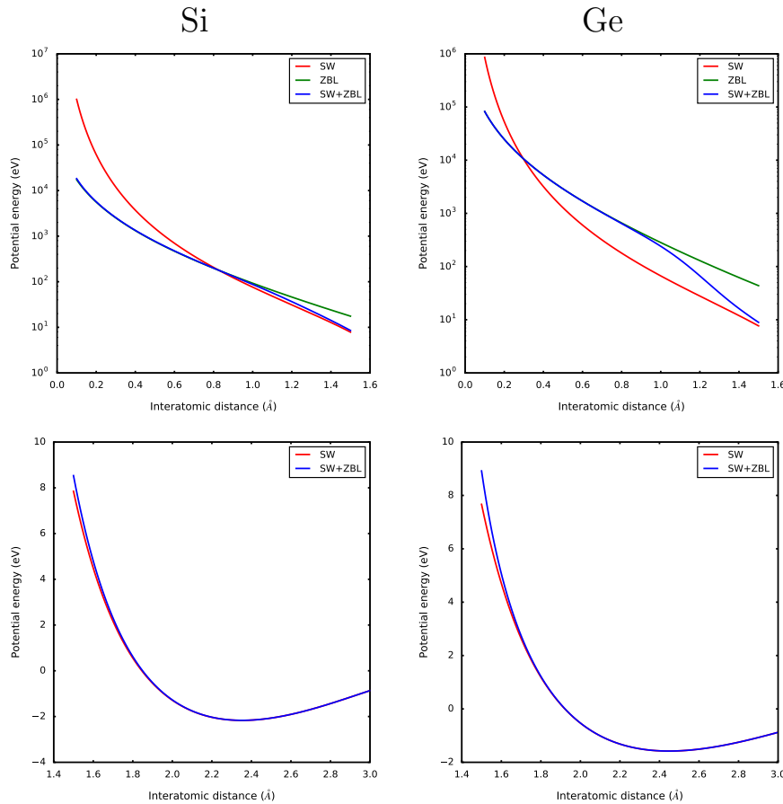
Figure 3.7: Short-range (top) and long-range (bottom) two-body SW, ZBL (top only) and SW+ZBL potentials for Si (left) and Ge (right).
