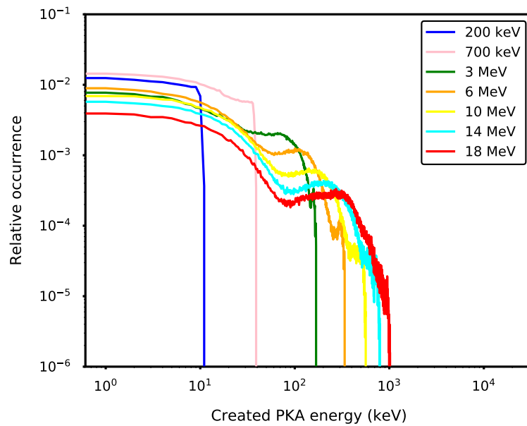
Figure 6.13: Relative occurrence of strictly Ge PKAs ( Z = 32 ) created in \text{Si}_{0.8}\text{Ge}_{0.2} as a function of their energy following collision with a neutron, for neutrons energy ranging from 200 keV to 18 MeV. For each neutron energy, 10^6 simulations have been launched.
