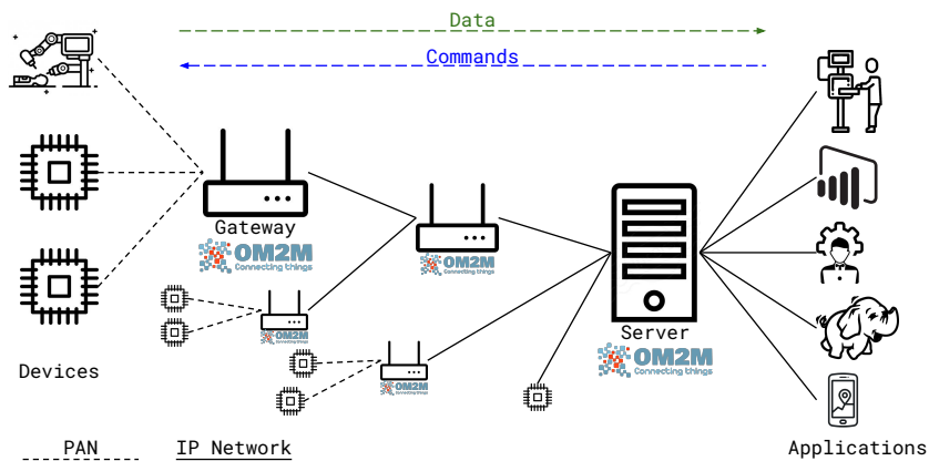
Figure 2.2: OM2M functional architecture
