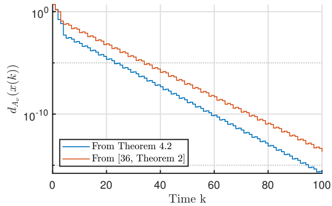
Figure 4.3: Evolution of the distance to the attractor d_{A_\nu}(x(k)) for Example 2 with control law (4.11) and the control law from [36, Theorem 2].
