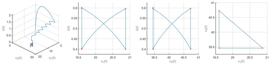
Figure 6.5: On the last three columns, from left to right, are figures illustrating the limit cycle where the system converges. On the first figure on the left is represented the global view of the state evolution in a phase space. In each column, the blue line represents the evolution of the state while the red crosses represent the point of the state limit cycle associated to the cycle \nu_0 (Example 3).
