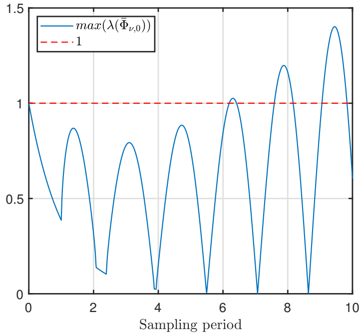
Figure 6.2: Illustration of the max absolute characteristic multiplier of the monodromy matrix for the cycle \nu_4 = [3 \ 3 \ 2 \ 1] (Example 1).
