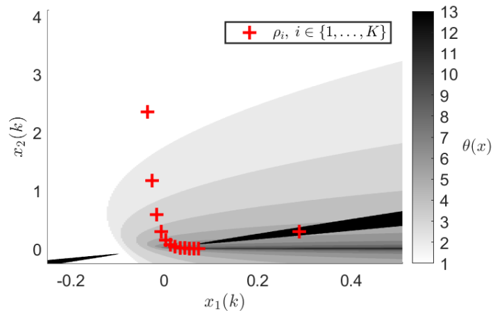
Figure 4.4: State-space partition \theta(x) (Example 3).
