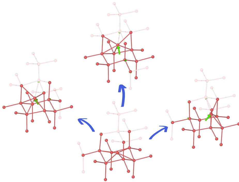
Figure 5.18: Hexagonal to hexagonal inside . The interstitial atom moves from one hexagon to another, within the same diamond unit cell structure.
