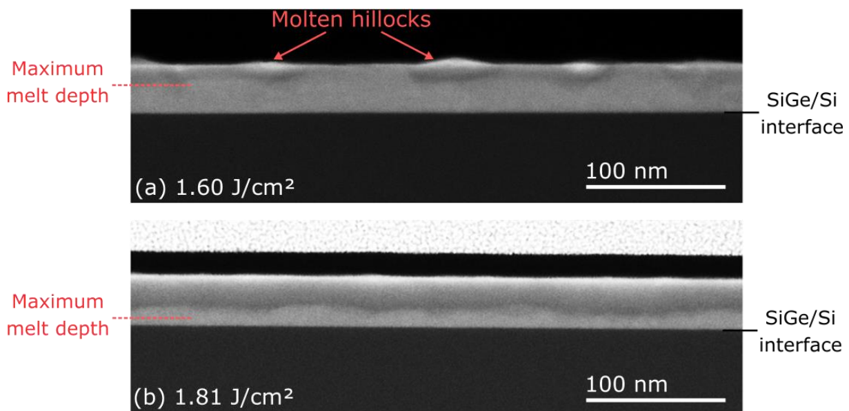
Figure IV - 4. STEM-HAADF micrographs of 30 nm \text{Si}_{0.6}\text{Ge}_{0.4} samples annealed at 1.60 \text{ J/cm}^2 (a), and 1.81 \text{ J/cm}^2 (b). The contrast is related to the chemical composition: Ge-rich areas are brighter. This enables to distinguish limits between un-melted areas and melted areas where segregation occurred.
