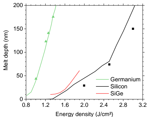
Figure I - 37. Melt depths in Si, \text{Si}_{0.5}\text{Ge}_{0.5} and Ge extracted from experimental (symbols) and simulations results (lines) after NLA with \lambda=308 nm and pulse duration at 160 ns [89–92].
