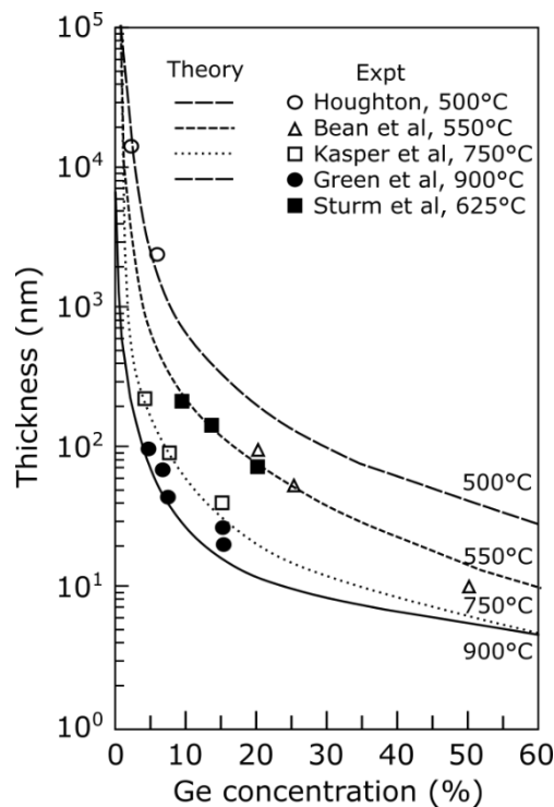
Figure I - 8. Critical thickness of \text{Si}_{1-x}\text{Ge}_x layers as a function of Ge content x , at various growth temperatures, from [16]. The critical thickness at a given content increases for lower growth temperatures.
