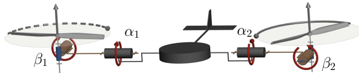
Figure 3.2 – Conceptual 3D kinematic representation of a generic birotor design with wing-tail stabilization.
