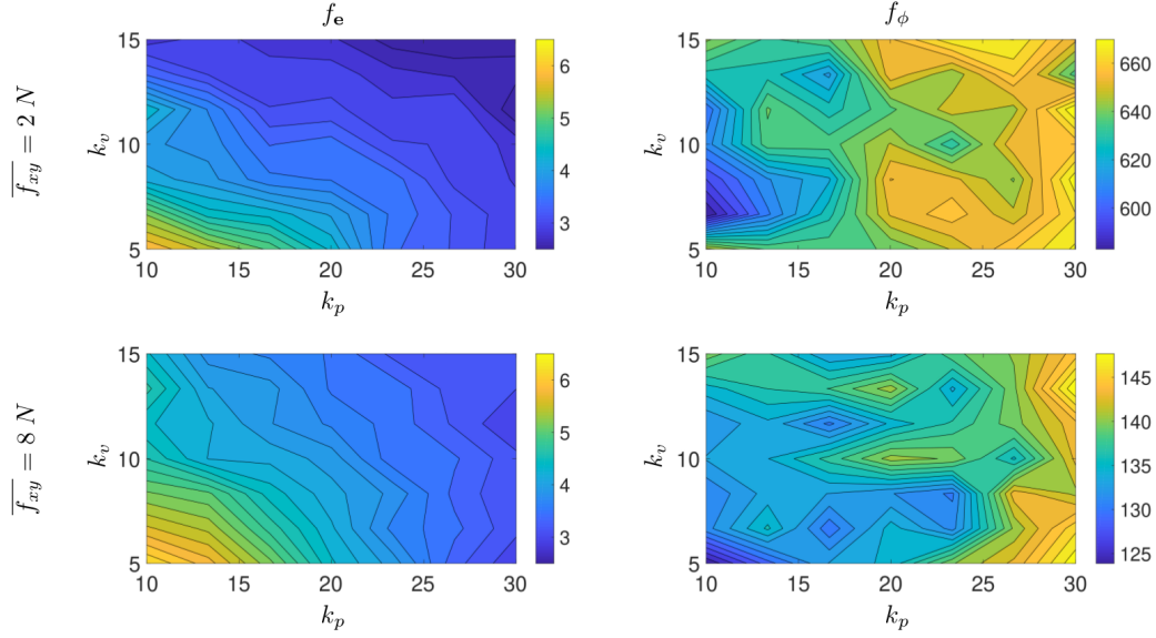
Figure 6.3 – Contour plots of f_e(k_p, k_v) and f_\phi(k_p, k_v) for two different values of \overline{f_{xy}} computed via simulation on a discretization of the ranges \mathfrak{D}_{k_p}^{(1)}, \mathfrak{D}_{k_v}^{(1)} .
