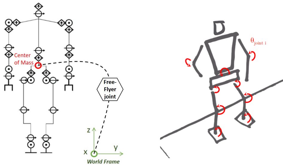
Figure 1.2: Kinematic structure of TALOS Scherrer [1]
