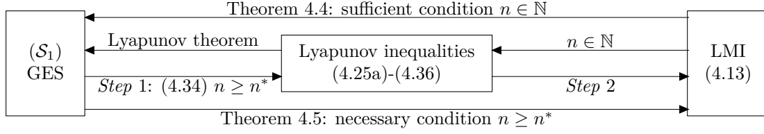
Figure 4.10: Necessary and sufficient LMI condition for stability.
