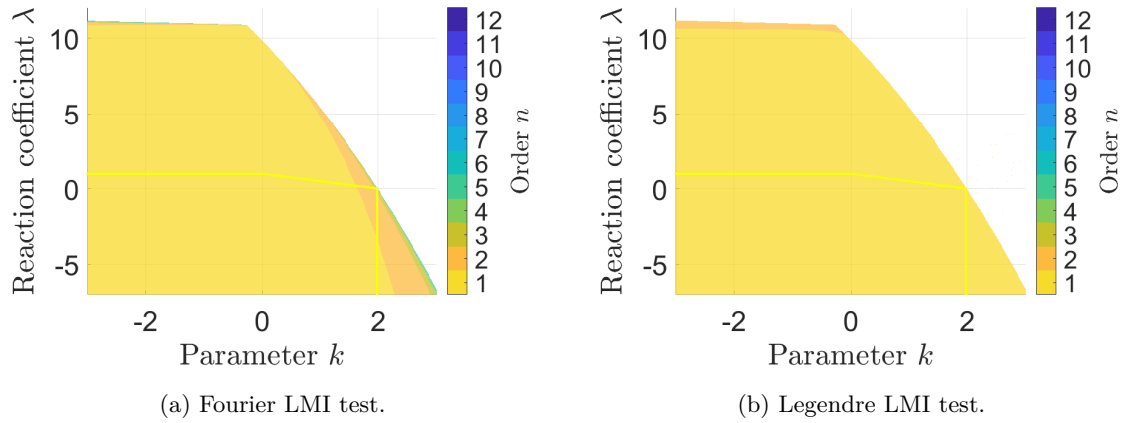
Figure 6.3: Allowable sets of stability given by Theorems 6.4 and 6.5 with respect to the orders n \in \{1, \dots, 12\} and for various pairs of parameters (\lambda, k) .
