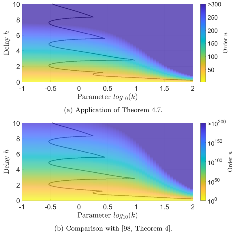
Figure 4.13: Estimation of the order n for the necessity of positivity conditions.
