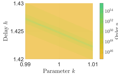
(b) Example 2 for (k, h) \simeq (1, 1.425) .
