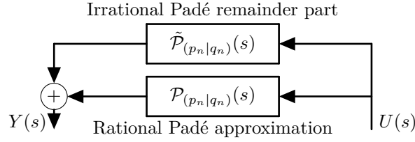
Figure 3.1: Padé modelling of the transport transfer function H(s) = e^{-hs} .
