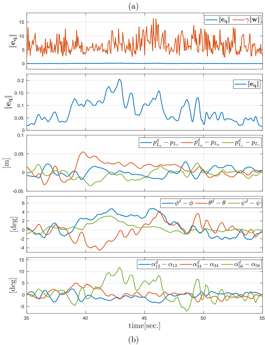
Figure 6.11: (a) Verification of conditions (5.28)-(5.30) for experiment 2). (b) Tracking error for experiment 2)
