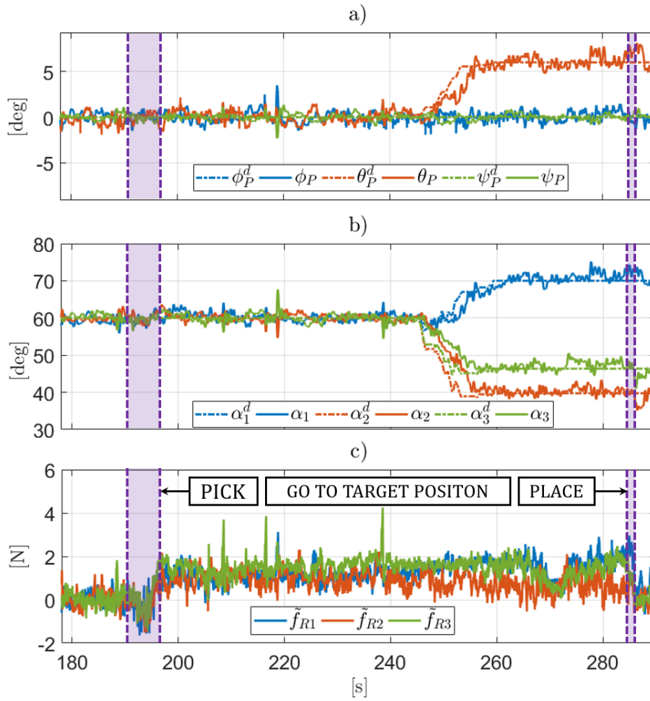
Figure 7.4: Tracking of the desired trajectory for the attitude and \alpha angles and comparing with the extra thrust.
