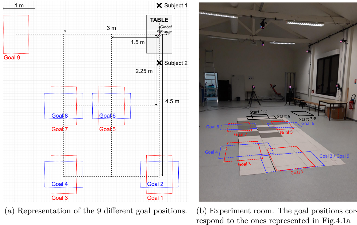
Figure 4.1: Experimental setup
