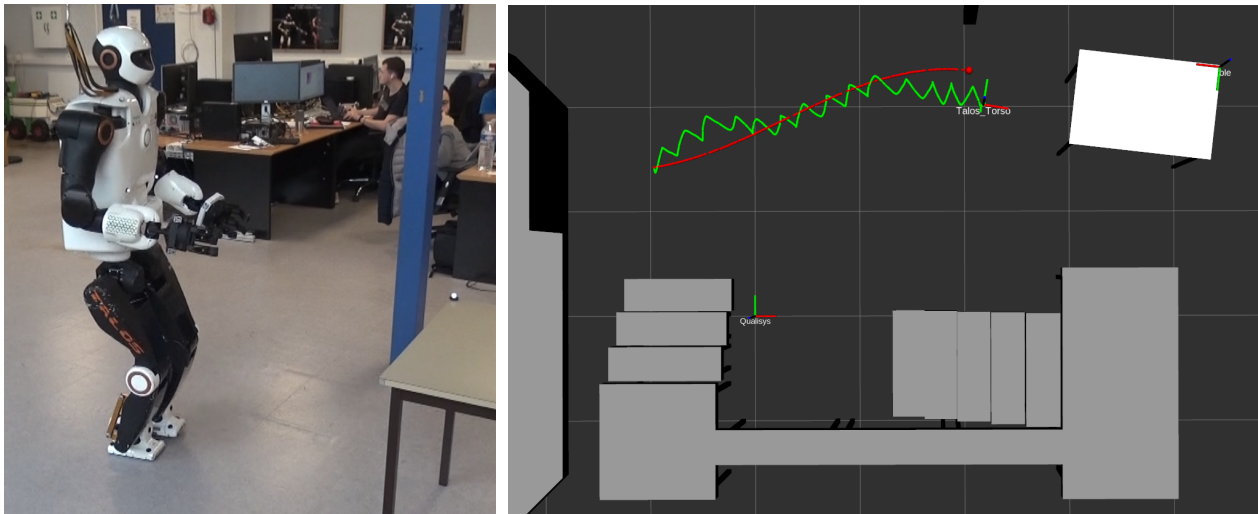
(a) TALOS robot walking toward a table (b) Visualization of the trajectory of the CoM of the robot (in green) during one experiment aiming to follow a clothoid trajectory (in red), in the upper right corner is the table (in white)
