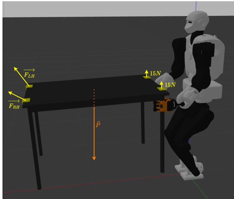
Figure 5.20: Simulation on Gazebo where a TALOS humanoid robot holds a 20.7 kg table. \vec{P} is the weight of the table. F_{RH} and F_{LH} are the forces applied on the left yellow spots to simulate the forces applied on the table by the hands of the human partner.
