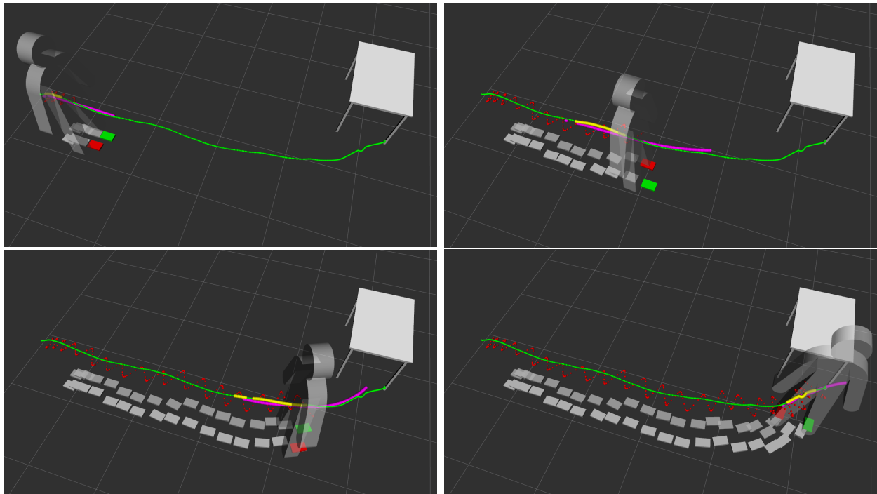
Figure 3.8: The robot CoM (in red ) and footsteps (past steps in grey , current support foot in red and future support foot in green ) are generated from the current optimal solution given by the prediction process (in purple ) which takes the recent past trajectory of the human (in yellow ) as an input. Here, the prediction parameters are N_0 = 50 and N_{OC} = 100 .
