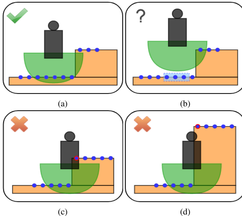
Figure 3.8: Approximated validity conditions: (Green) robot range of motion, (blue) height map. Configuration (a) is valid, (b) is valid with \mathcal{C} and \tilde{\mathcal{R}} but invalid with \tilde{\mathcal{R}}^* where none of the high-lighted blue dots are reachable, (c) and (d) are valid with \tilde{\mathcal{R}}^* but in collision.
