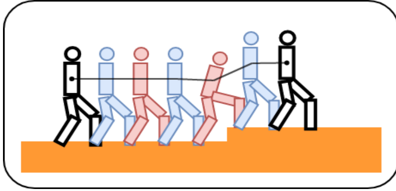
Figure 4.1: Given a guide path, our contact planner generates key configurations in contact along it.
