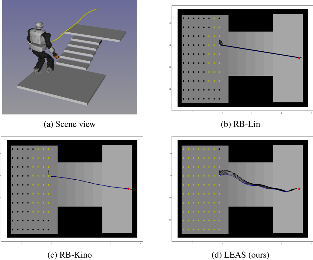
Figure 3.14: Comparison on stairs where dots represent initial states from where the SM generates a valid (yellow) or invalid (black) guide path up to the goal (red). The height map is represented by the grey shades from dark to bright, that are lower and higher heights respectively. We illustrate for each SM one trajectory where the black arrows represent the robot orientation along the guide.
