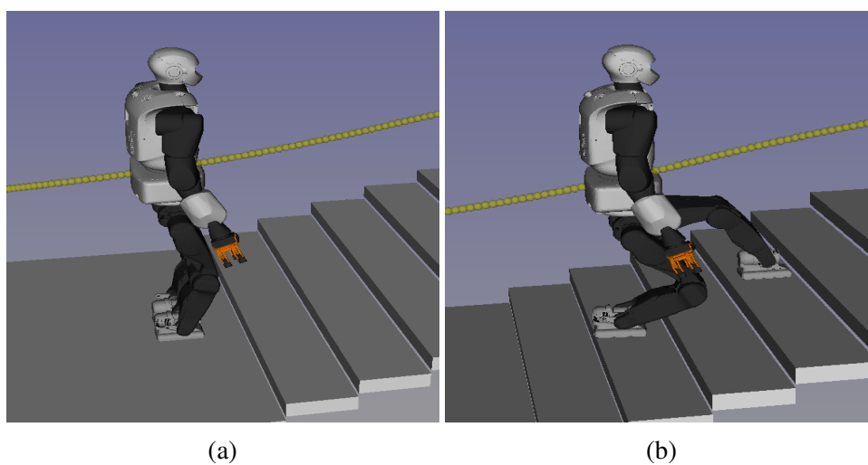
Figure 4.16: Scenario C2: Difficult root configuration on the guide for SBCP: (a) too high where the robot has its legs in extension and can not reach the next root position, (b) too low where the robot climbs the stairs crouched.
