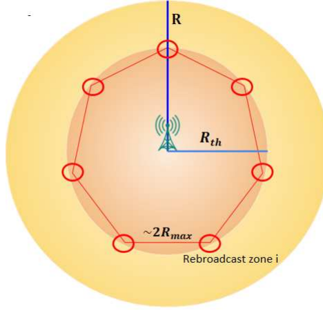
Figure 3.2: Rebroadcast zones
