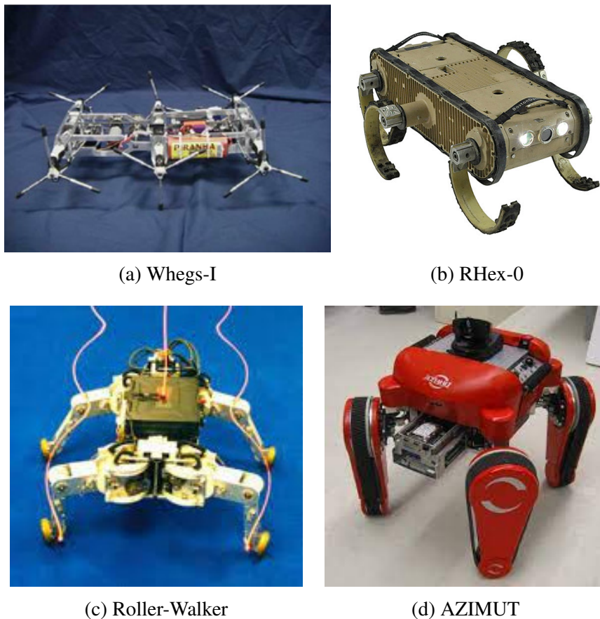
Figure 1.4: Innovative robots combining wheeled and legged locomotion.
