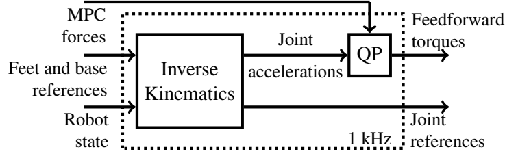
Figure 9.2: Whole-body control scheme with its two successive steps: inverse kinematics and solving of a QP problem
