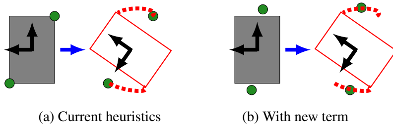
Figure 7.1: Expected feet placement with and without the new heuristics term. Here the robot is just at the beginning of the stance phase for the front right and hind left feet, with \dot{q}_{lin} = [0 \ 0 \ 0]^T and \dot{q}_{ang} = [0 \ 0 \ \dot{q}_{ang,z}]^T . The red rectangles represent the expected orientation of the body at the end of the stance phase. By shifting the feet with the new term in (b), shoulders would be more centered on the contacts on average, compared to what is obtained with the current heuristic (a).
