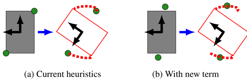
Figure 7.1: Expected feet placement with and without the new heuristics term. Here the robot is just at the beginning of the stance phase for the front right and hind left feet, with \dot{q}_{lin} = [0 \ 0 \ 0]^T and \dot{q}_{ang} = [0 \ 0 \ \dot{q}_{ang,z}]^T . The red rectangles represent the expected orientation of the body at the end of the stance phase. By shifting the feet with the new term in (b), shoulders would be more centered on the contacts on average, compared to what is obtained with the current heuristic (a).
