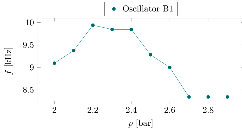
Figure 6.12: Detected frequency of Oscillator B1 for different inlet pressures.
