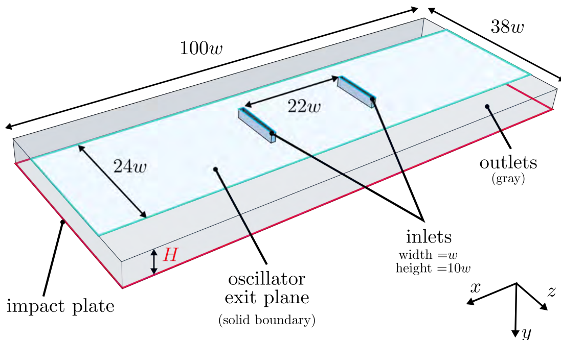
Figure 5.16: Computational domain and boundary conditions
