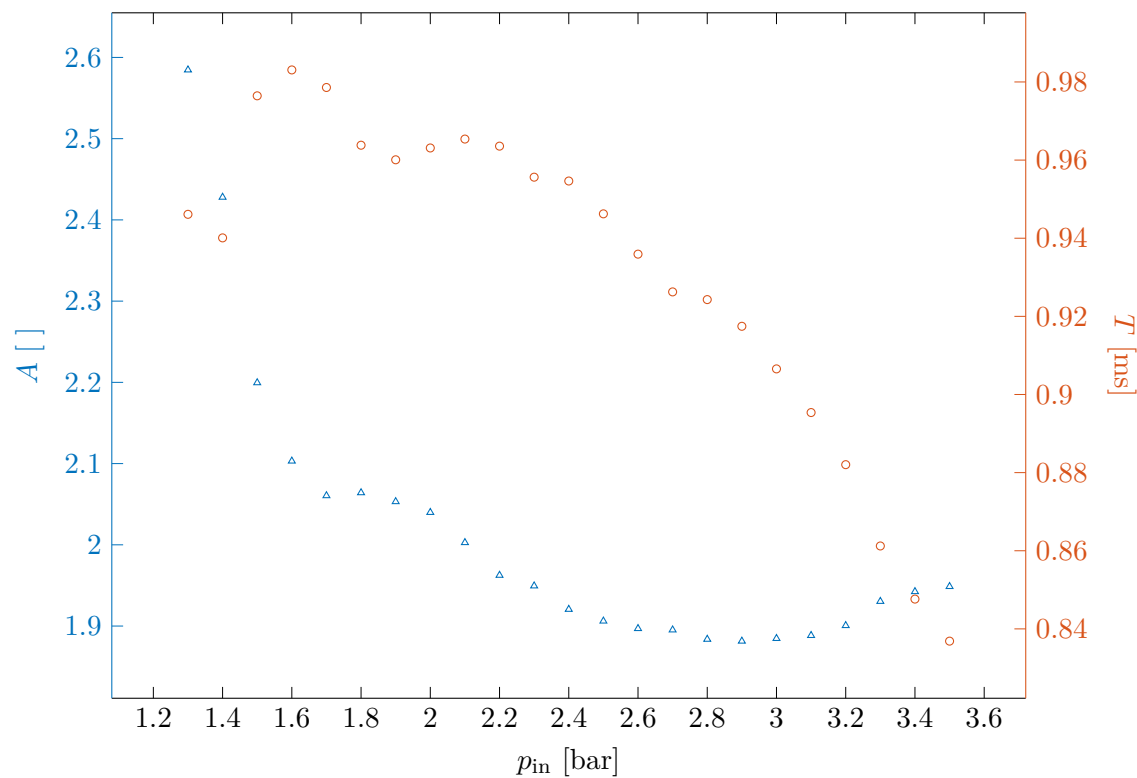
Figure 3.13: Travel length A (triangles) and switching time \tau_{\text{switch}} (circles) versus supply pressure.
