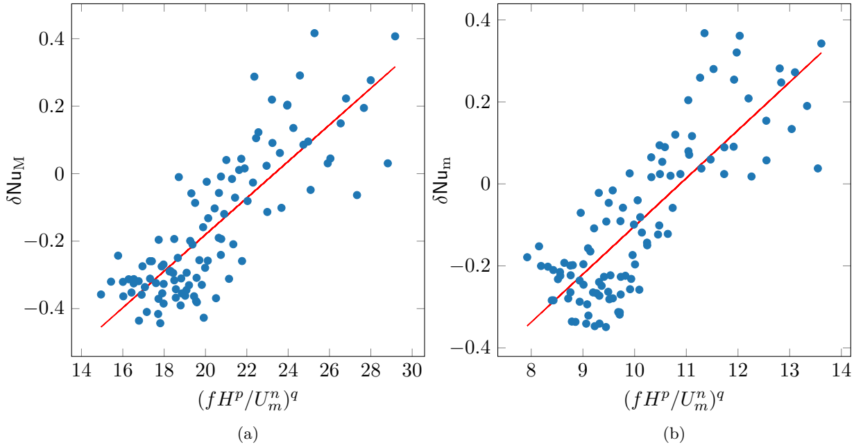
Figure 4.13: Scaling of (a) \delta Nu_M and (b) \delta Nu_m using Eqs. 4.20 and 4.19, respectively.
