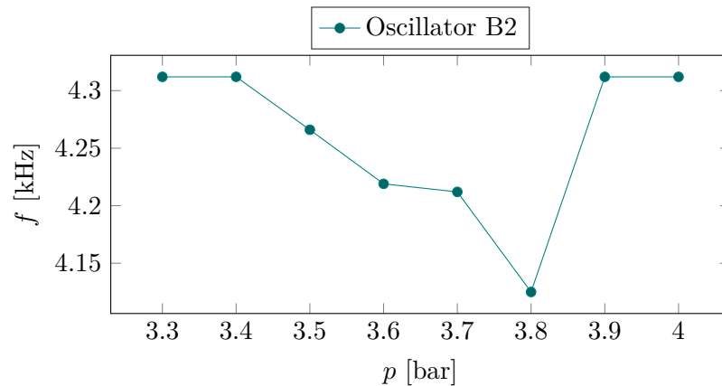
Figure 6.13: Detected frequency of Oscillator B2 for different inlet pressures.
