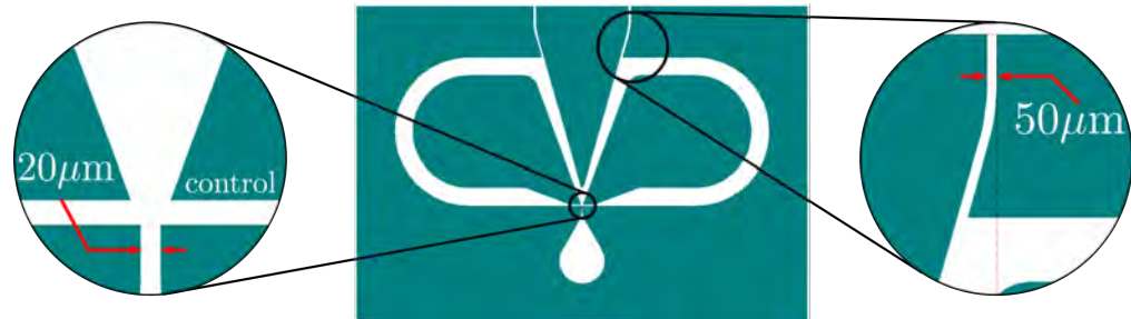
(a) Butterfly (B1): L_f = 11\,000\ \mu\text{m}
