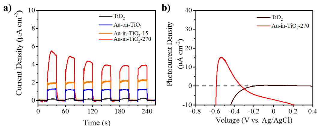
Figure 2.16 (a) On/off photocurrent measurements on \text{TiO}_2 and \text{Au/TiO}_2 hybrid structures. The samples were irradiated under visible light (400-1100 nm): \text{TiO}_2 (black curve), \text{Au-on-TiO}_2 (blue curve), \text{Au-in-TiO}_2-15 (orange curve) and \text{Au-in-TiO}_2-270 (red curve). Off corresponds to the dark current. (b) Photocurrent-potential curves in 0.05 M \text{Na}_2\text{SO}_4 solution for \text{TiO}_2 (black curve) and \text{Au-in-TiO}_2 (red curve) obtained under dark and UV+Vis light (353-1100 nm).
