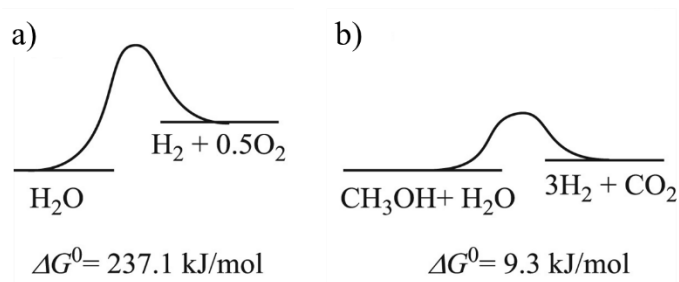
Figure 1.12 Energy diagrams for (a) water splitting (up-hill), and (b) water splitting with scavenger agent (small up-hill) processes. Retrieved from 121 .
