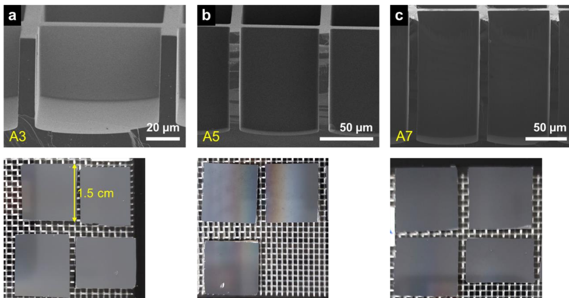
Figure 3.12 Silicon 3D scaffolds featuring different (a) AEF 3, (b) 5, and (c) 7, with a Depth of 50, 100 and 150 \mu\text{m} , respectively. Top: SEM cross-sectional images of the microcavities, bottom: photographs of the cut scaffolds.
