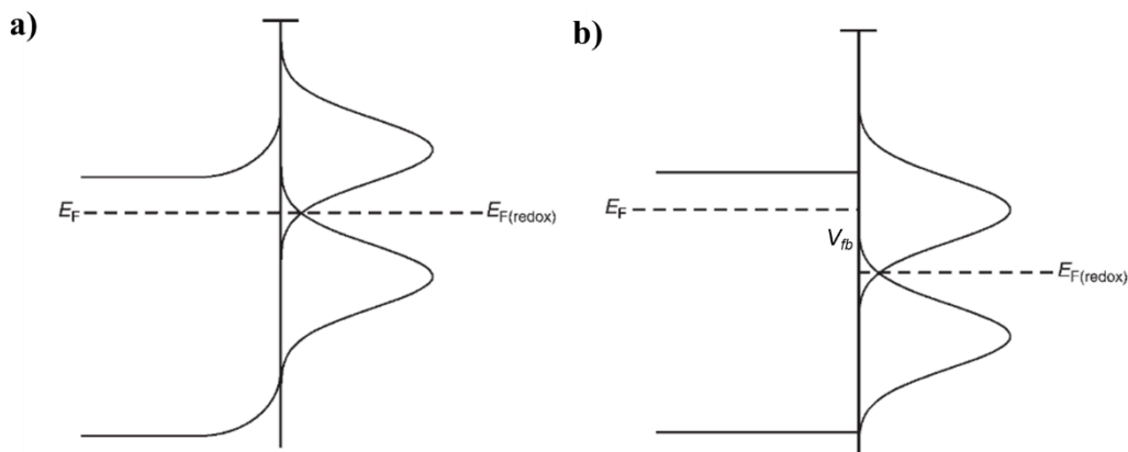
Figure 2.7 Scheme of an n-type semiconductor showing the fermi level ( E_F ) and the redox states of the electrolyte with its corresponding fermi level ( E_{F(redox)} ) (a) at the electronic equilibrium and (b) situation when the semiconductor is at its flat-band potential V_{fb} .
