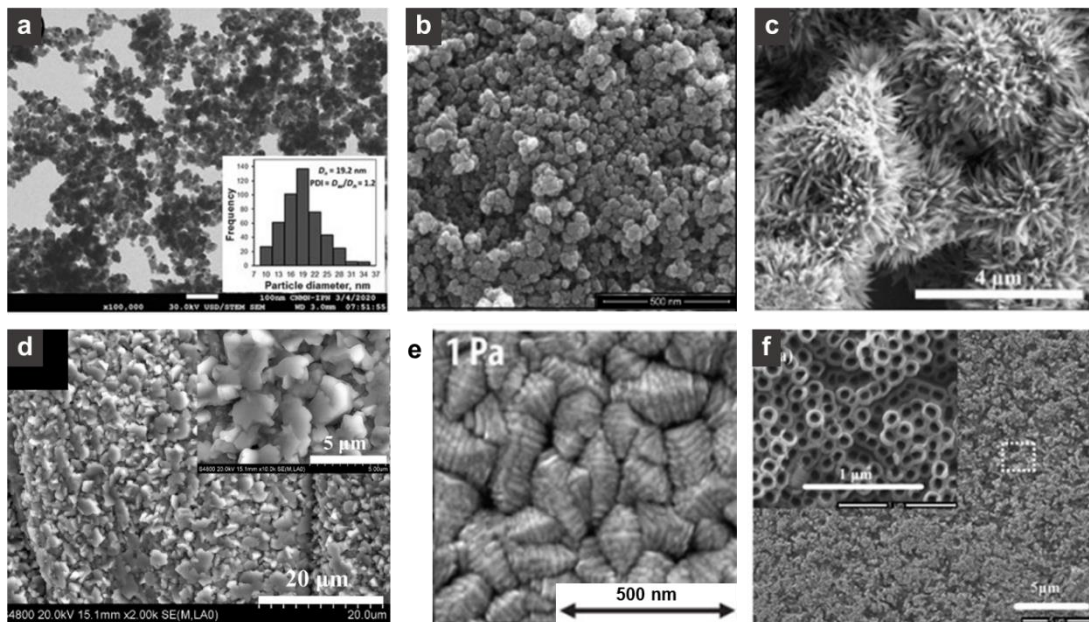
Figure 1.10 SEM images of TiO 2 nanostructures fabricated through (a) precipitation, 114 (b) sol-gel hydrolysis, 115 (c) solvothermal synthesis, 116 (d) CVD, 117 (e) sputtering 118 and (f) electrolytic anodization. 119
